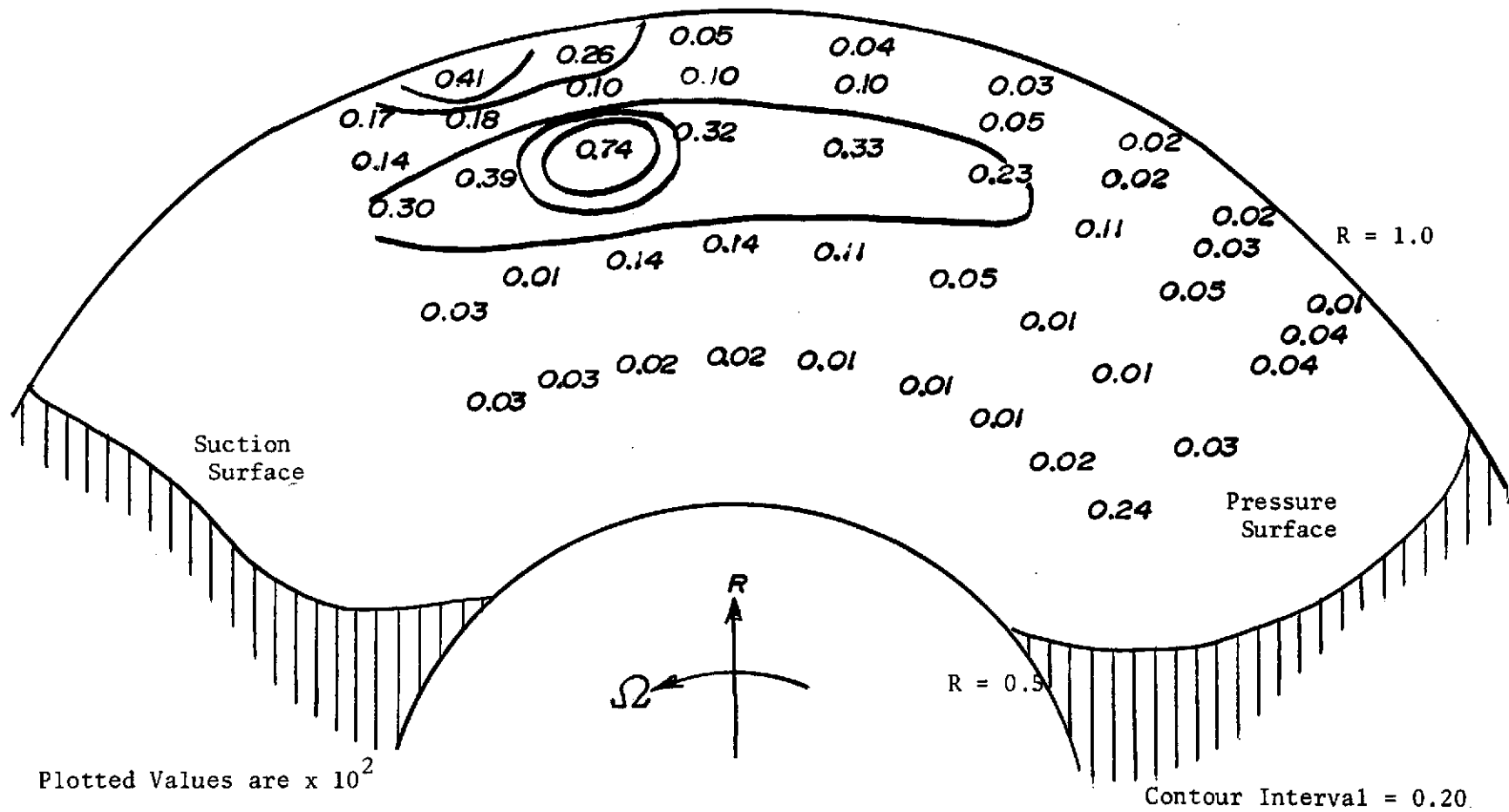
Figure 39. Turbulence Velocity Correlation (\overline{uw}/Q_R^2) at Station 2
