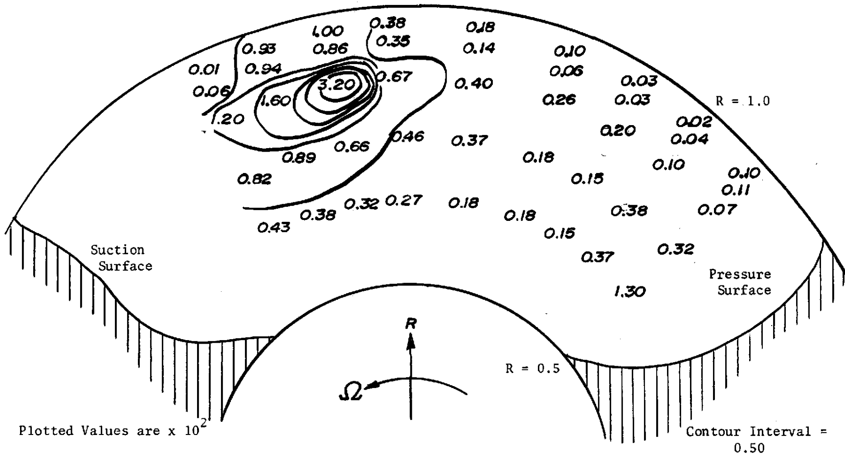
Figure 38. Turbulence Velocity Correlation (\overline{uv}/Q_R^2) at Station 2
