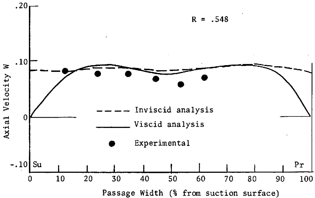
Figure 48. Comparison of Axial Velocity Distributions at Station 1, R = .973 and R = .548
