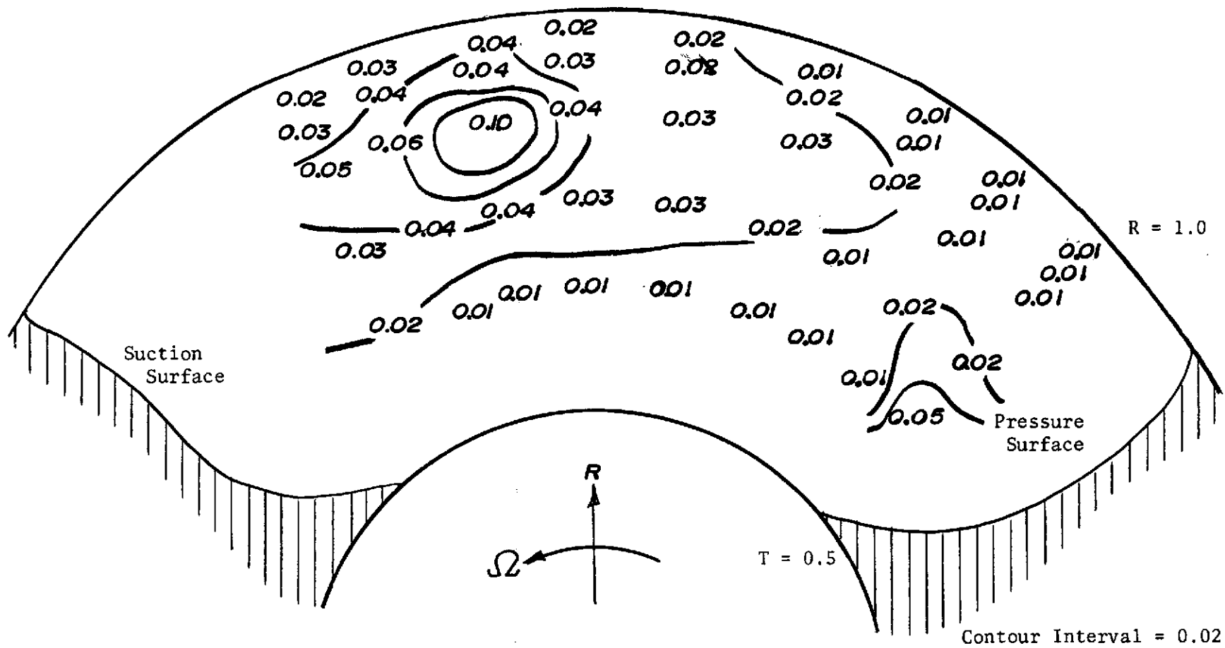
Figure 37. Total Turbulence Energy ( \overline{q^2}/Q_R^2 ) at Station 2
