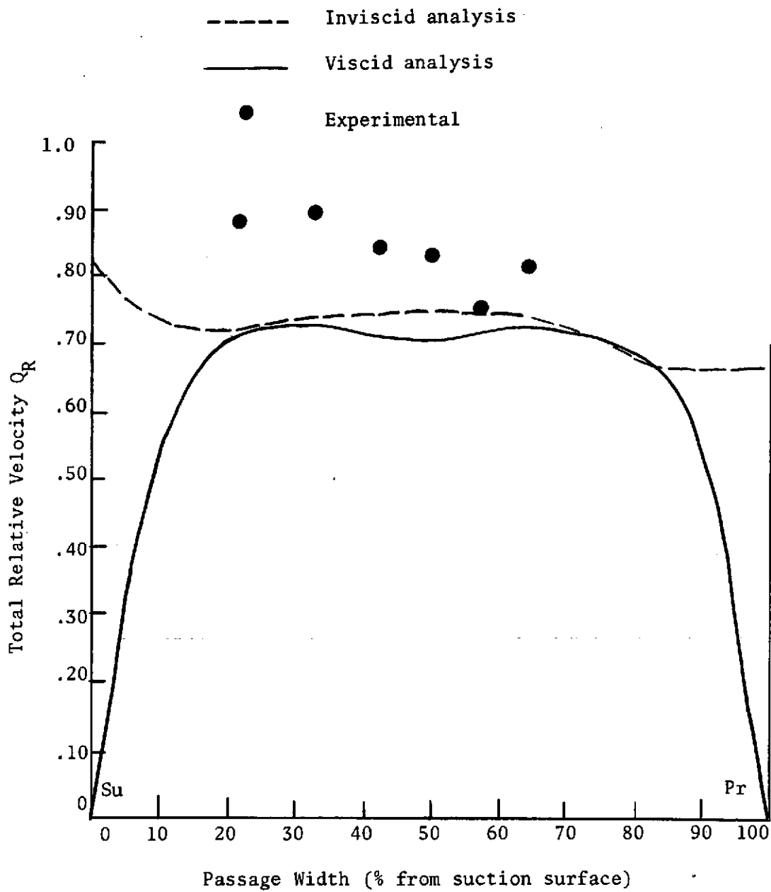
Figure 46. Comparison of Total Relative Velocity Distributions at Station 1; R = .973
