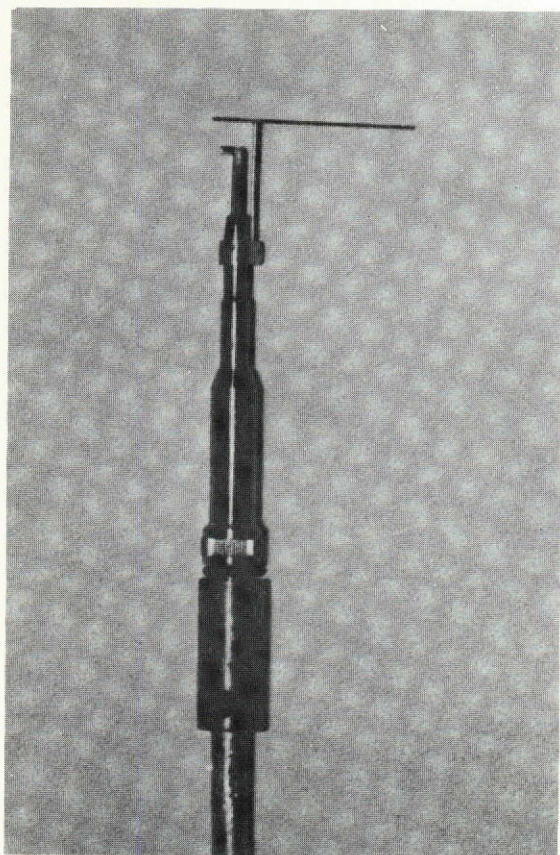
Figure 10a. Triaxial Hotwire Probe and Support
