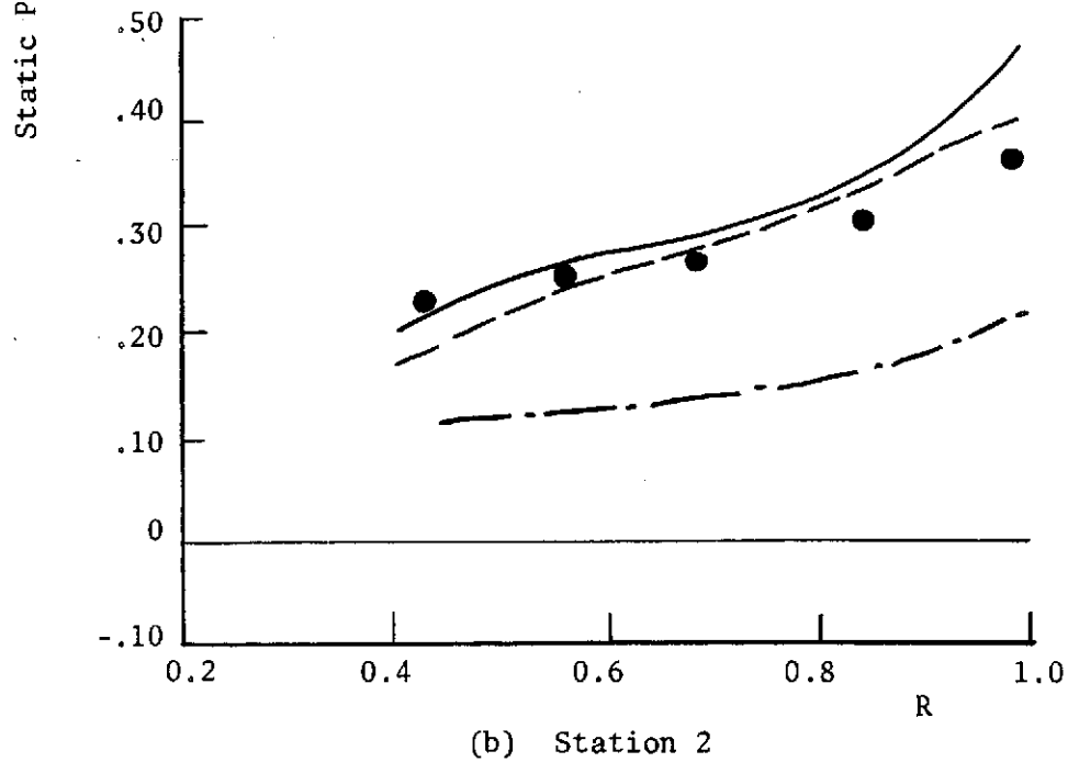
Figure 17. Radial Variation of Passage-Averaged Static Pressure Coefficient at Stations 1 and 2
