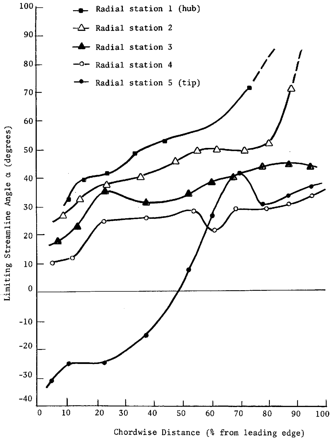
Figure 18. Chordwise Variation of Limiting Streamline Angle on Blade Pressure Surface
