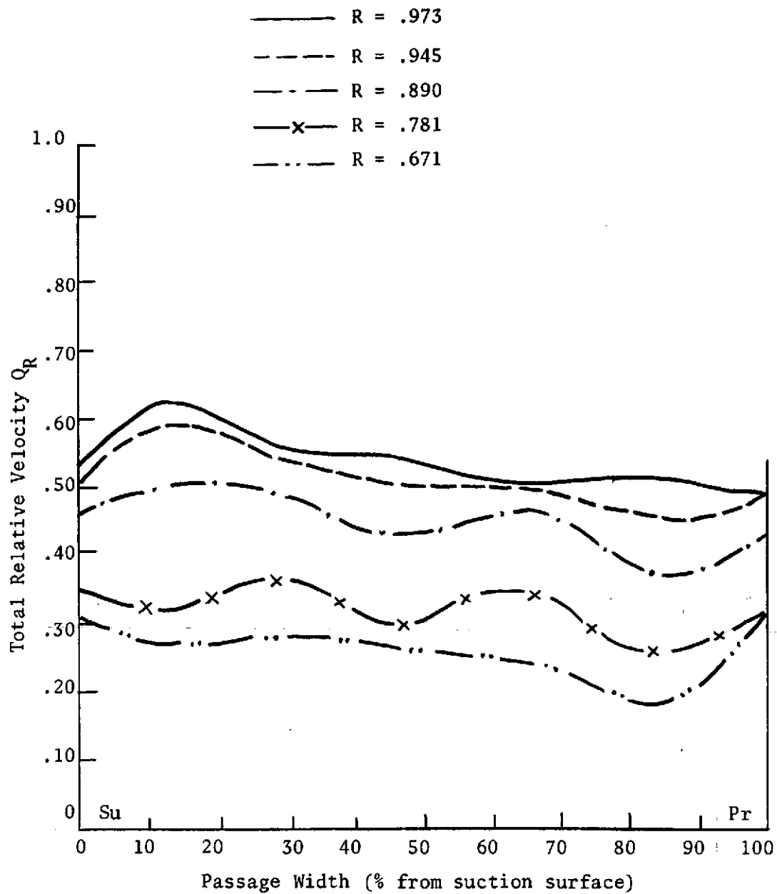
Figure 49. Inviscid Analysis Results for Total Relative Velocity Distribution at Station 2
