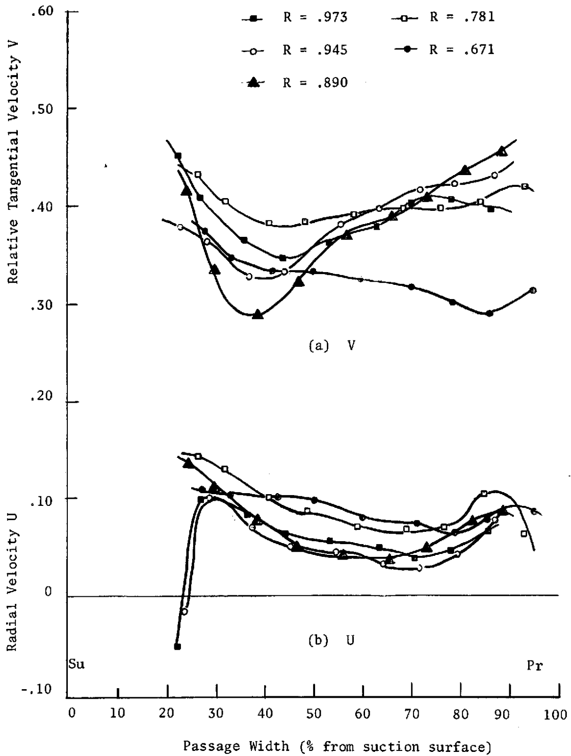
Figure 32. Relative Tangential Velocity and Radial Velocity Distributions at Station 2
