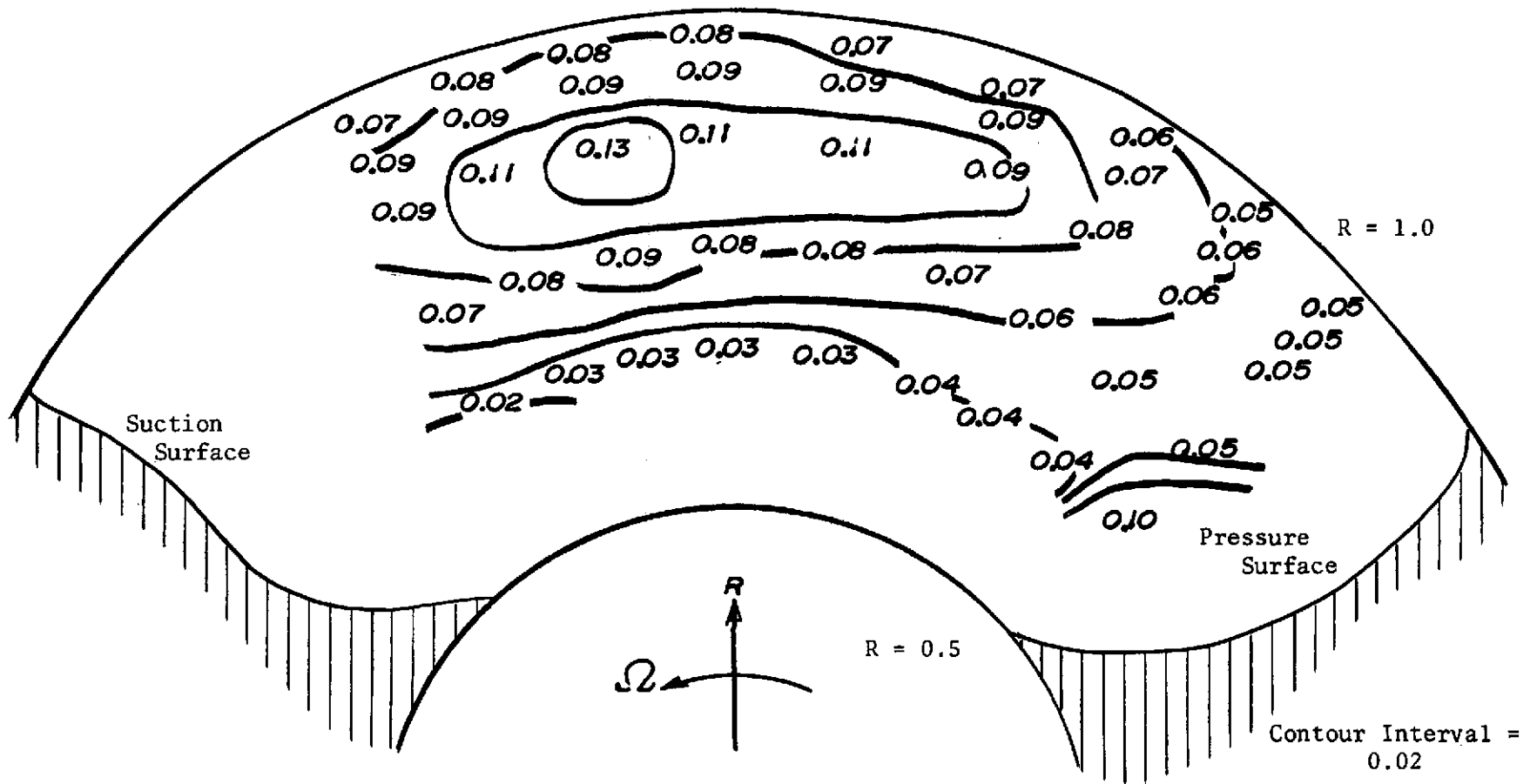
Figure 35. Axial Turbulence Intensity ( \sqrt{w^2}/Q_R ) at Station 2
