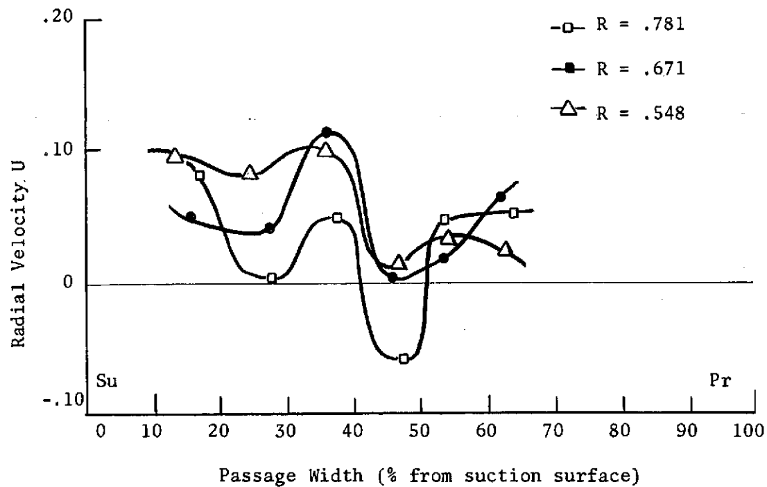
Figure 28. Radial Velocity Distribution at Station 1
