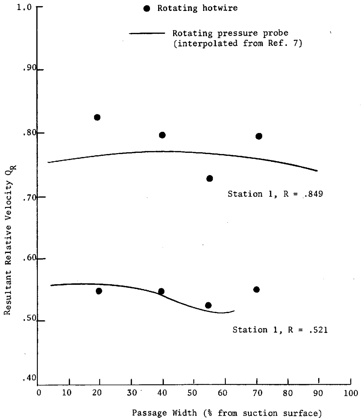
Figure 21. Comparison of Rotating Hotwire and Rotating Pressure Probe Measurements.
