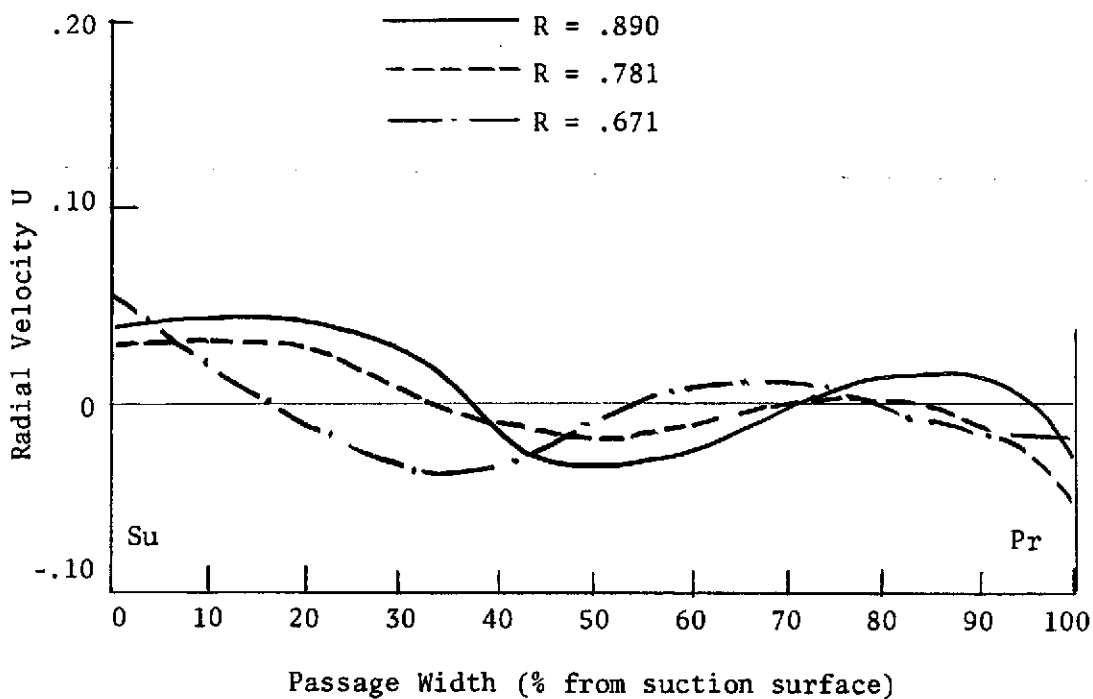
Figure 56. Inviscid Analysis Results for Radial Velocity Distribution at Station 2
