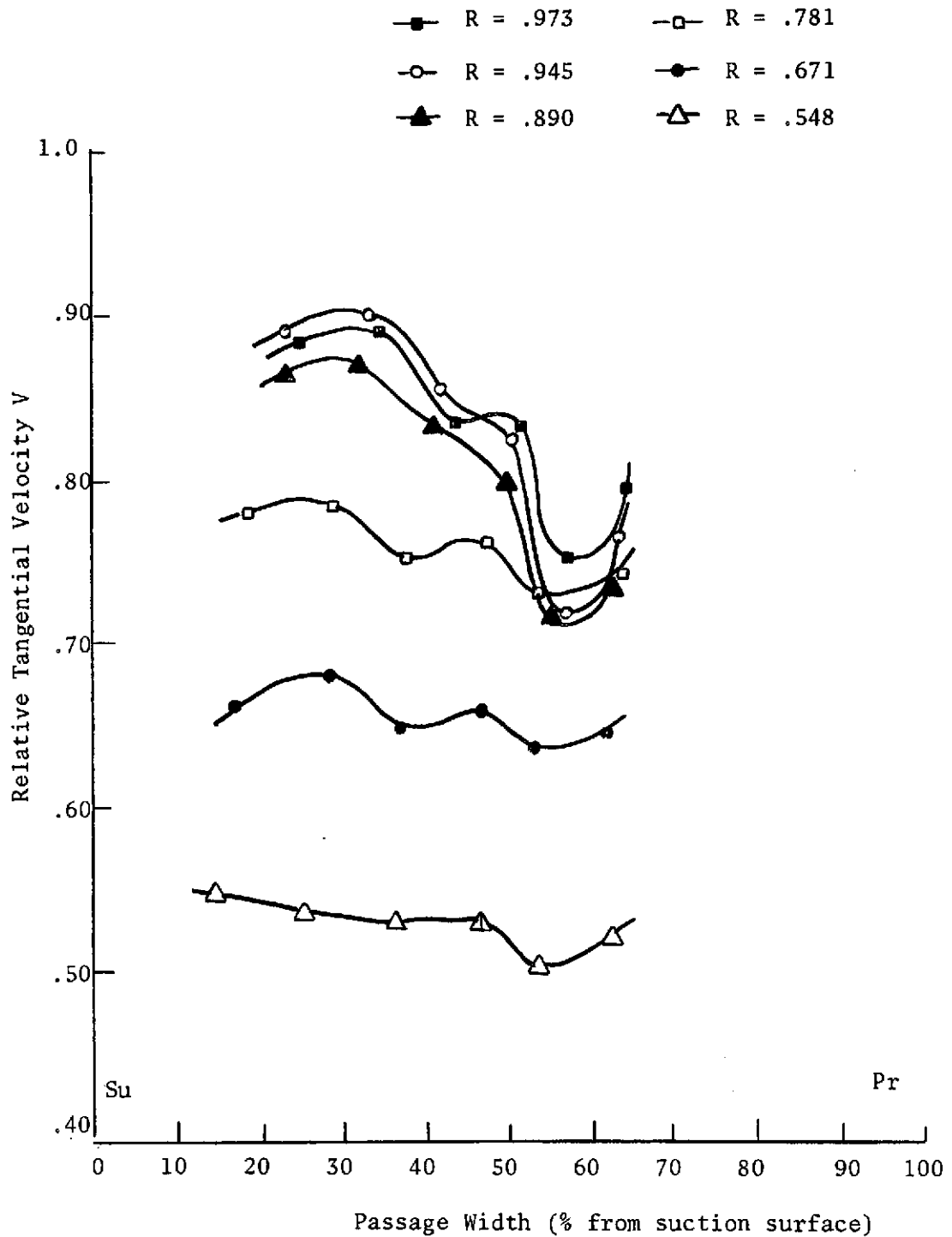
Figure 24. Relative Tangential Velocity Distribution at Station 1
