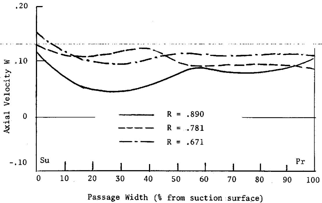
Figure 53. Inviscid Analysis Results for Axial Velocity Distribution at Station 2.
