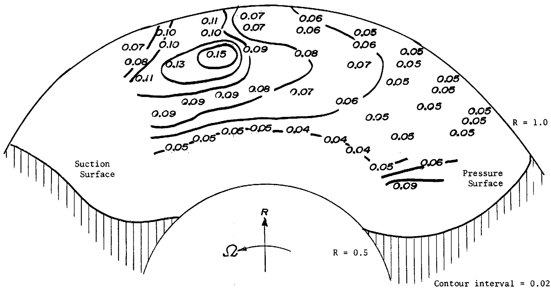
Figure 34. Tangential Turbulence Intensity ( \sqrt{v^2}/Q_R ) at Station 2
