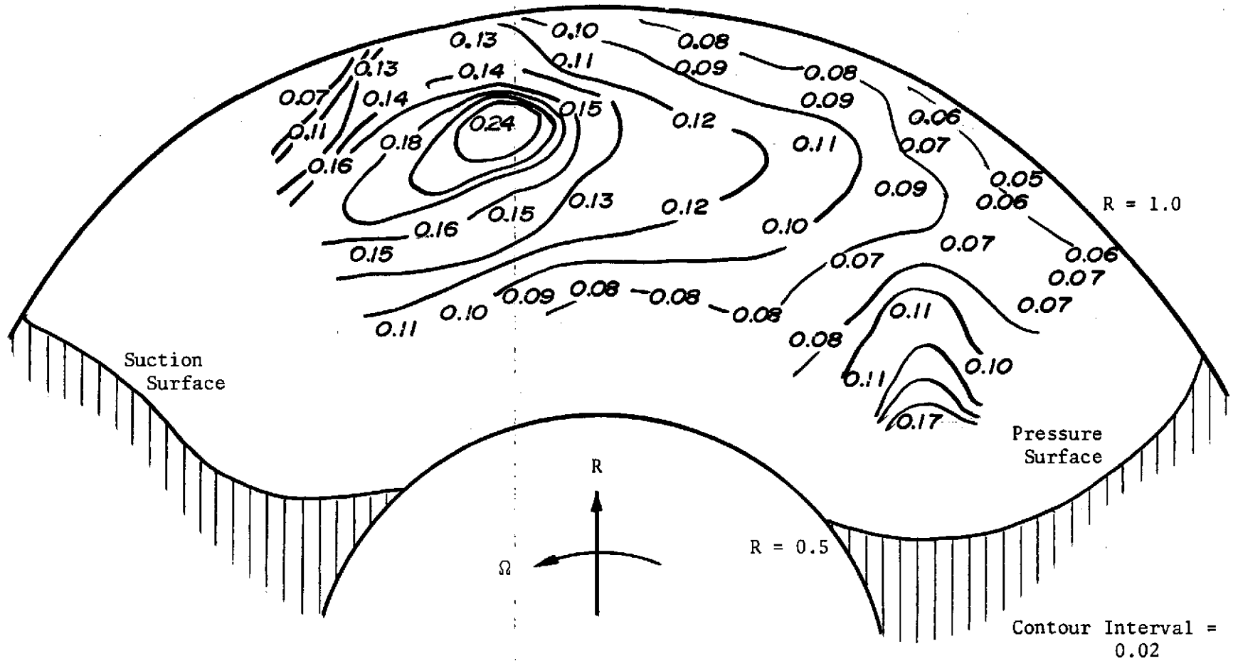
Figure 36. Radial Turbulence Intensity ( \sqrt{u^2}/Q_R ) at Station 2
