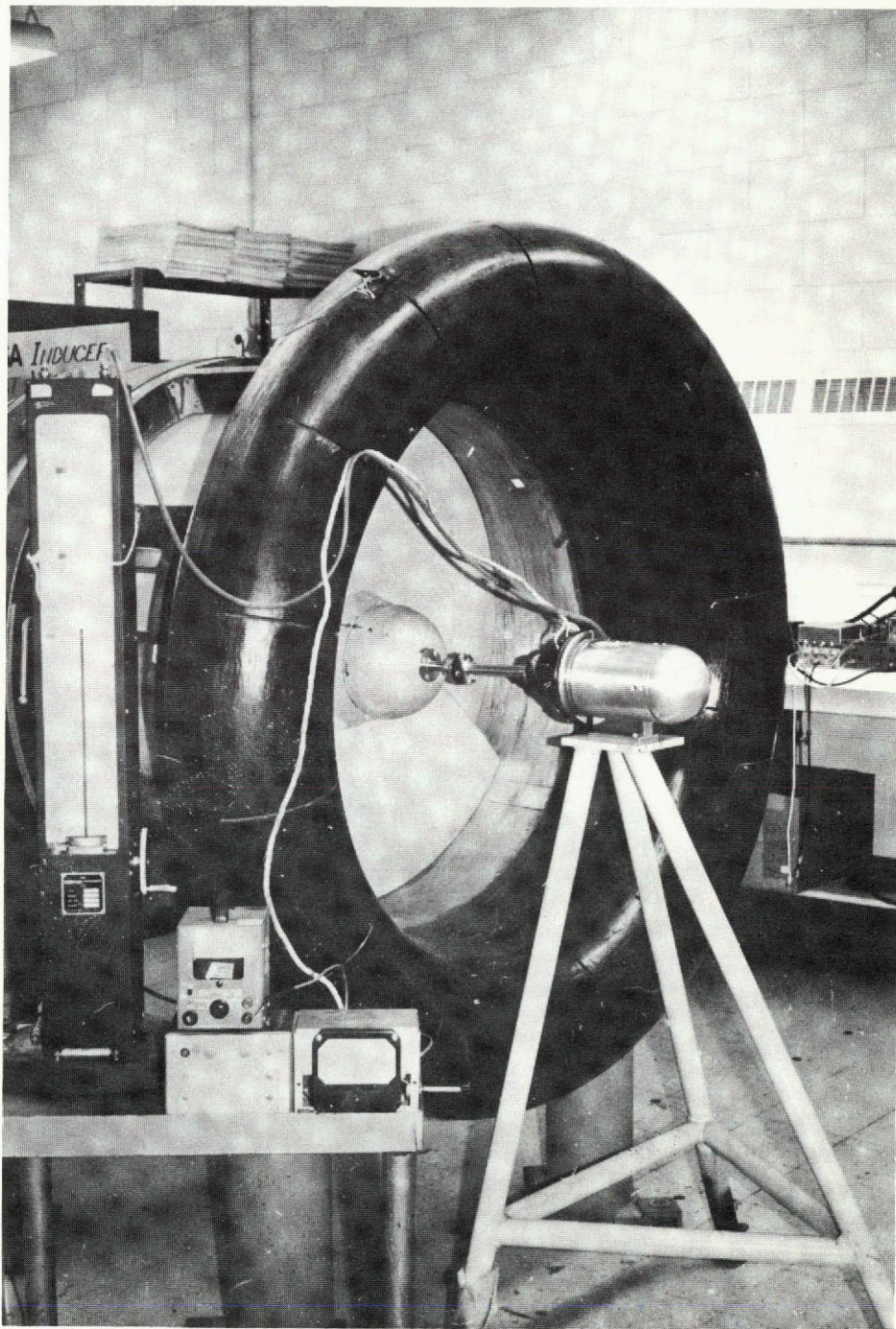
Figure 7. Blade Static Pressure Test Setup
