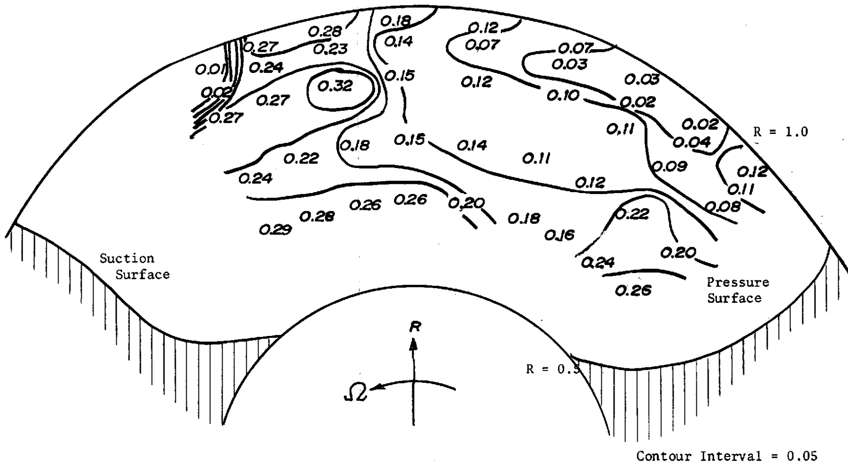
Figure 41. Turbulence Ratio ( \overline{uv}/q^2 ) at Station 2
