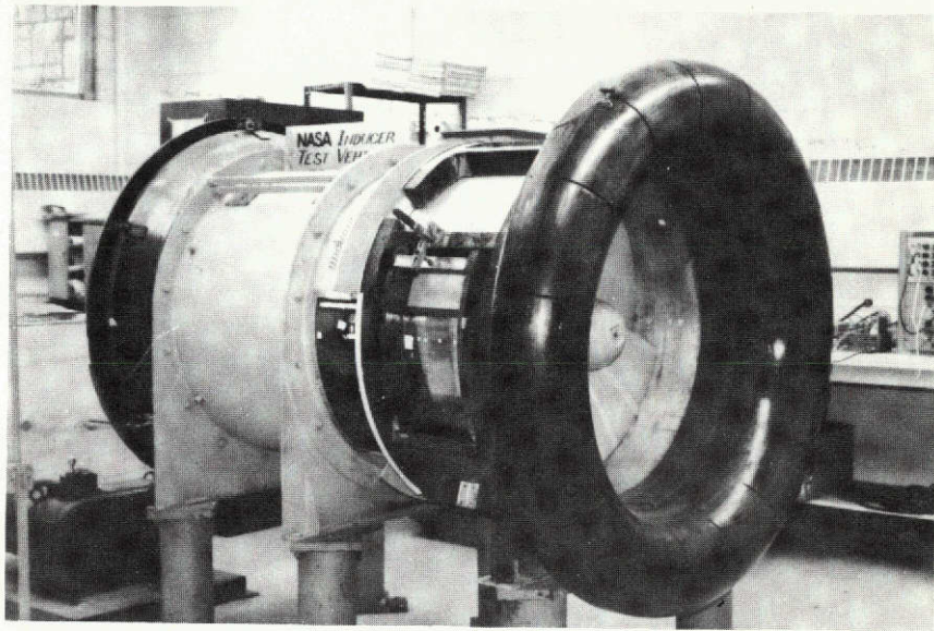
Figure 1a. Inducer Test Facility
