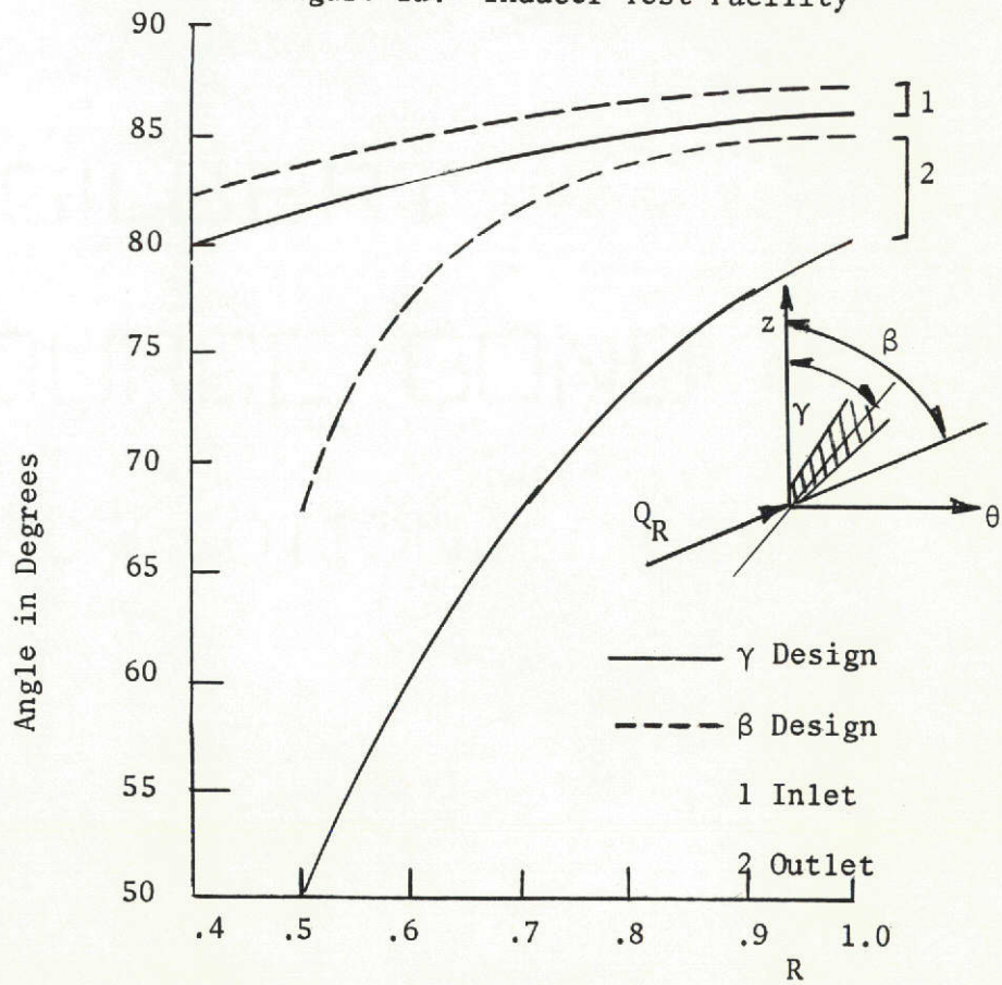
Figure 1b. Inducer Inlet and Outlet Angle
