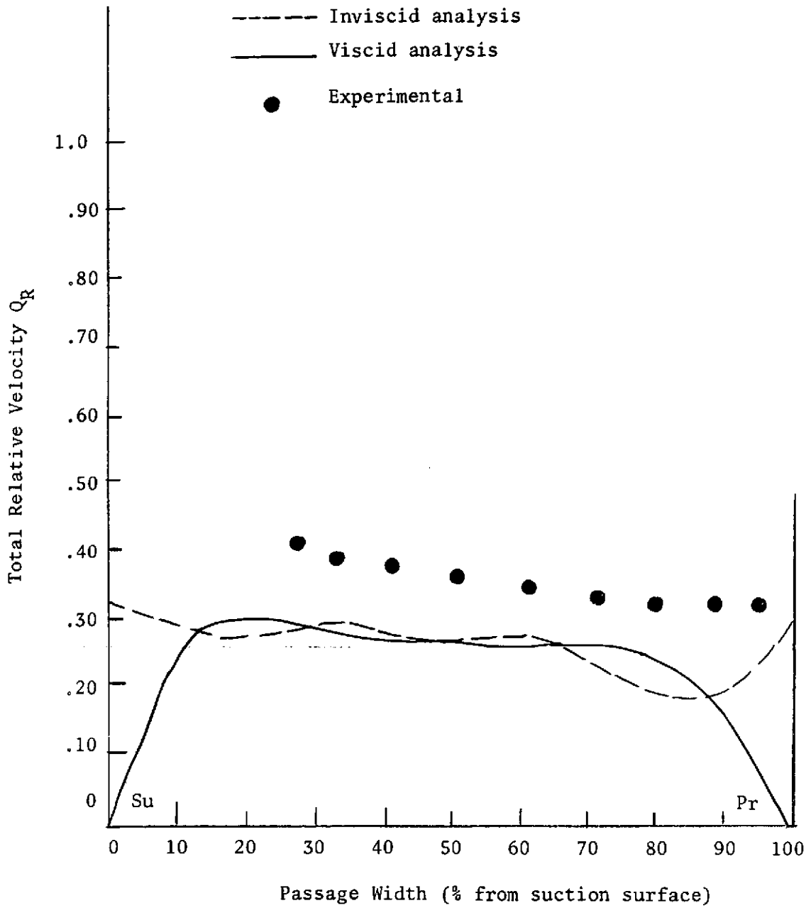
Figure 52. Comparison of Total Relative Velocity Distributions at Station 2, R = .671
