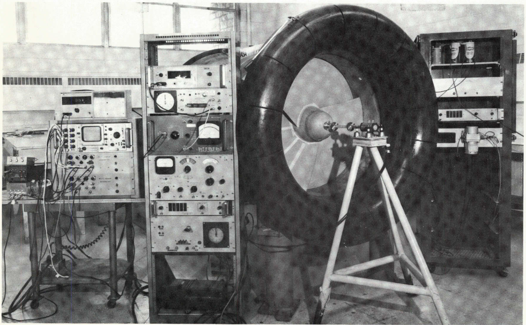
Figure 11. Rotating Hotwire Test Setup
