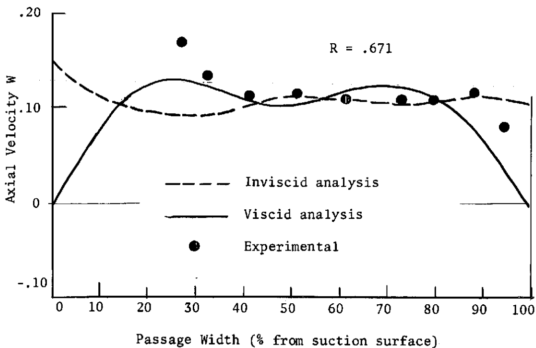
Figure 55. Comparison of Axial Velocity Distributions at Station 2, R = .973 and R = .671
