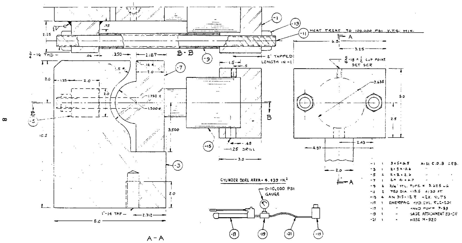
Figure 3-1. Test Fixture for Press Tonnage Determination
