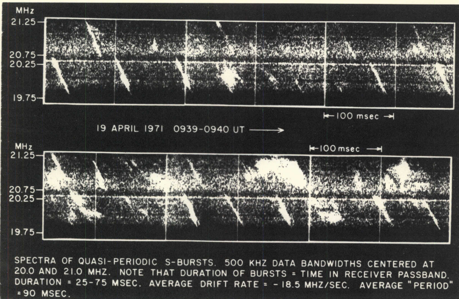
Figure 2 -- Spectra of two 500-kHz-bandwidth channels as recorded in Huanta, Chile in 1971.
