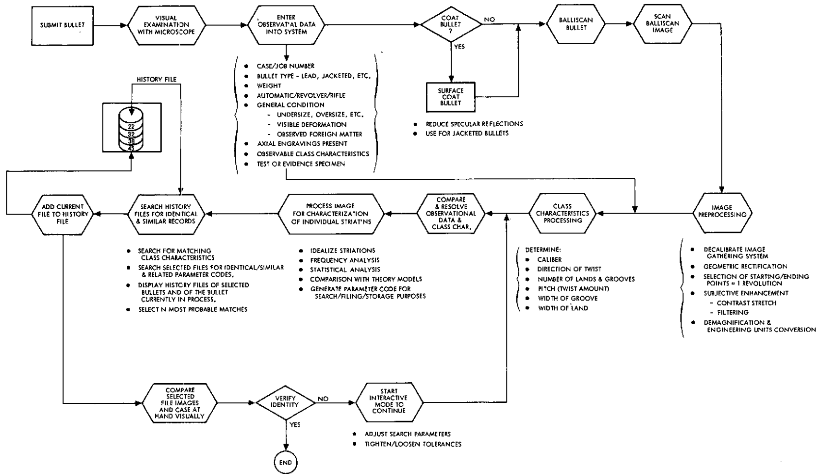
Figure 11. Schematic diagram of image processing system for bullet data
