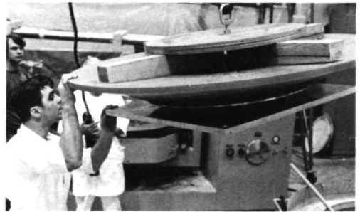
D. Loading mirror with mount onto polishing machine. Center and edge thicknesses of mirror can be seen.
