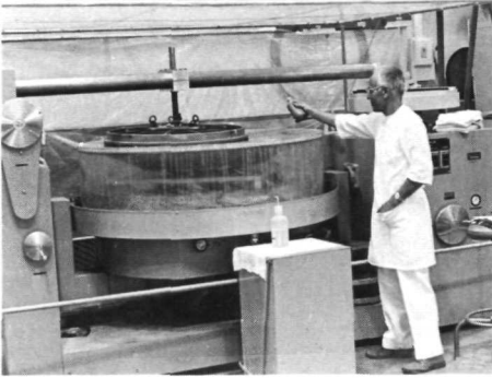
E. Polishing the primary.
