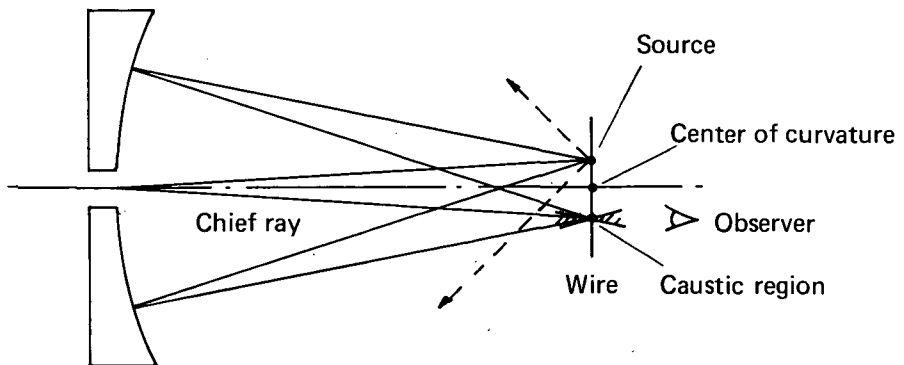
Schematic of axial wire test.
