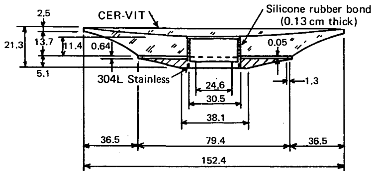
AFCRL 152-cm f/2.5 mirror. Design credit: W. E. Carter.
