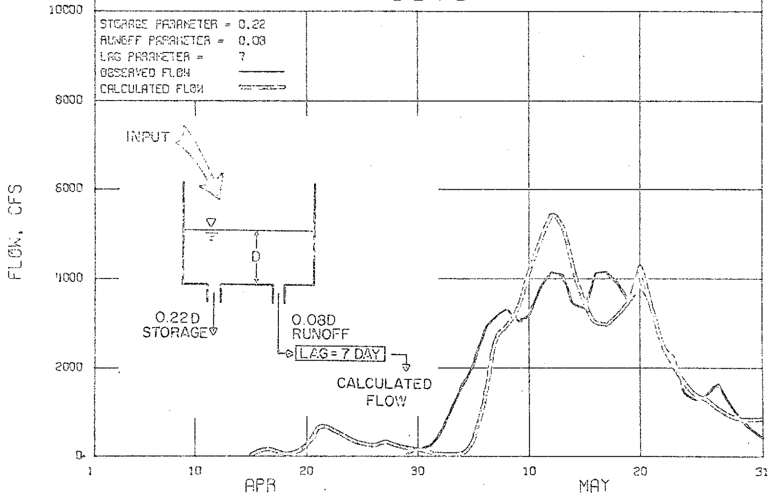
Fig. 13. Snowmelt Runoff vs. Time from Computer Snowmelt Model and Direct Measurements
