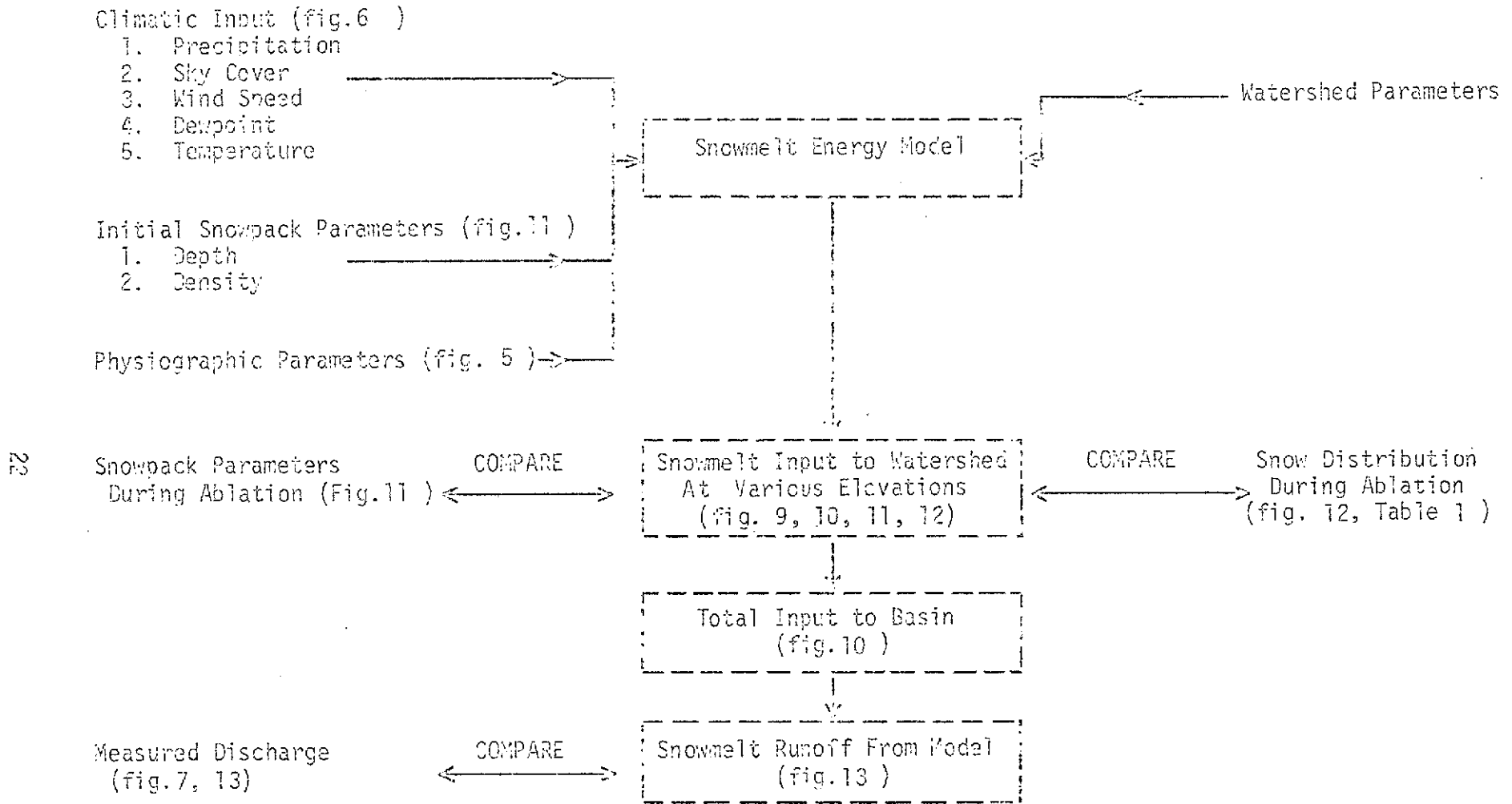
Fig. 14. Diagram Illustrating the Relationship Between the Ground Truth, Computer Snowmelt Model, and ERTS-1 Imagery.
