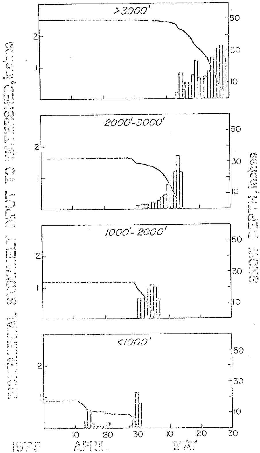
Fig. 2. Daily Incremental Snowmelt Input to Watershed From Snowmelt Model at Different Elevation Ranges
