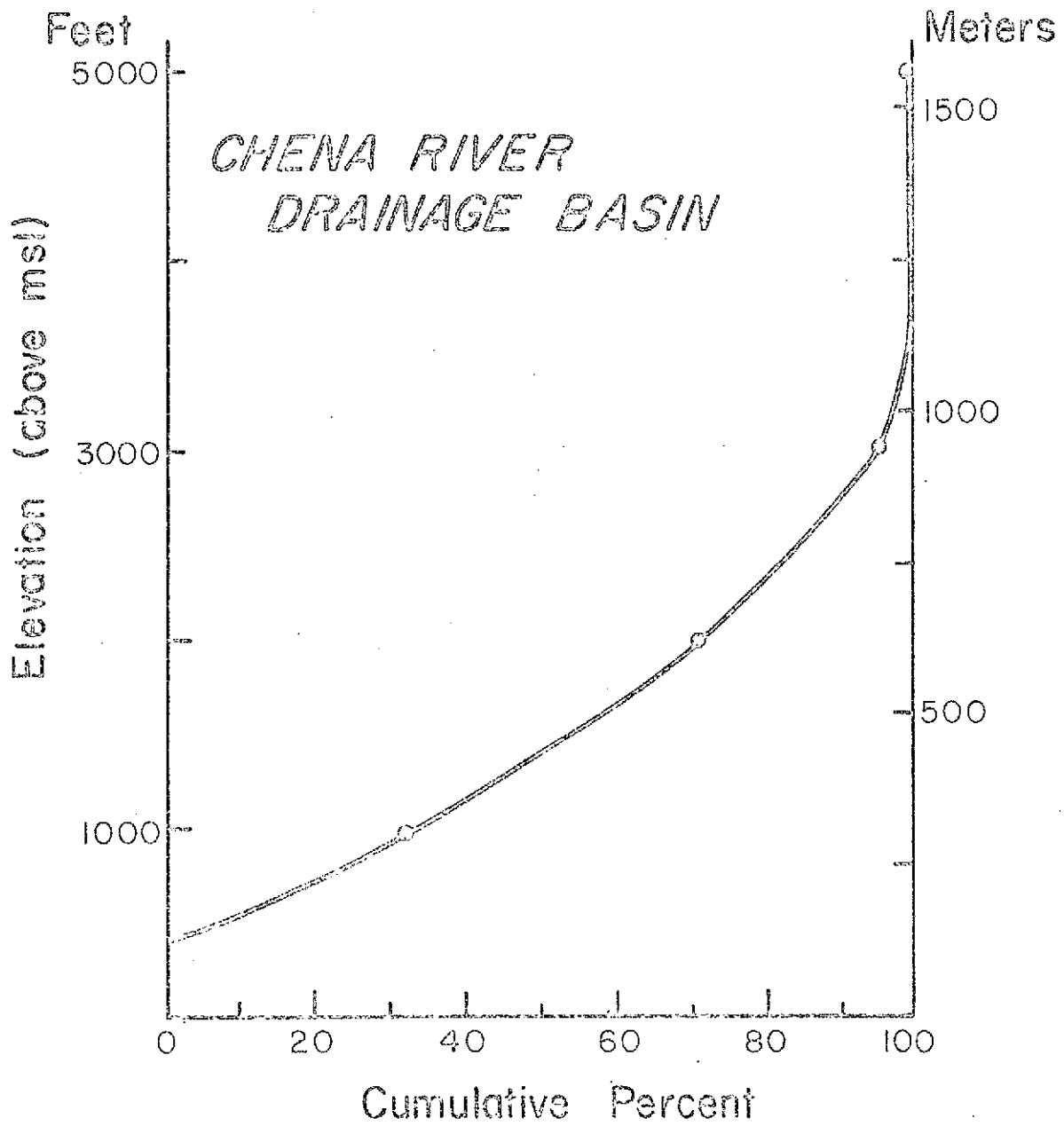
Fig. 5. Percent Area-Elevation Curve for Chena River Basin
