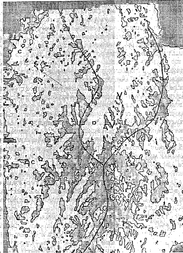
Figure 3. Printout of microdensitometer scan of the original of which Figure 1 was derived. Clouds and their shadows (C), Big Creek valley (V), and small valleys (D) appear. The main dark area is spruce forest. The highest ridges are shown as a heavy line.
