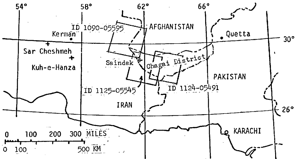
Figure 1.--Index map of the Saindak area, showing ERTS-1 image coverage.
