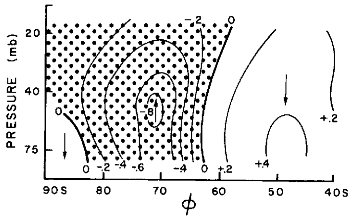
Fig. 5.10 Zonally-averaged vertical motion patterns for the S. H. for July 1969. Units: \text{mb day}^{-1} .
