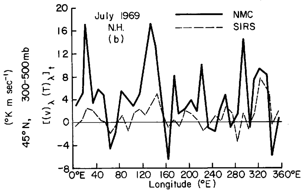
Fig. 4.12 Longitudinal distribution of total eddy heat flux for the layer 300-500 mb, at 45^{\circ}\text{N} in January 1970 and July 1969.
