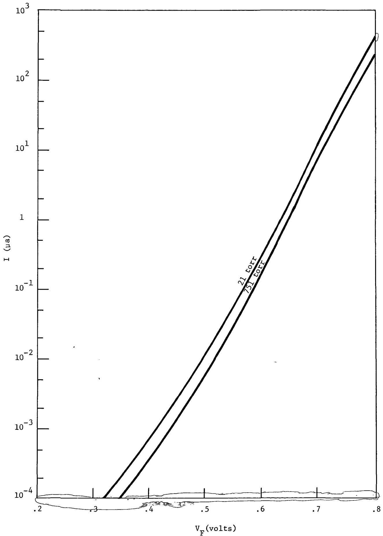
Figure 47. Log Current-Voltage Characteristics of Transducer 10-B50
