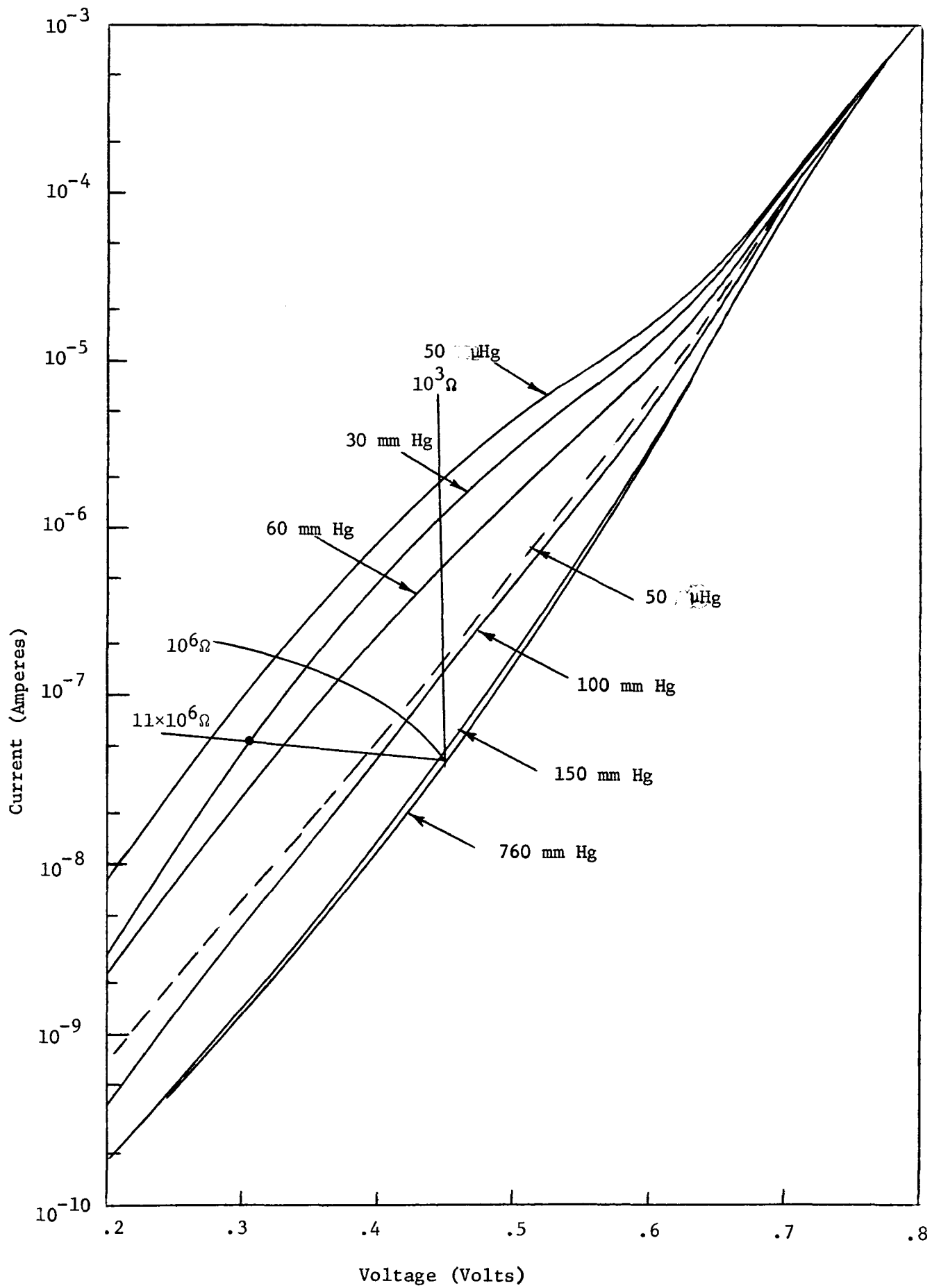
Figure 28. Log I-V Characteristics of Transducer No. 1; Bias Condition 4
