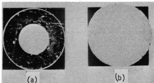
Fig. 2. Bottom view of electrostatically sealed piezoresistive pressure transducers. (a) Borosilicate glass cavity, (b) Silicon cavity.
