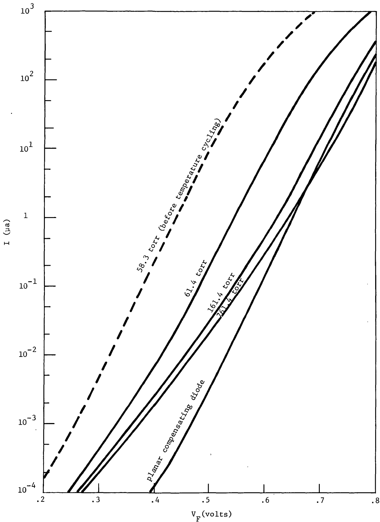
Figure 45. Log Current-Voltage Characteristics of Transducer 877
