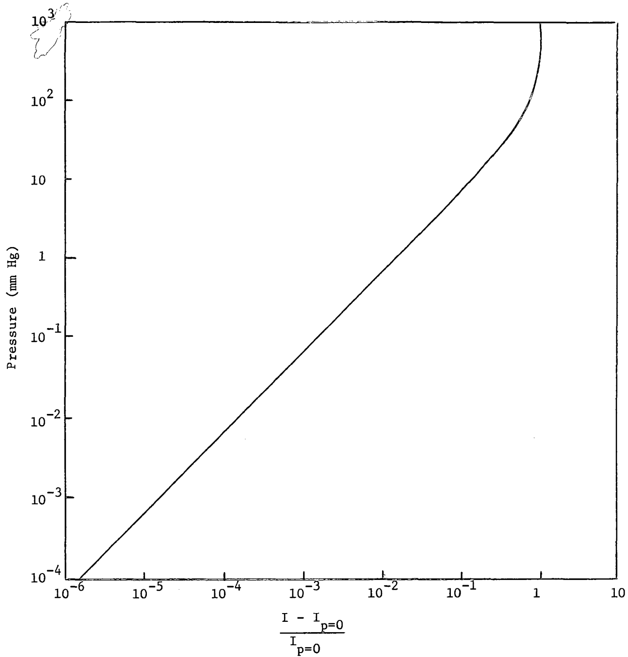
Fig. 11. Relative Change in Current Per Unit Pressure.
