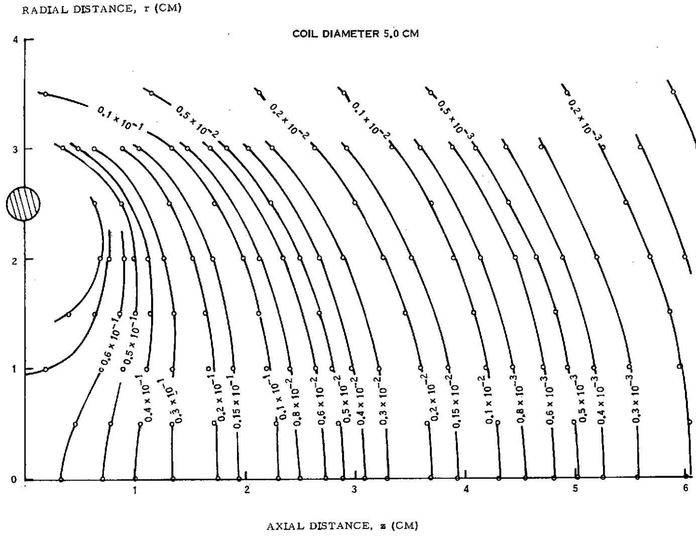
Figure 5-4. \left(\frac{B}{NI}\right)^2 for Circular Coil (Contours are labeled in \text{gauss}^2/\text{amp}^2 )
