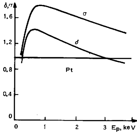
Figure 4-8. True and Total Electron Emission Coefficients as a Function of Energy for Platinum
