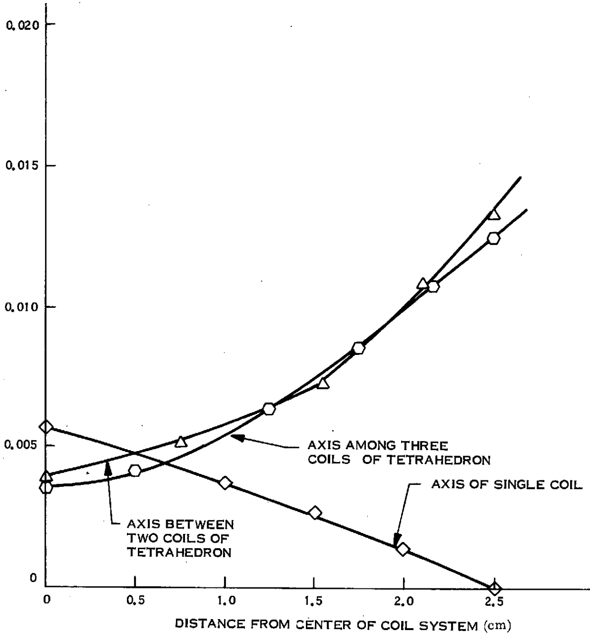
Figure 5-12. Calculated Force Along Axes of Symmetry for Tetrahedron with Coils of Radius 5.0 cm, a Distance 2.5 cm from the Center of the Coil System
