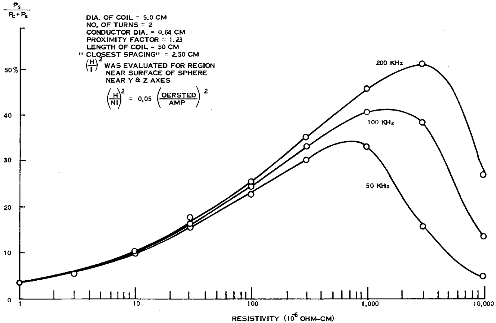
Figure 5-29. Efficiency of Heating a Specimen vs. Resistivity for a Baseball Coil
