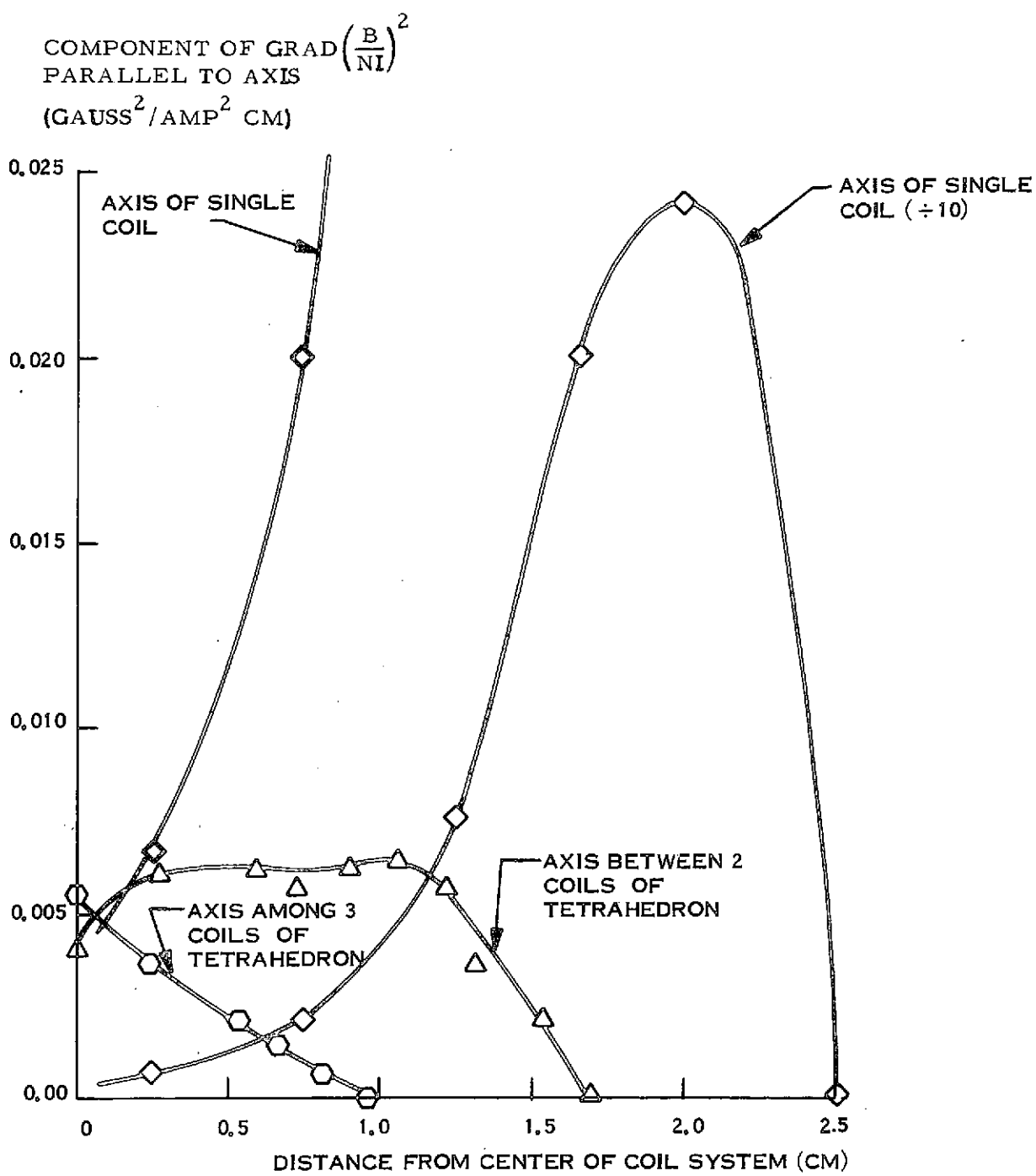
Figure 5-11. Calculated Force Along Axes of Symmetry for Tetrahedron with Coils of Radius 2.5 cm, a Distance 2.5 cm from the Center of the Coil System
