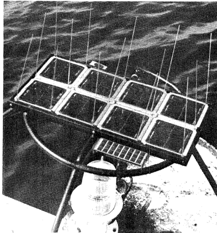
Figure 15. - A 1-watt FEP-encapsulated solar cell module mounted on a Coast Guard Navigation Buoy, Boston Harbor, Massachusetts.
