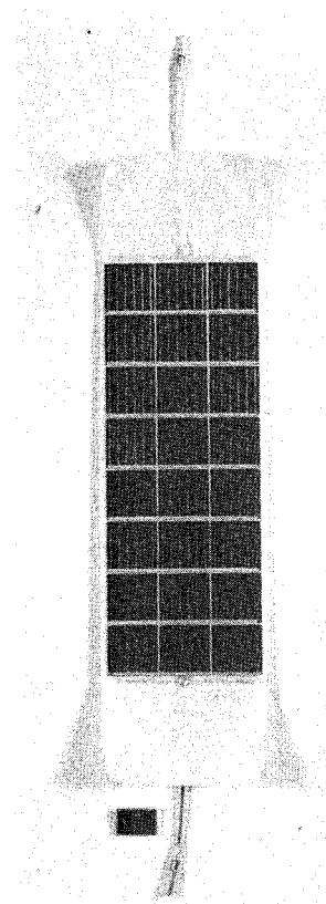
Figure 2. - A 1-watt fiber-glass cloth substrate FEP-encapsulated module.
