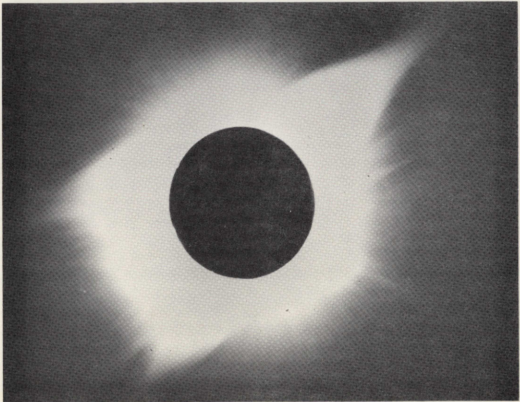
Fig. 2 Eclipse, 25 February 1952
