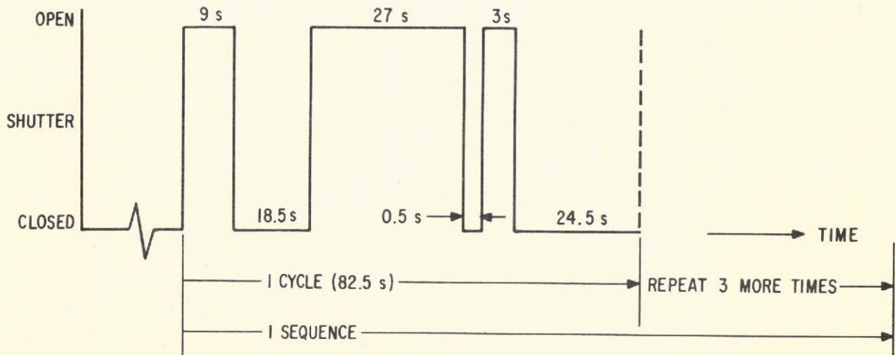
Fig. 3 Eclipse, 7 March 1970
