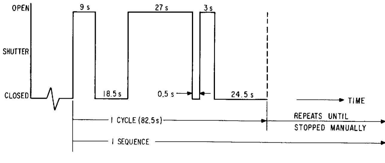
Fig. 5 Operational mode sequence, extended standard patrol
