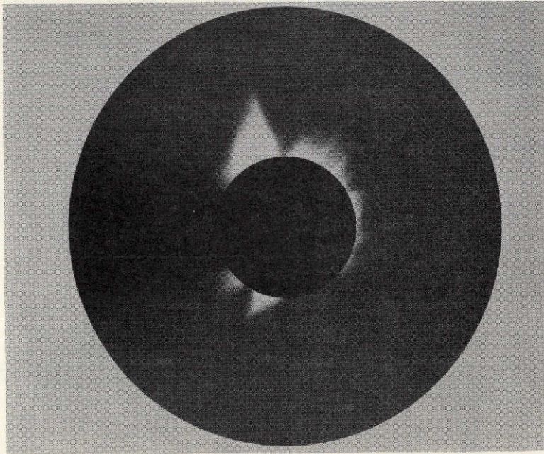
Fig. 12 Simulated TV photograph of 7 March 1970 eclipse
