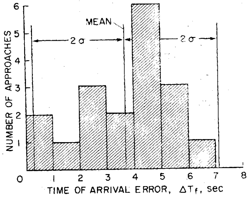
Figure 11.- Time-of-arrival error at waypoint 13.
