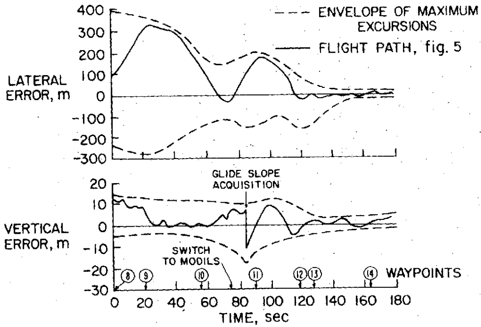
Figure 7.- Guidance errors.
