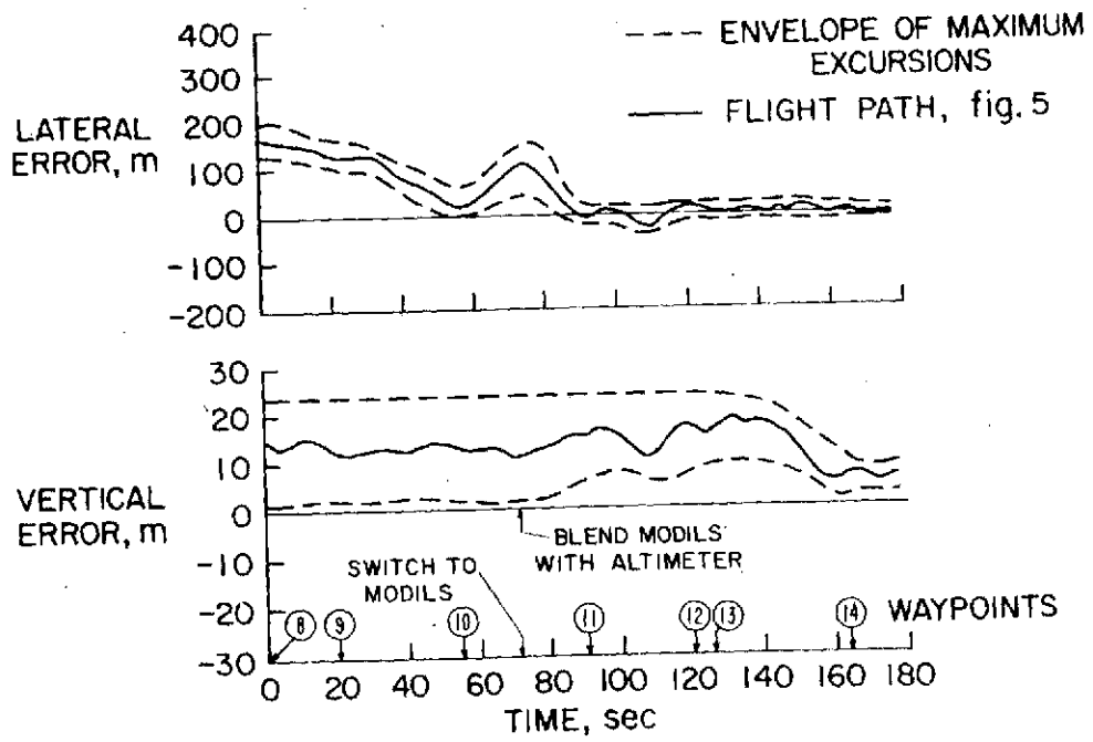
Figure 6.- Navigation errors.
