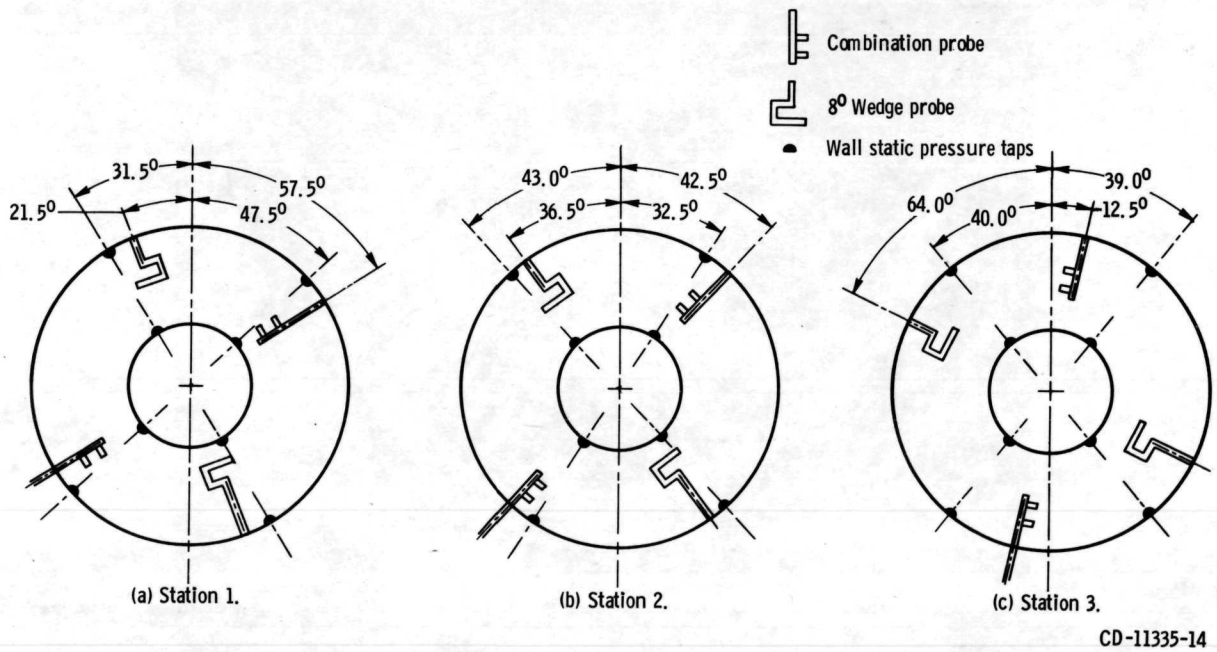
Figure 6. - Circumferential location of instrumentation at measuring stations (facing downstream).
