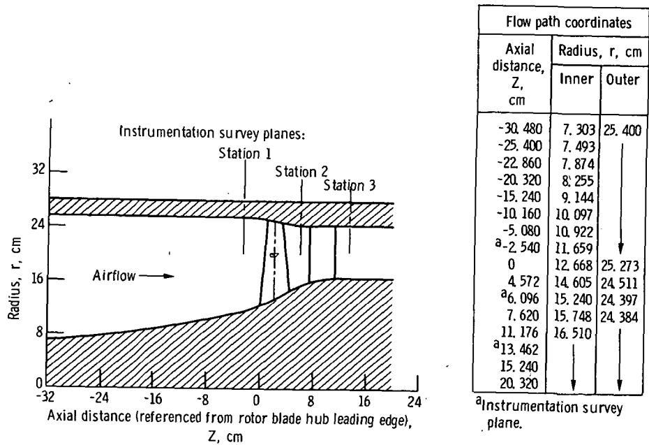
Figure 1. - Flow path for stage 18-13, showing axial location of instrumentation.
