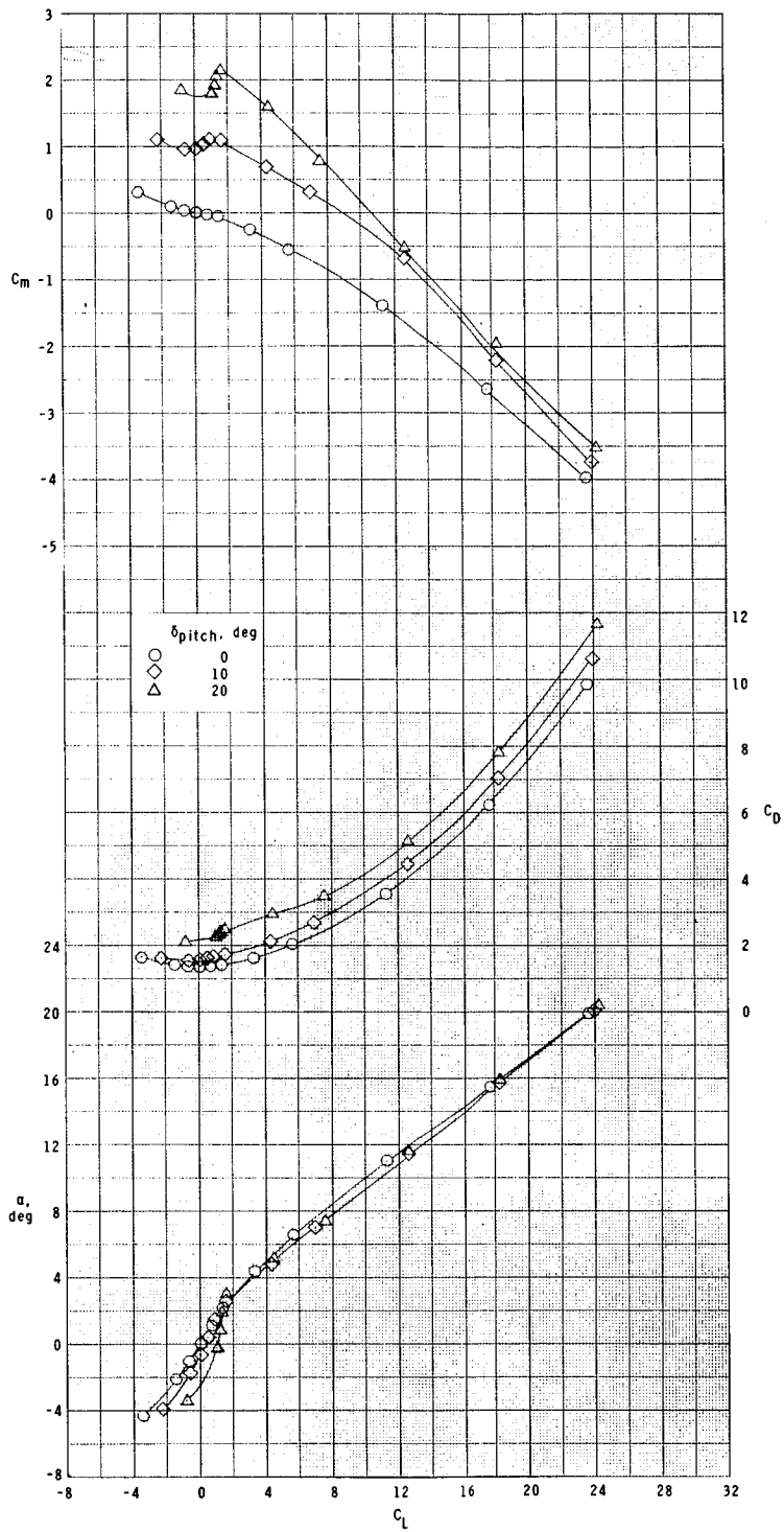
(e) Concluded. Figure 4.- Continued.
