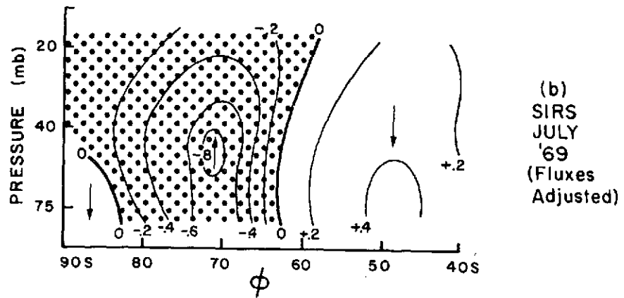
Fig. 5.10 Zonally-averaged vertical motion patterns for the S. H. for July 1969. Units: \text{mb day}^{-1} .
