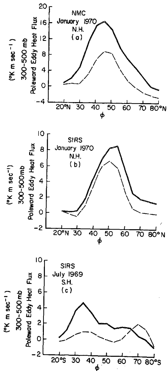
Fig. 4.9 Wintertime, total poleward eddy flux of heat, \pm [(v)_\lambda(T)_\lambda]_{\lambda,t} (solid lines), and poleward eddy flux of heat due to standing eddies, \pm [([v]_t)_\lambda([T]_t)_\lambda]_{\lambda} (dashed lines) for the layer 300-500 mb in both hemispheres.
