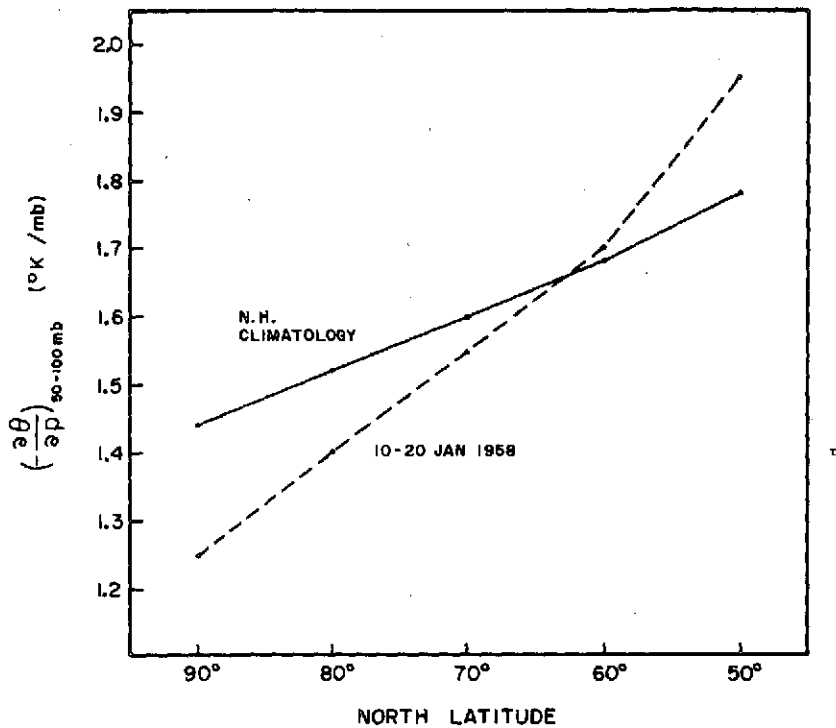
Fig. 5.1 Static stability (-\frac{\partial\theta}{\partial p}) in the layer 50-100 mb as a function of latitude in the Northern Hemisphere for January.
