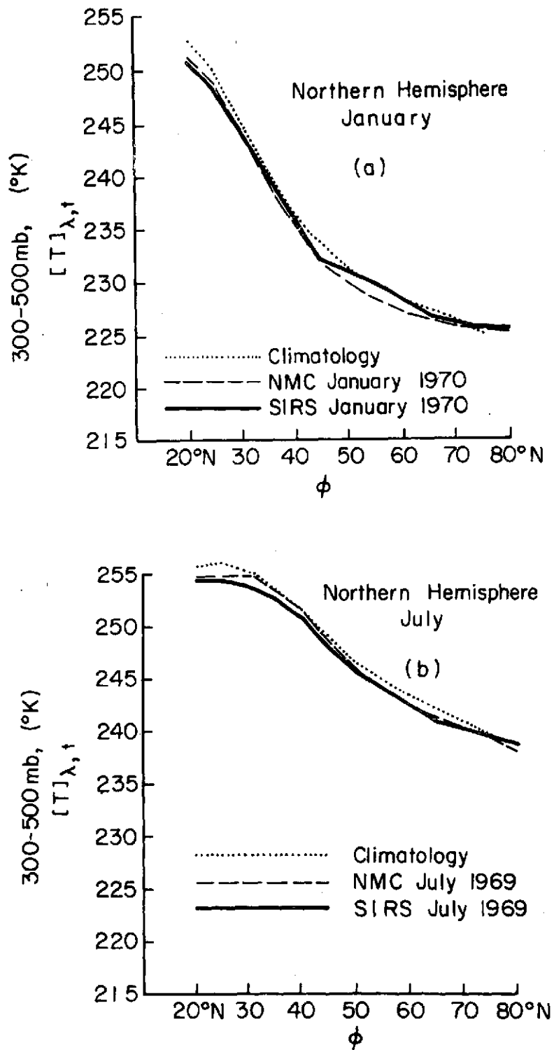
Fig. 4.1 Mean meridional temperature gradients in the upper troposphere (300-500 mb) in the Northern and Southern Hemispheres for January and July.
