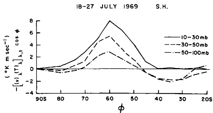
Fig. 5.15 Poleward heat fluxes in the S. H. during the periods (a) 1-10 July and (b) 18-27 July 1969.
