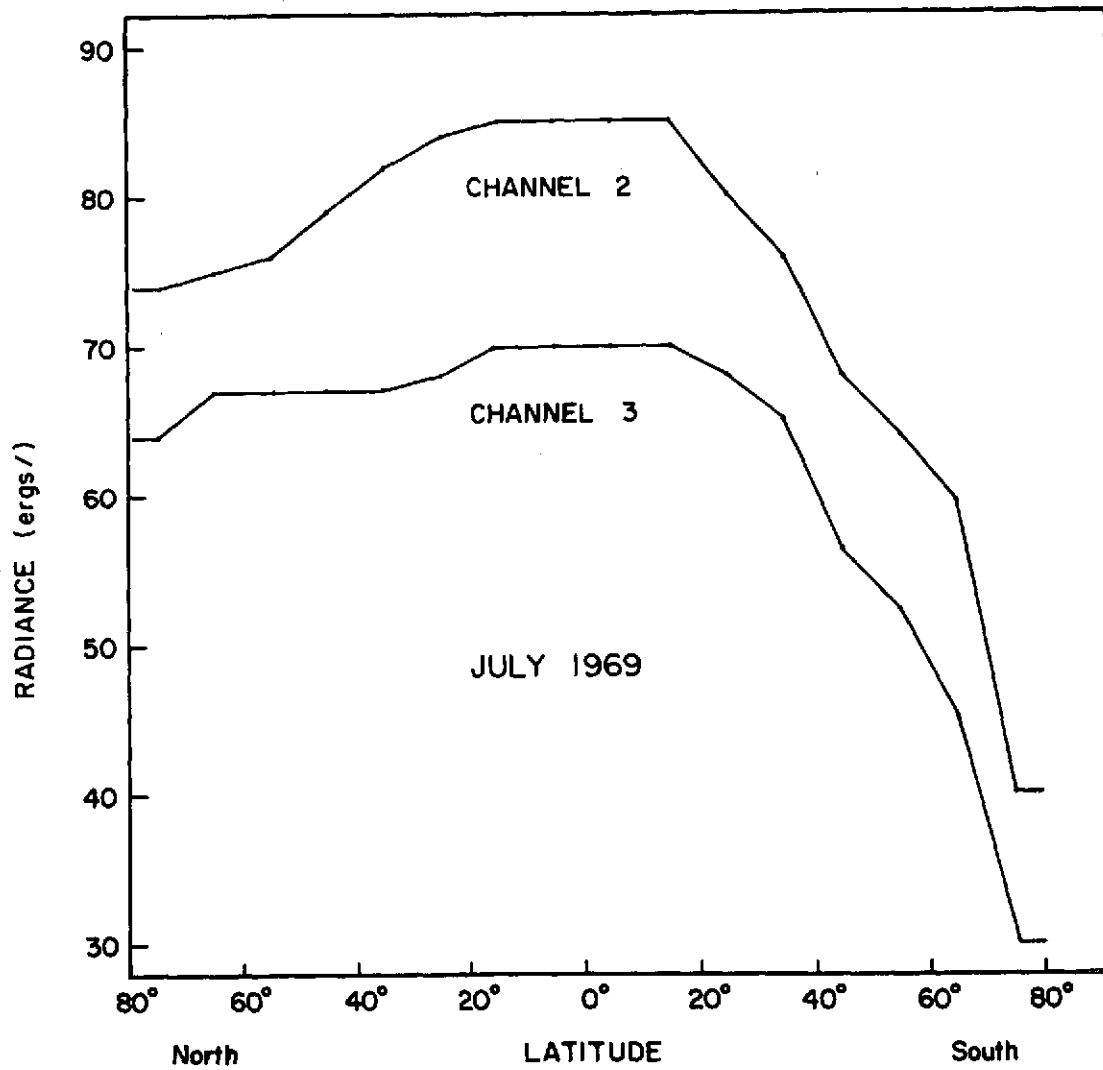
Fig. 3.3 The distribution with latitude of critical values of channels 2 and 3 for the cloud check procedure for July 1969.
