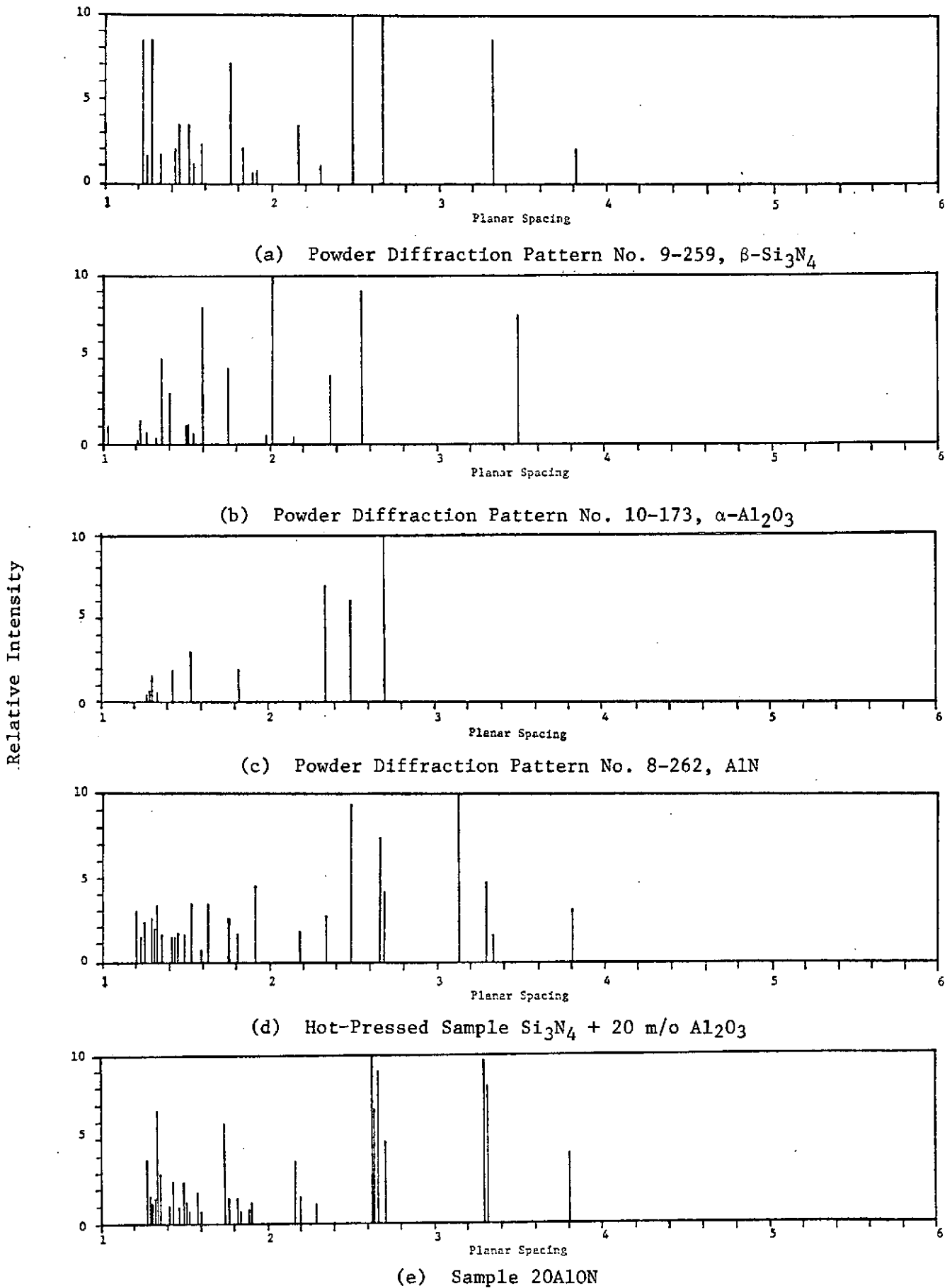
FIGURE 9. DUAL ADDITIVE SIALON, COMPOSITION 20AlON
