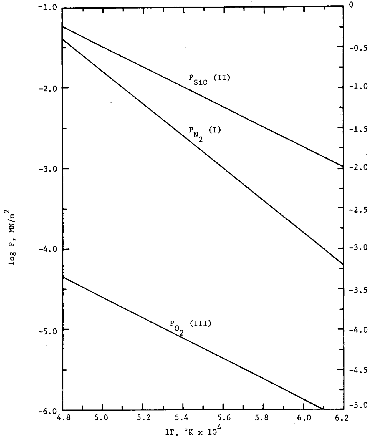
FIGURE 1. GAS PHASE PARTIAL PRESSURE RELATIONSHIPS FROM POTENTIAL REACTIONS
