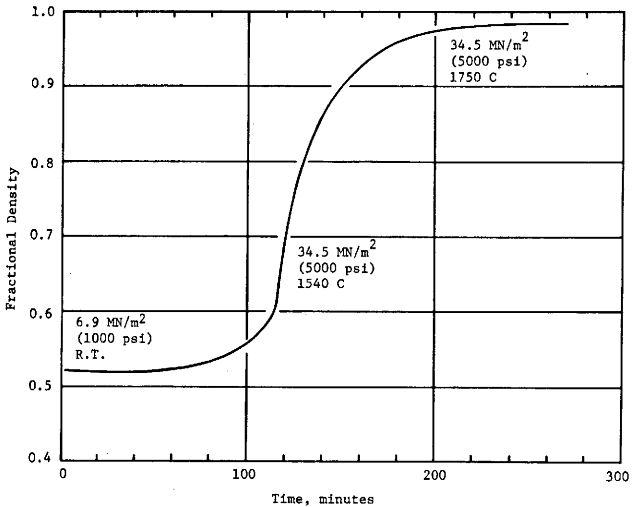
FIGURE 11. TIME-DENSITY RELATIONSHIP FOR HOT-PRESSING \text{Si}_3\text{N}_4\text{-Mg}_3\text{N}_2 TEST BILLETS.
