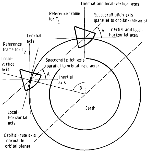
Figure 1. - Displacement of the local-vertical reference frame with respect to the inertial reference frame (for an unperturbed spacecraft in a circular orbit).
