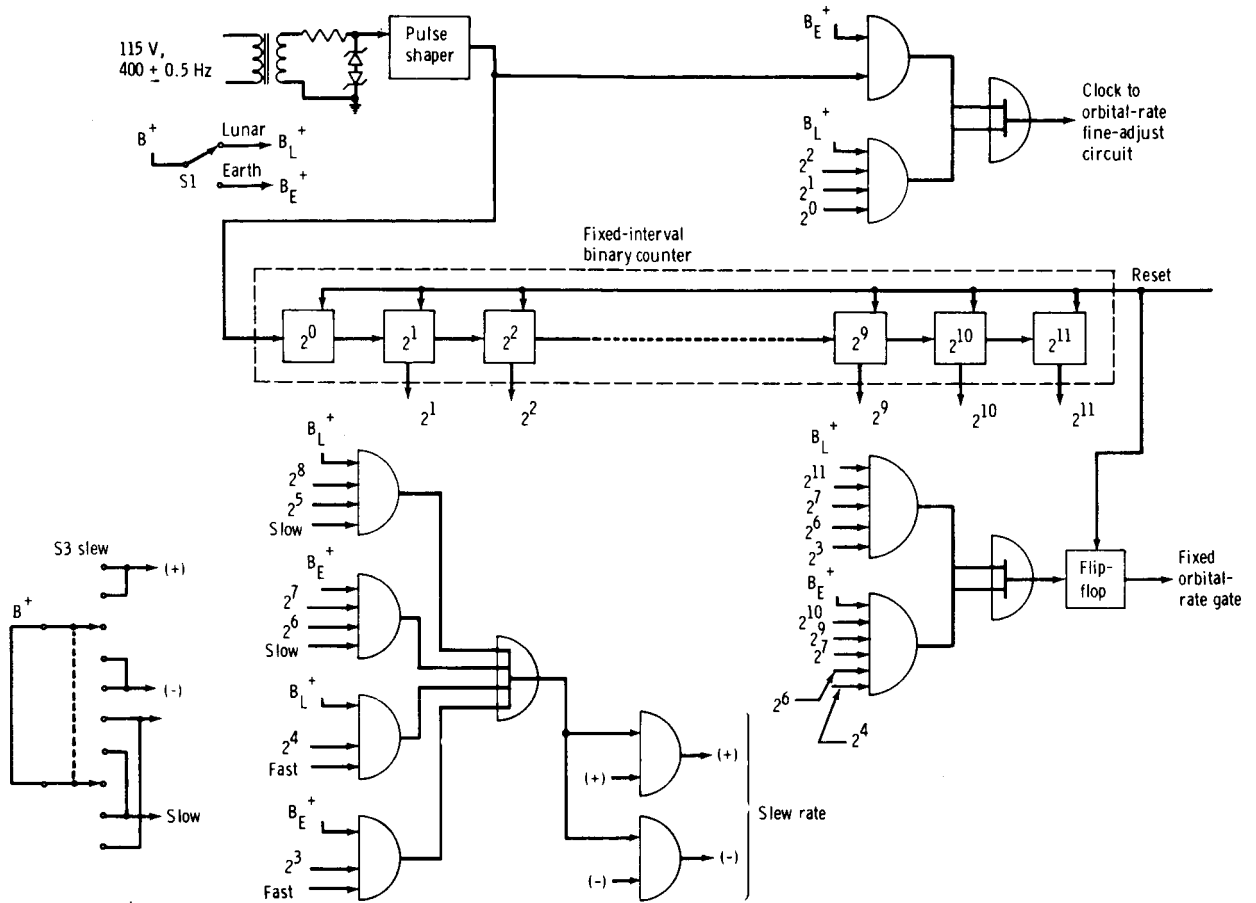
(a) Counter and gate circuitry and slew-rate circuitry.
