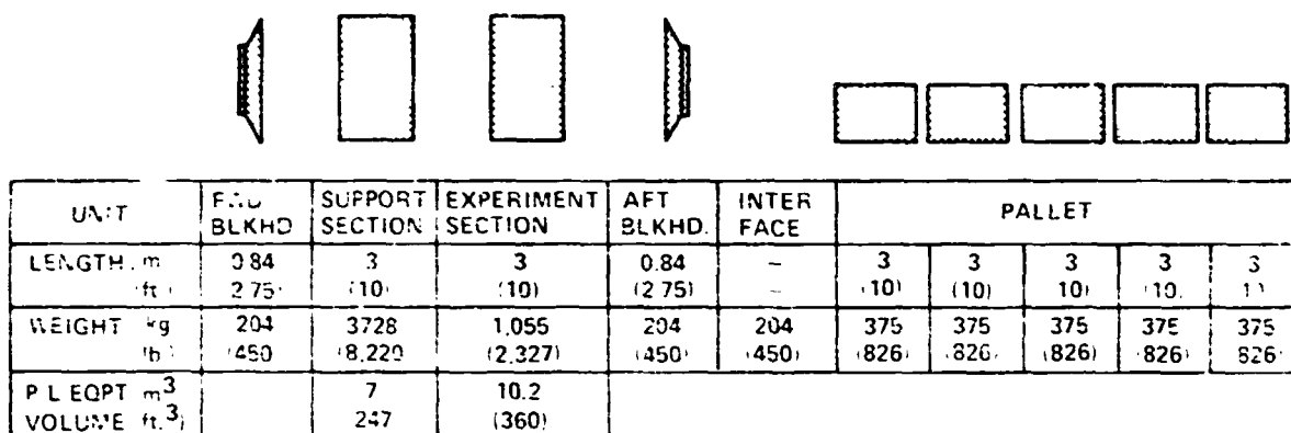
Figure 3. NASA/ESRO Spacelab Configuration Definition
