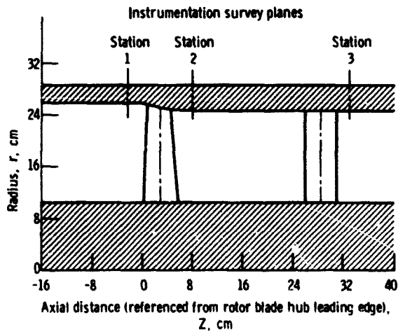
Figure 1. - Flow path for stage 52-52 showing axial location of instrumentation.
