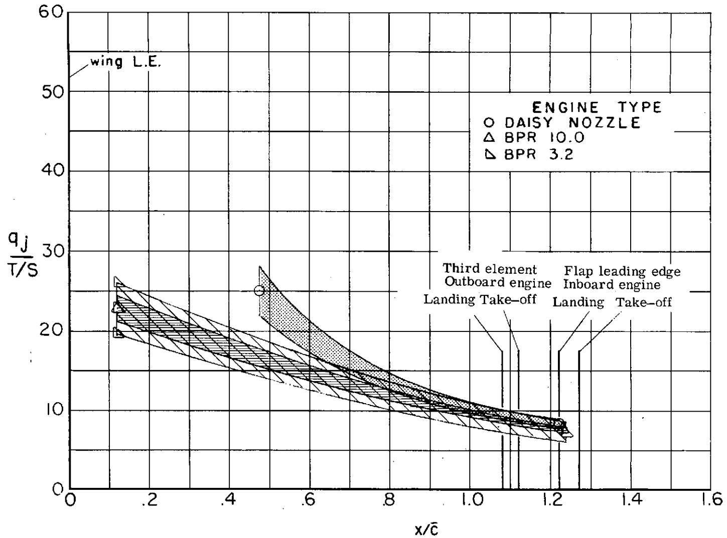
(b) Daisy nozzle; bypass ratios 10.0 and 3.2.
