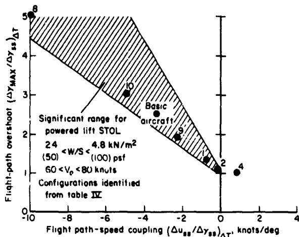
Figure 29.- Interrelationship between flight-path overshoot and flight-path/speed coupling parameters.
