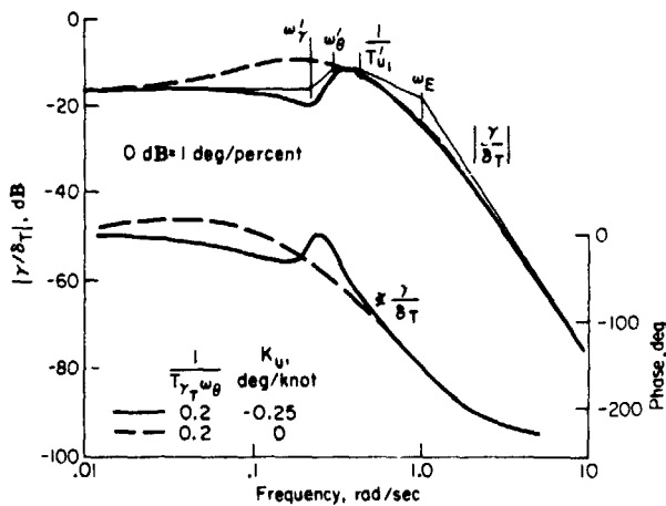
Figure 18.- Flight-path control with thrust with airspeed control by pitch attitude (rate command attitude control system).
