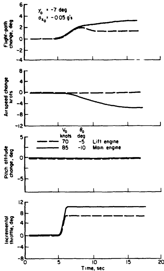
Figure 38.- Flight-path and airspeed response to a thrust change for the D0-31 during a step, decelerating approach.
