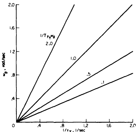
Figure 21.- Relationship between \tau_{\gamma} and \omega_{\theta} .
