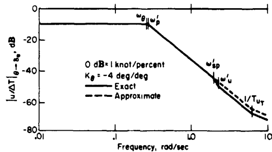
Figure 52.- Comparison of exact and approximate airspeed response to thrust with pitch attitude stabilized.
