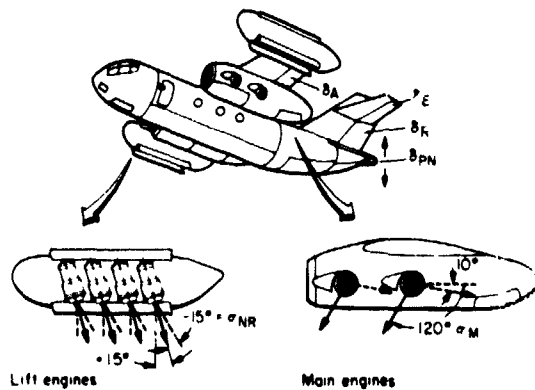
Figure 36.- Dornier DO-31 jet VTOL transport.
