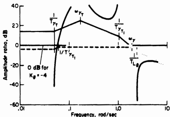
Figure 47.- Influence of pitch attitude stabilization on the roots of the numerator of the flight-path to thrust transfer function.
