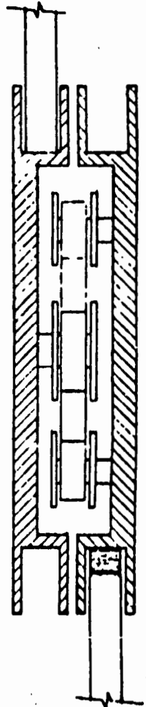
FIGURE 1-7. TAPE TENSIONING CONFIGURATION USING NEG'ATOR SPRING
