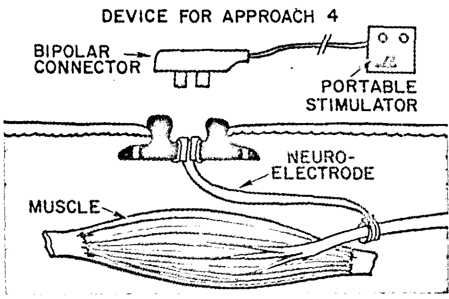
Fig 5--Illustration of system for neuroelectrodes (or other wire electrodes.)
