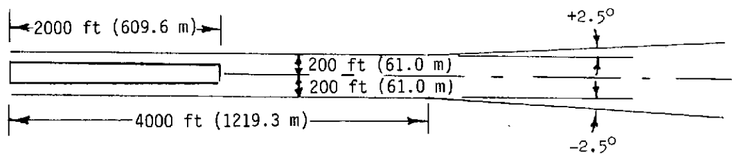
(b) Localizer.
