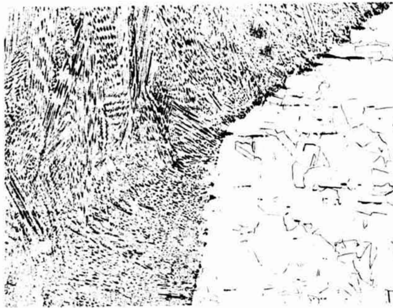
FIGURE A-47. FUSION LINE REGION AT SHAPE CHANGE
