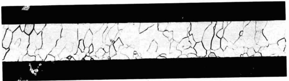
FIGURE B-39. CHORD SECTION IN S/N 145 SKYLAB
