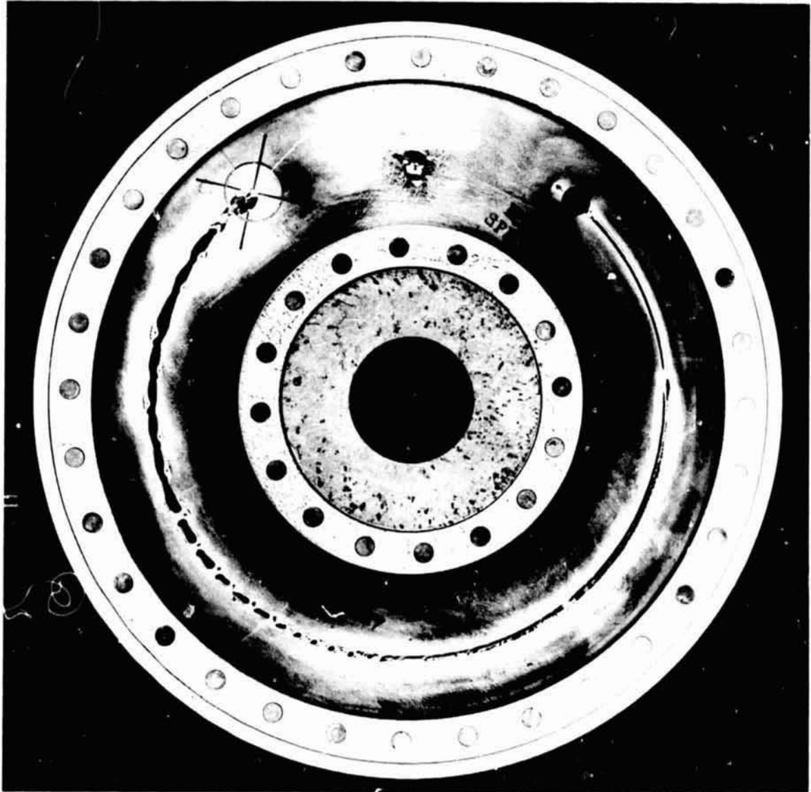
FIGURE B-32. FRONT SURFACE S/N 1-7
