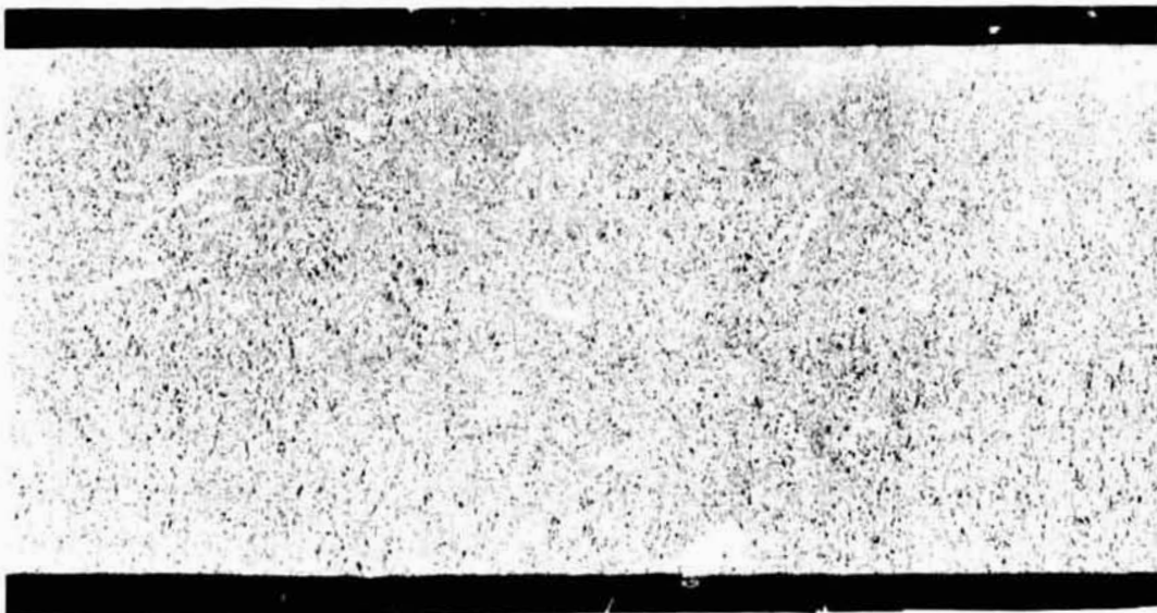
FIGURE E-10. CHORD SECTION IN FULL PENETRATION REGION - S/N 129
