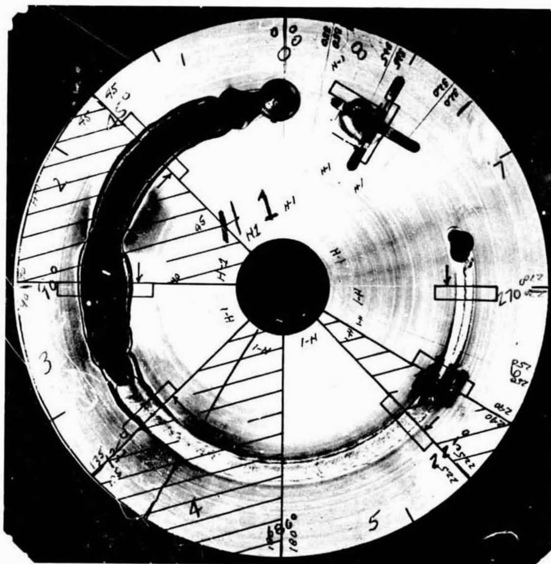
FIGURE A-4. FRONT SURFACE H-1
