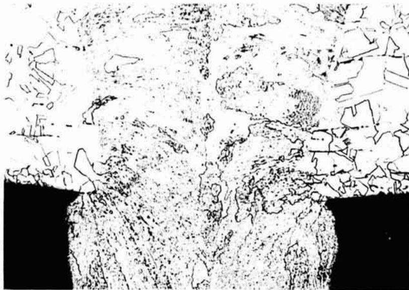
FIGURE A-45. SECTION AT ROOT OF WELD
