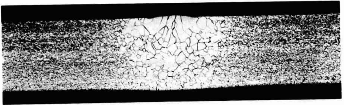
FIGURE B-38. SECTION THROUGH PARTIAL PENETRATION REGION - S/N 145 SKYLAB
