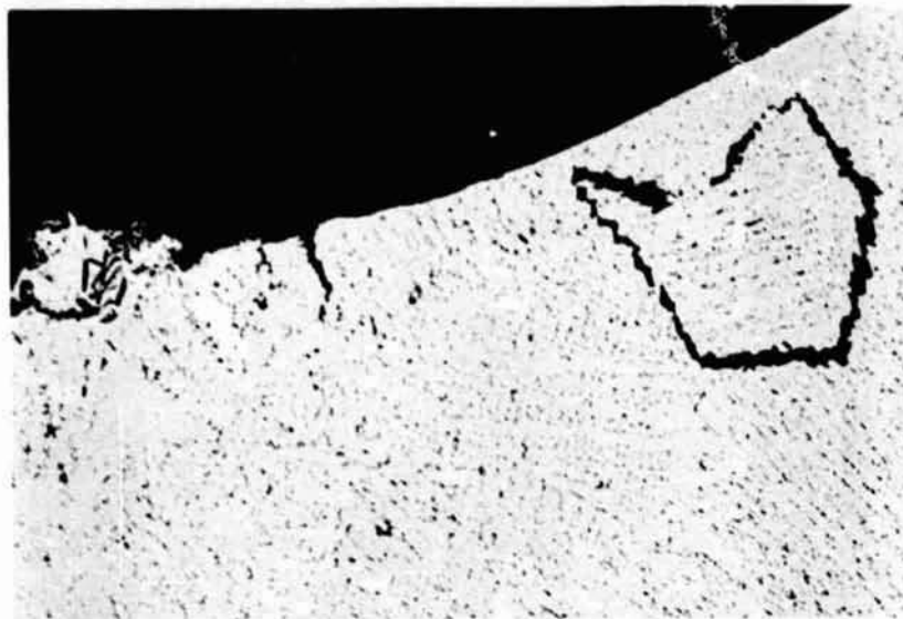
FIGURE A-22. CRACKS NEAR TOP OF DWELL REGION- H-1
