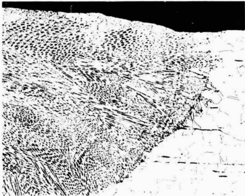
a. Fusion Line at Top
