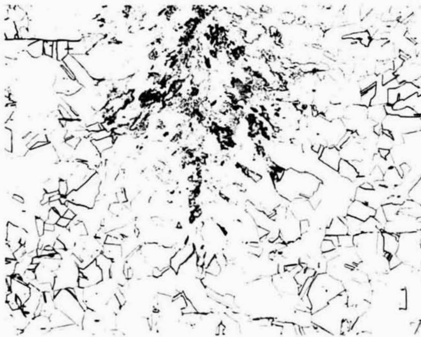
Fusion Line
