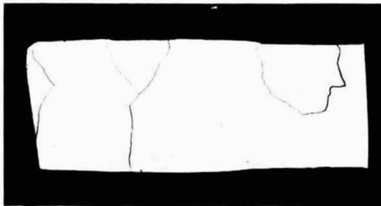
FIGURE A-63. CHORD SECTION THROUGH DWELL REGION S/N 143
