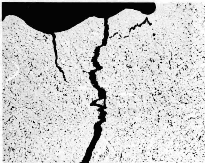
b. Main crack near center in Figure A-19
