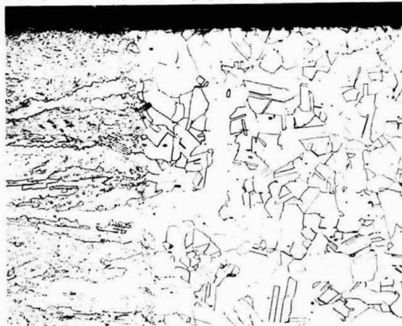
FIGURE B-27. CONTOUR OF TOP FUSION LINE AREAS IN DWELL REGION - S/N 106 SKYLAB
