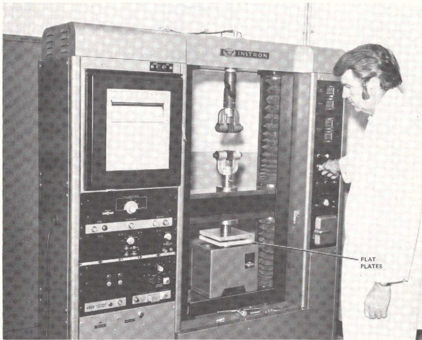
Figure 3. Instron Testing Machine with crush test setup.
