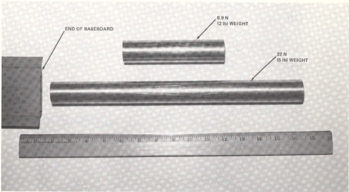
Figure 7. Impact test weights.
