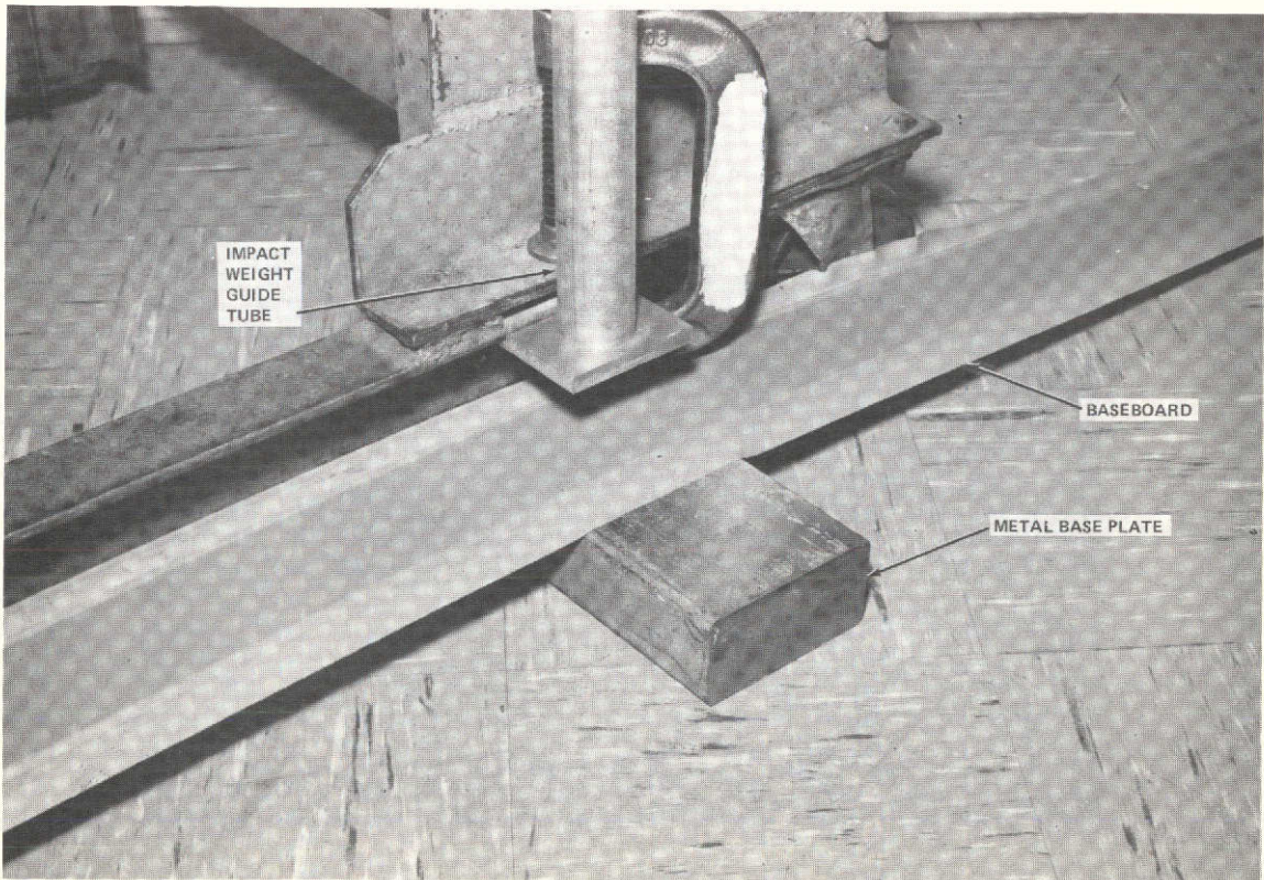
Figure 8. Baseboard in impact test position.
