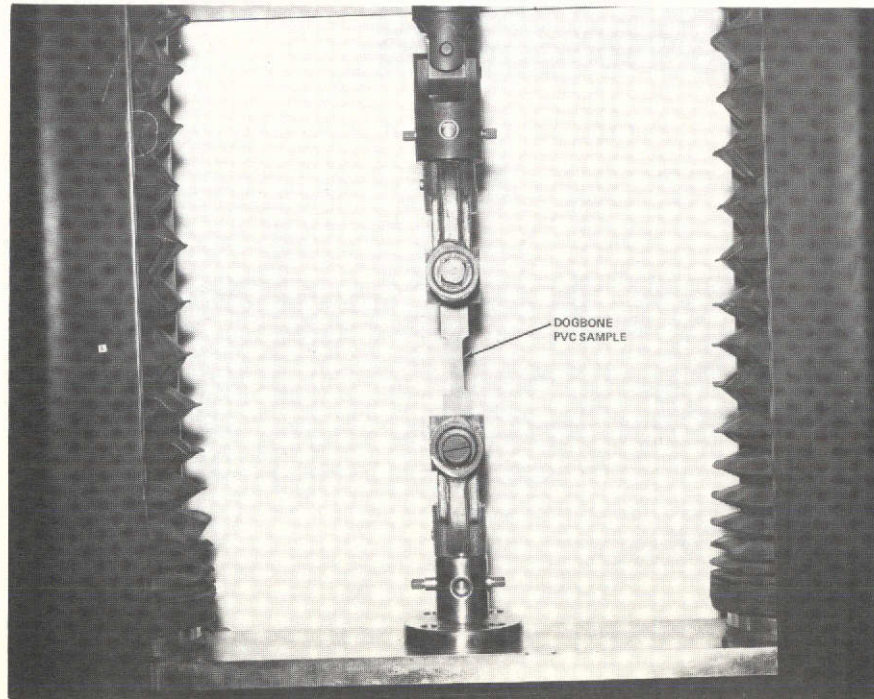
Figure 12. Tensile test setup.
