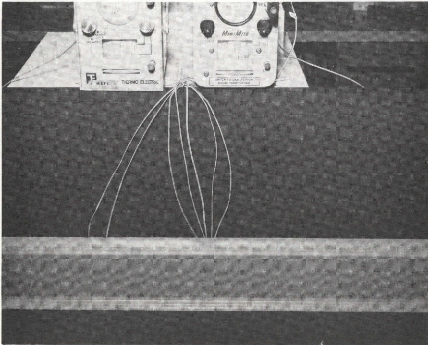
Figure 10. Heat test thermocouple wires.
