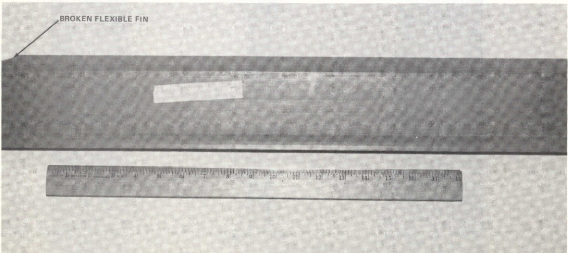
Figure 14. Low temperature dropped sample.
