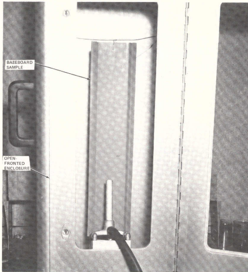
Figure 15. Flame test setup.
