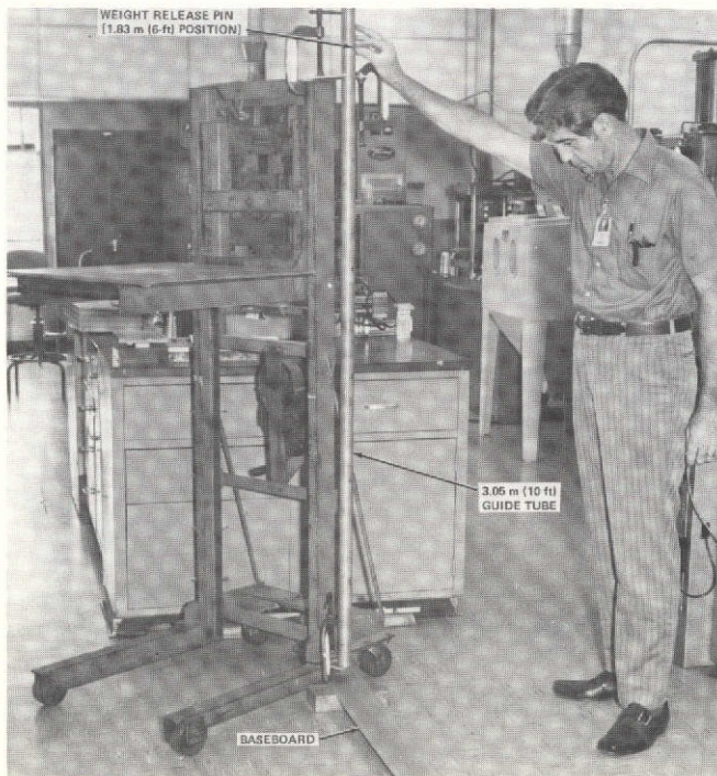
Figure 6. Impact test setup.
