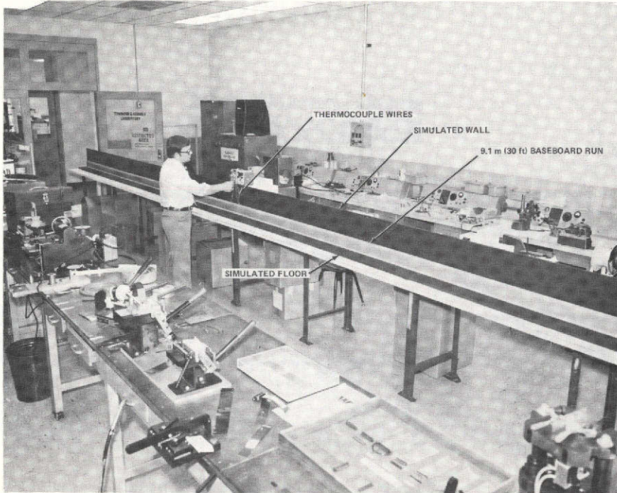
Figure 9. Heat test setup.
