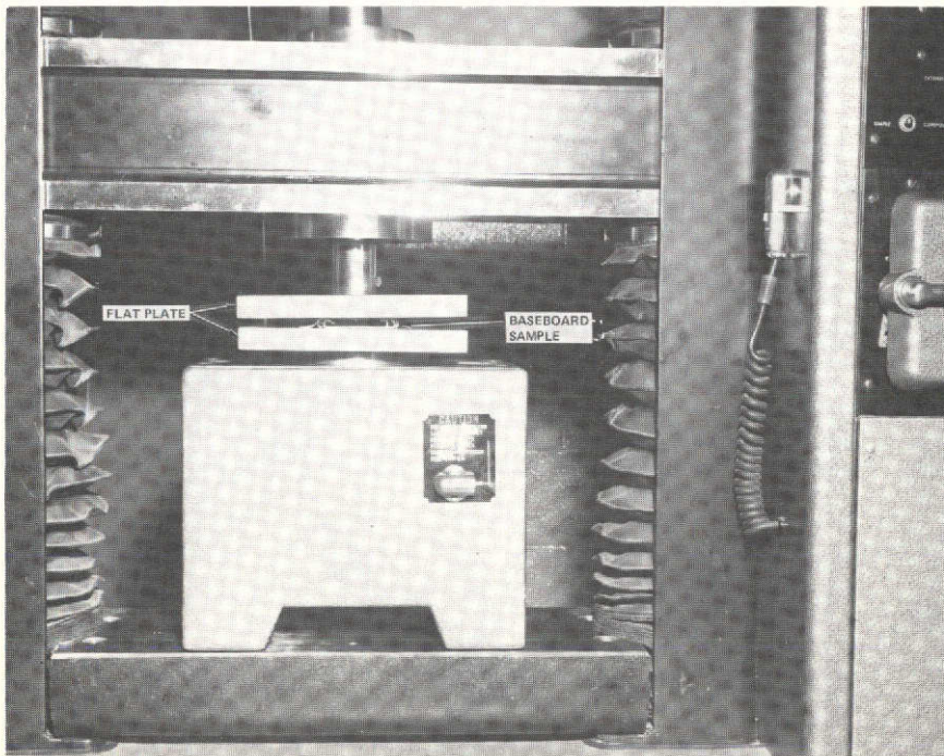
Figure 4. Crush test sample between flat plates.
