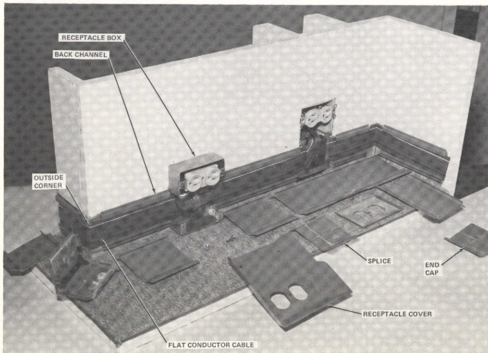
Figure 2. Unassembled baseboard display.
