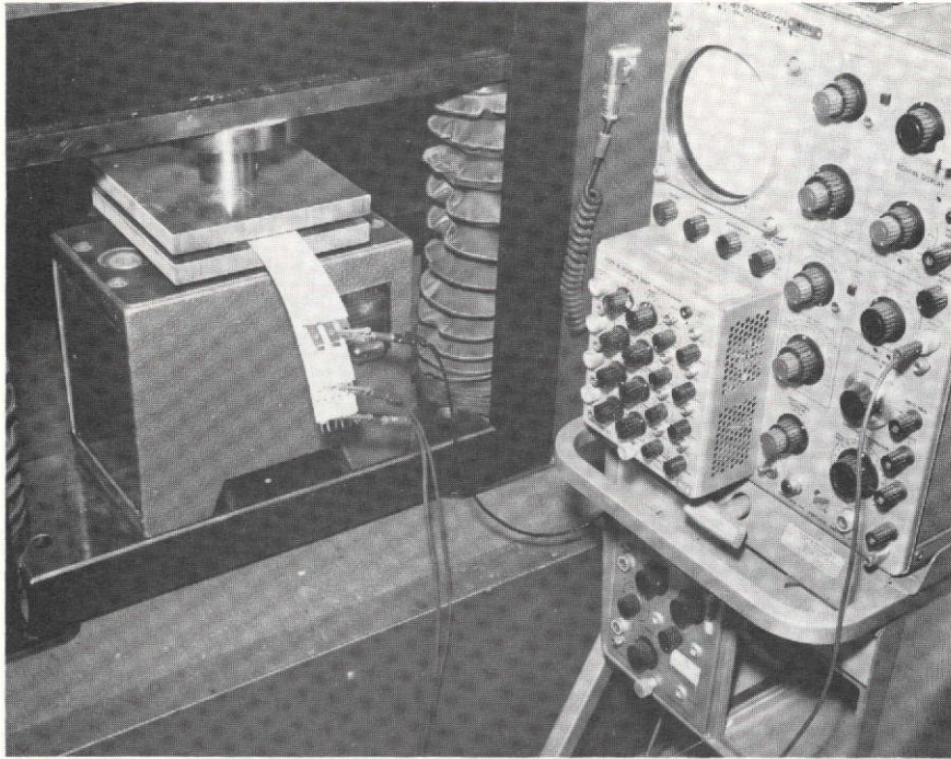
Figure 5. Crush test setup with cables.
