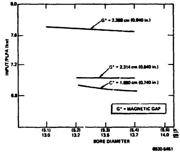
Figure 48. Power Input vs Bore Diameter for Dual Helical PLPA [25.4 cm (10 in.) stack length, 24.9 cm (9.8 in.) OD]
