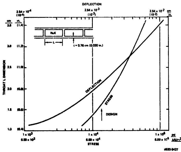
← Figure 34. Linear Pump Throat Deflection and Stress
