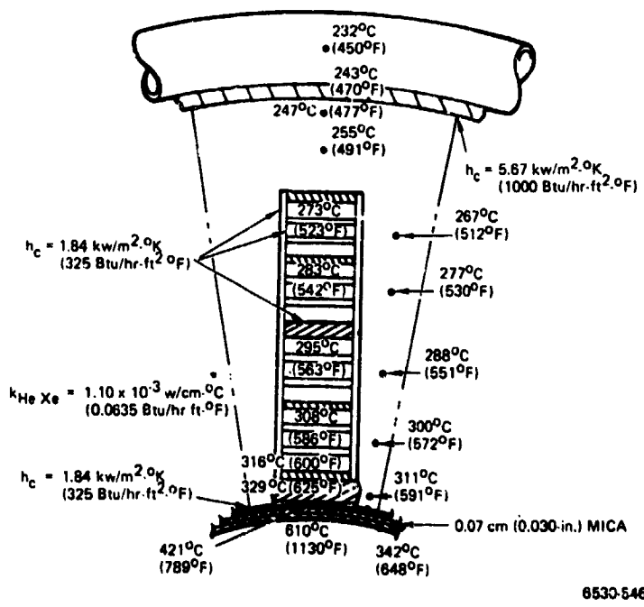
Figure 64. Effect of High Thermal Conductivity Gas on Helical Pump Slot Temperatures – Design No. 74
