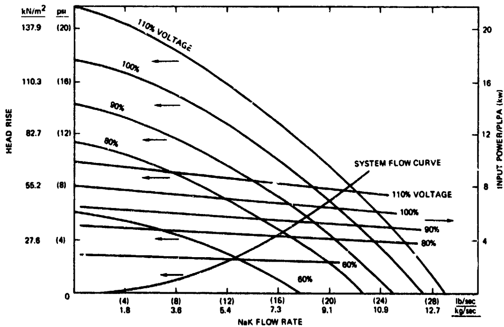
Figure 56. Head Rise vs Flow Rate for Dual Helical PLPA [Design No. 74, 610°C (1130°F) NaK rated at 43.4 v and 46 Hz]
