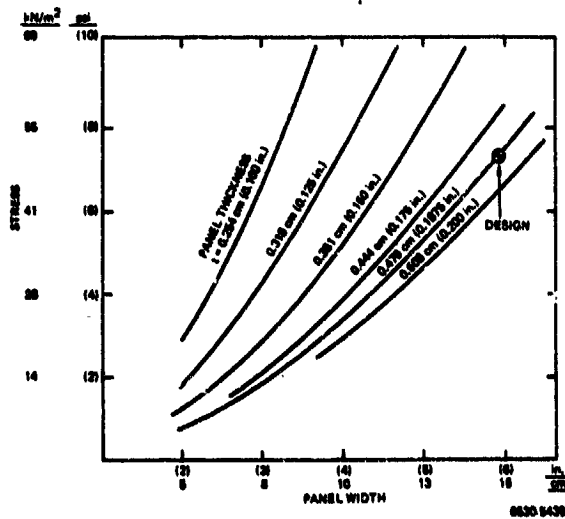
← Figure 36. Outer Gas Shell Stress for Linear Pump [103 \text{kN/m}^2 (15 psi) internal pressure]
