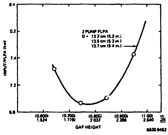
Figure 49. Power Input vs Gap Height for Dual Helical PLPA [25.4 cm (10 in.) stack length]
