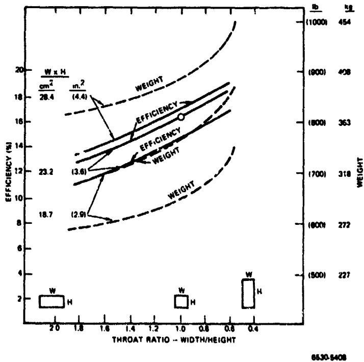
Figure 9. Efficiency and Pump Weight vs Throat Aspect Ratio for dc PLPA (Uncompensated 3-pump PLPA)
