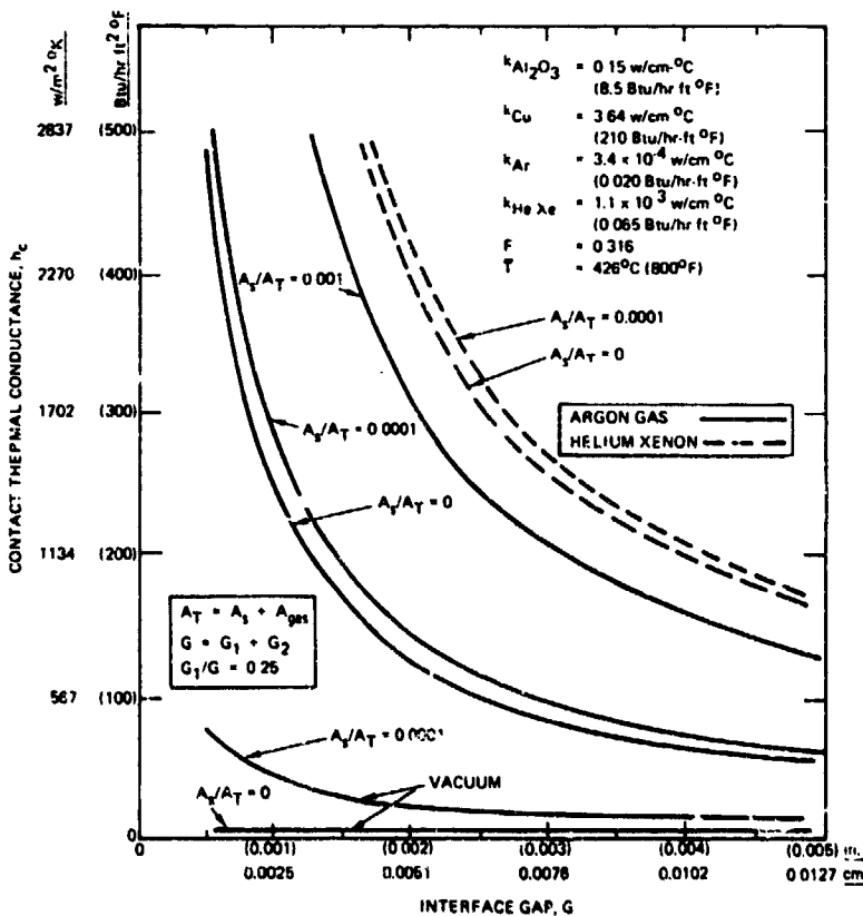
Figure 59. Thermal Conductance Across Interfaces
