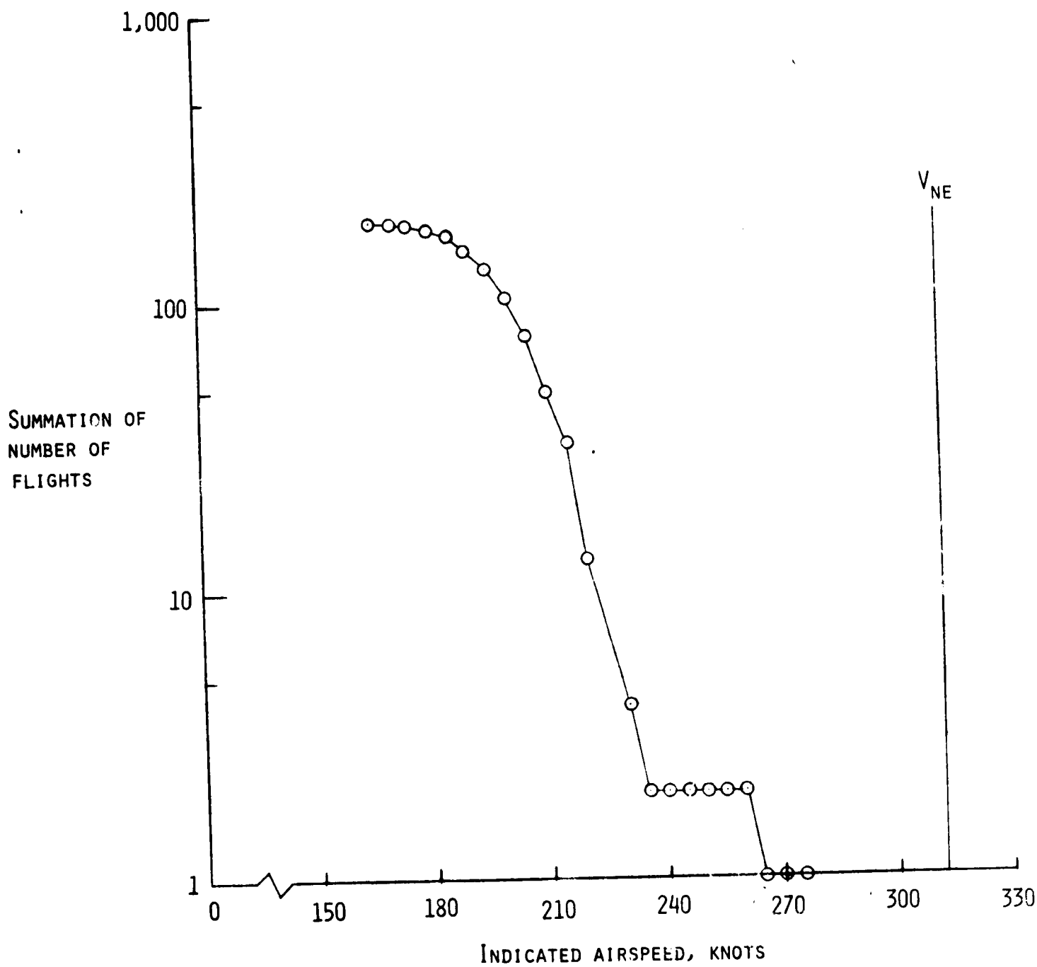
FIGURE 11. - RELATIONSHIP OF THE MAXIMUM INDICATED AIRSPEED RECORDED DURING A FIRE FIGHTING FLIGHT TO THE PLACARD NEVER-EXCEED SPEED.
