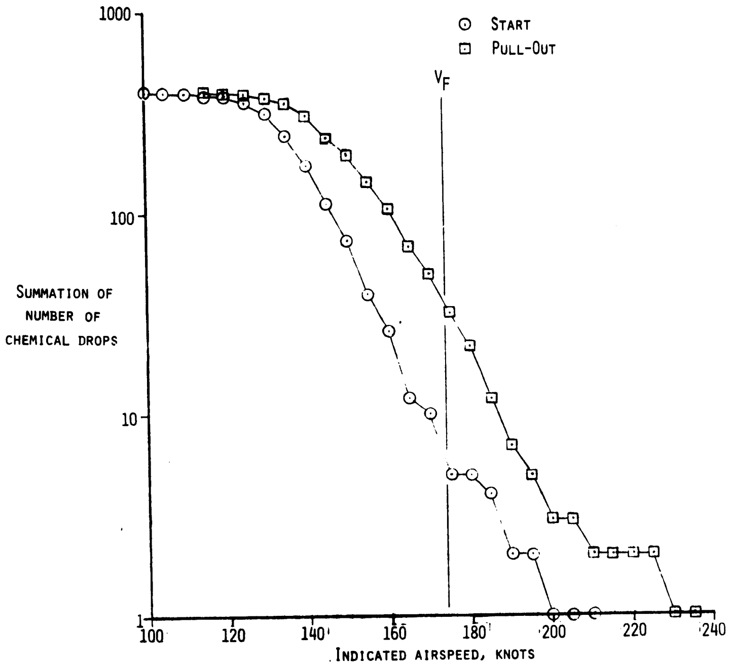
FIGURE 5. - RELATIONSHIP OF SPEED DURING RETARDANT DROP RUN TO THE DESIGN FLAP SPEED.
