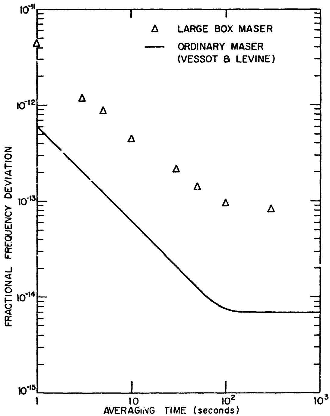
Figure 5. Fractional Frequency Deviations of Large Storage Box Maser (cone out, low flux, \nu_2 = 15 kHz)
