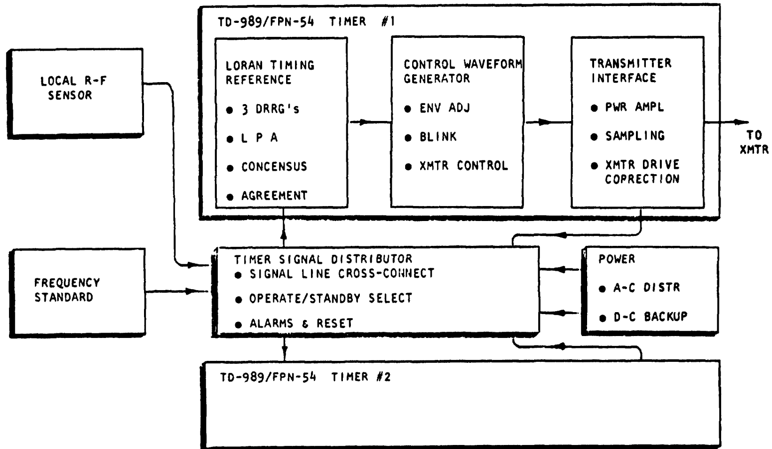
Figure 3. AN/FPN-54 (COLAC) Loran-C Timer Set
