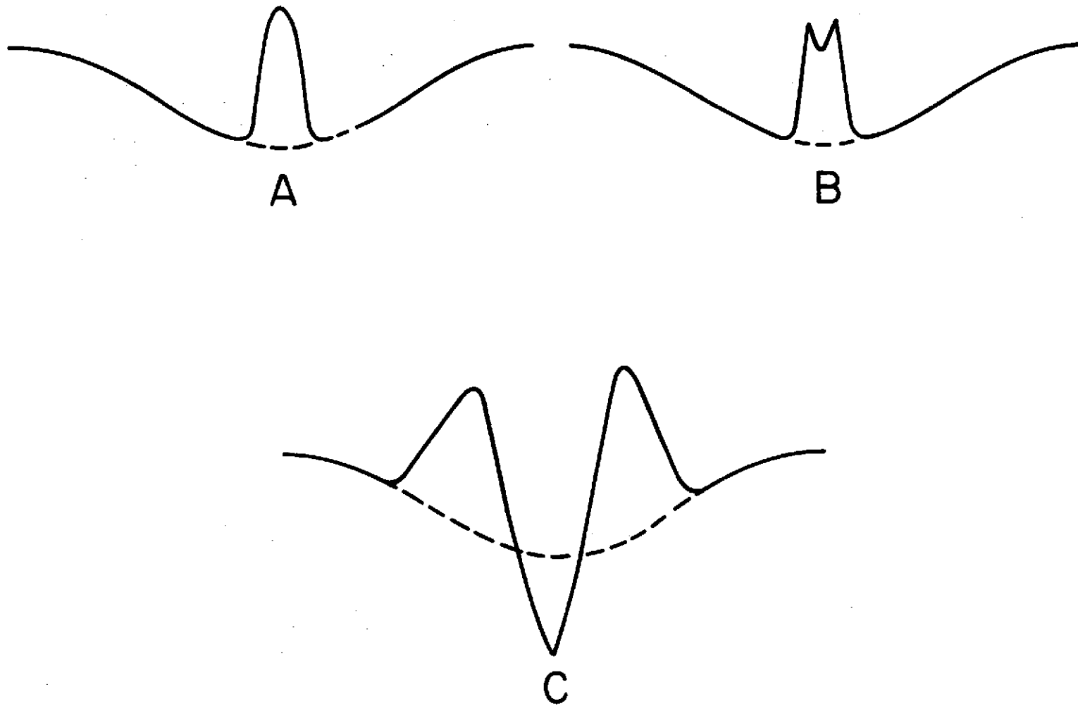
Fig. 1 Be AND Fe SHELL HYDROGEN LINE PROFILES
