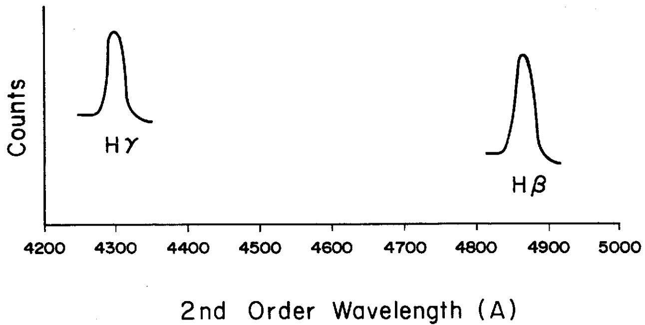
FIG. 5 SCANNING REGIONS FOR H \beta AND H \gamma
