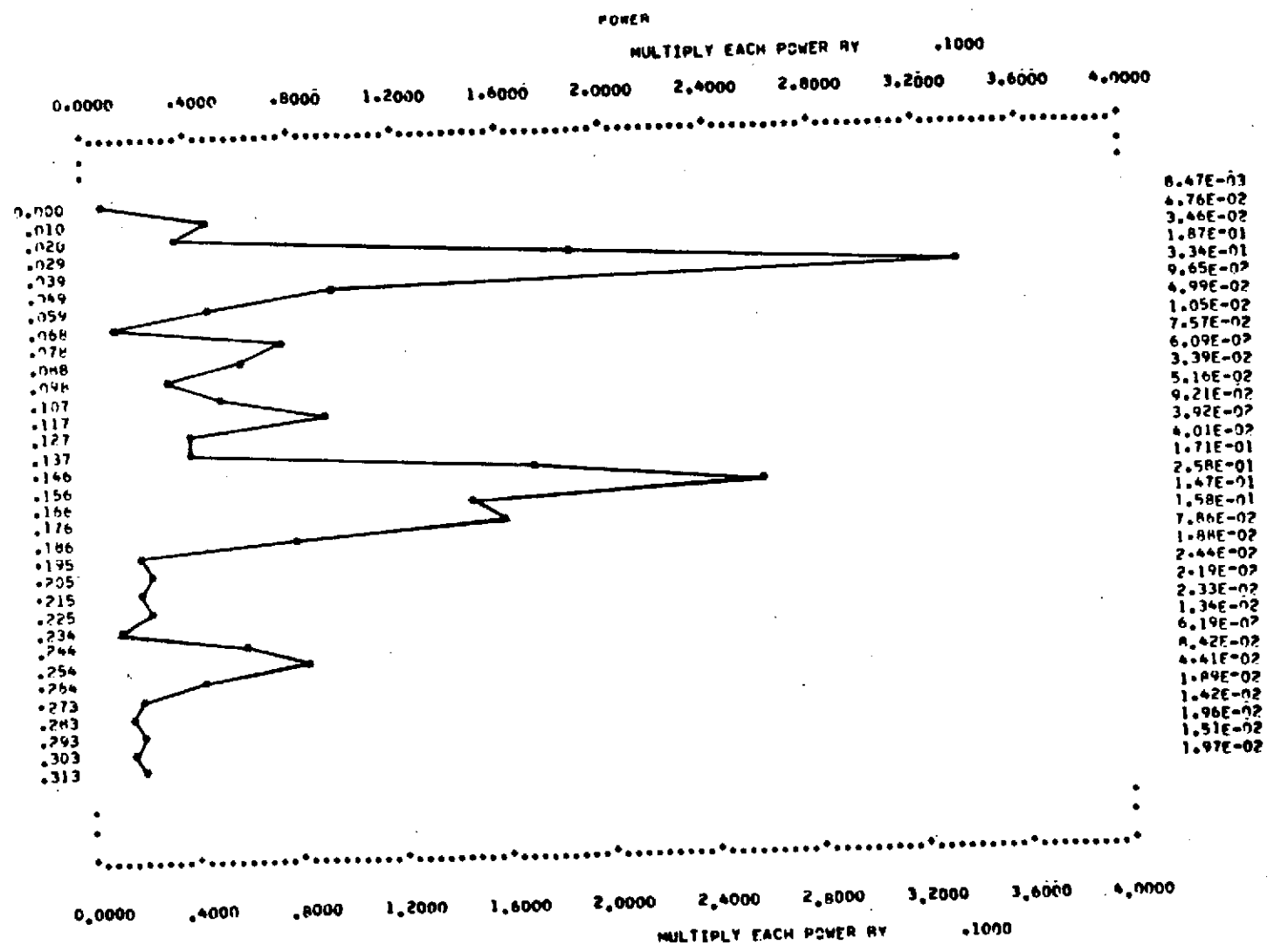
Fig. 11 POWER SPECTRUM FOR 28 TAU, HY, 12 OCTOBER 1972 (UT) Abscissa: Frequency (min -1 ) Ordinate: Power
