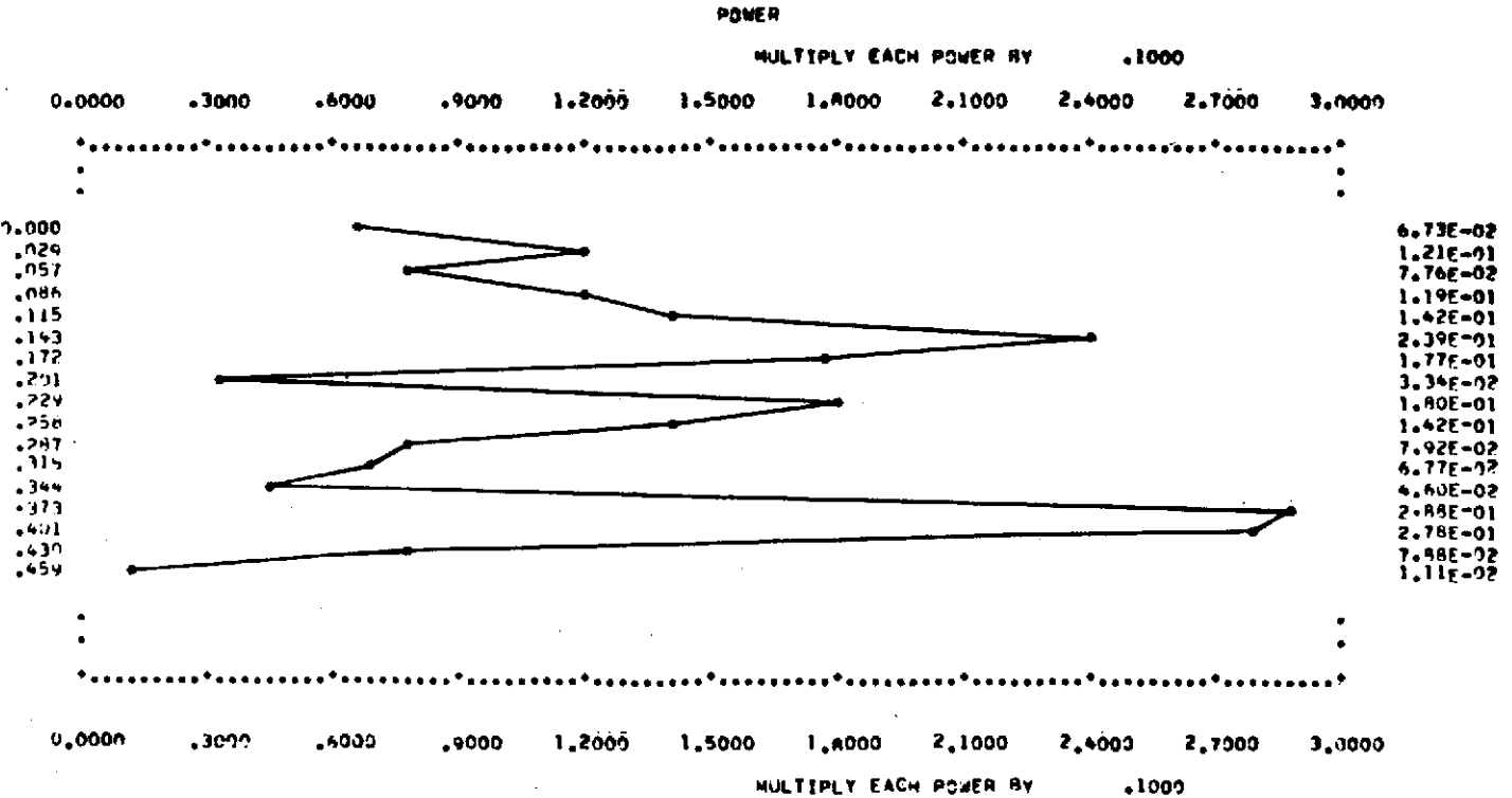
FIG. 10 POWER SPECTRUM FOR 48 PER, Hc, 10 OCTOBER 1972 (UT) Abscissa: Frequency (min -1 ) Ordinate: Power
