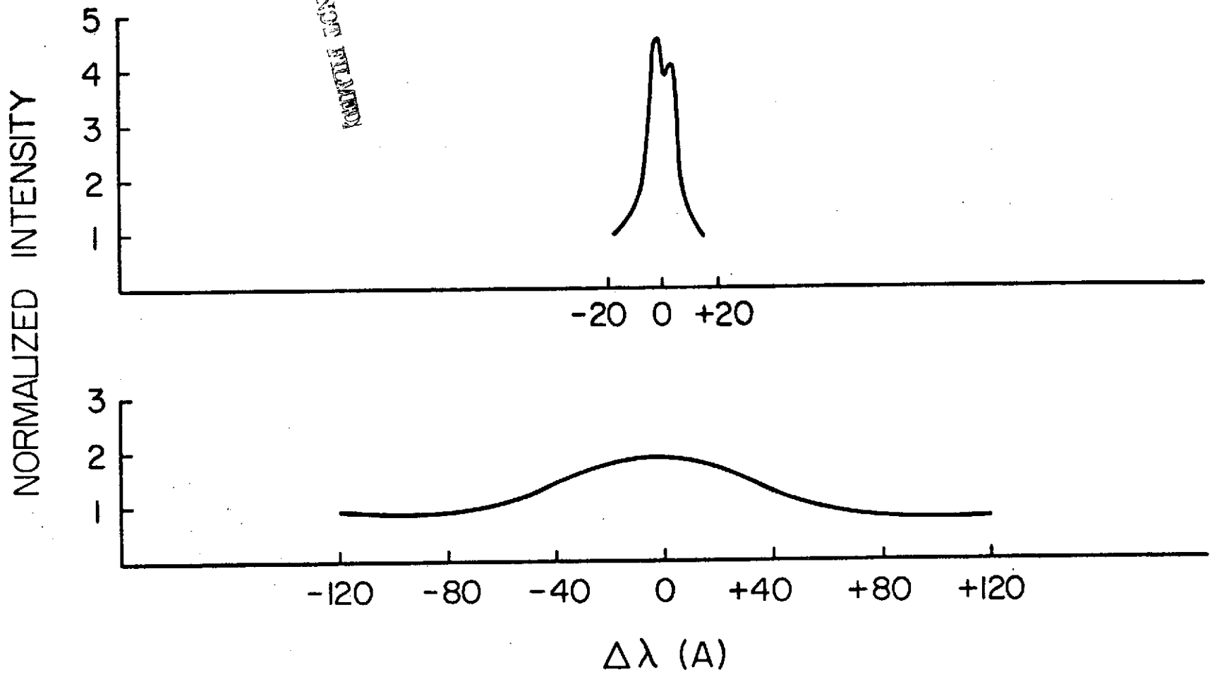
Fig. 4 EFFECT OF LOW SPECTRAL RESOLUTION ON OBSERVED LINE PROFILE
