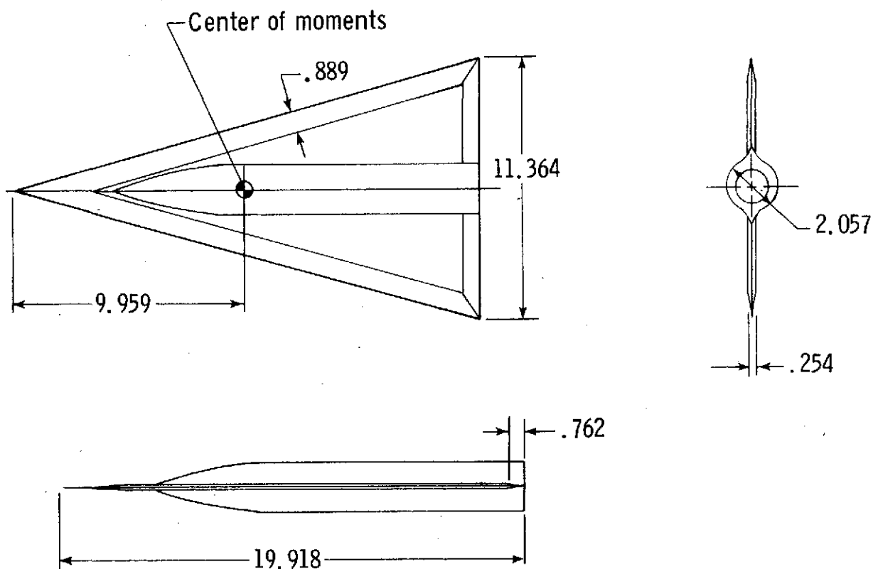
Figure 18.- 74° delta-wing model tested in low-speed cryogenic tunnel. Dimensions in centimeters.
