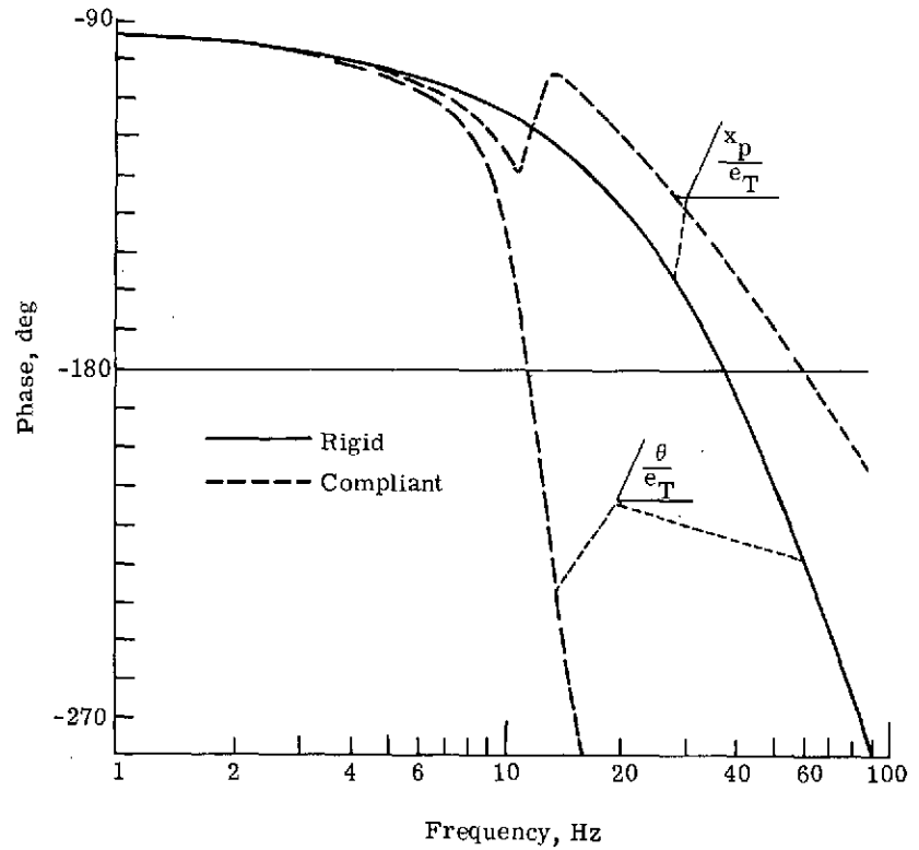
(b) Phase.
