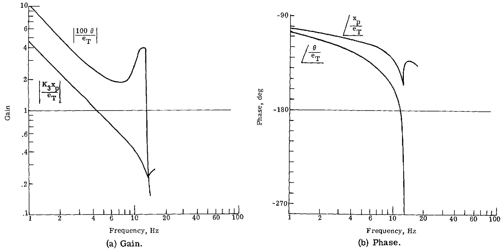
Figure 7.- Open-loop frequency response from experimental data.
