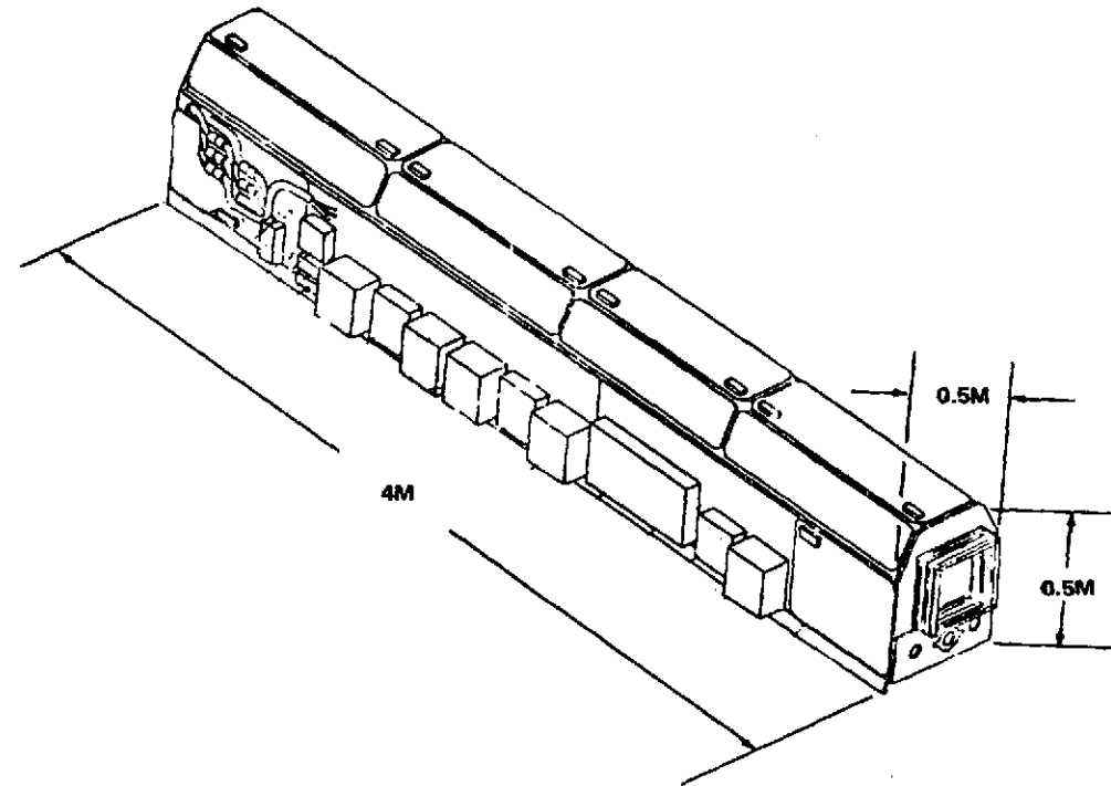
SO020 SOFT X-RAY SPECTROGRAPH TELESCOPE
