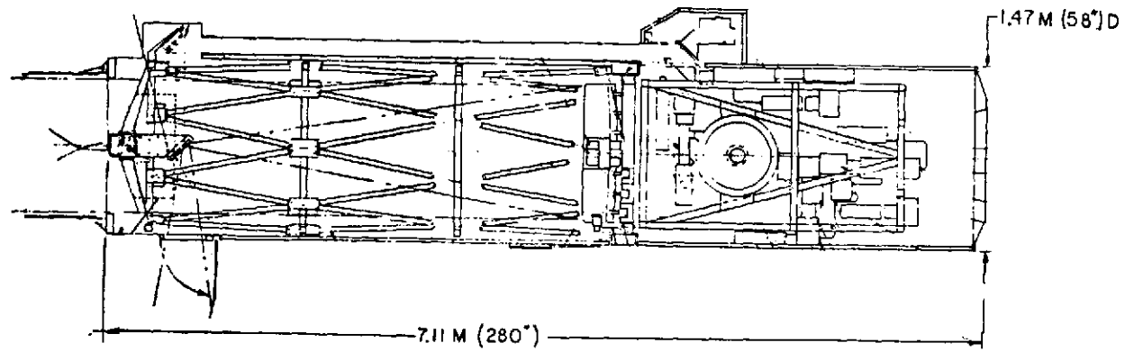
S0 007 SPECTROMETER, 60FT X-RAY/SPECTROHELIOGRAPH
