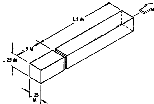
S0 008 PHOTOMETER, GRID COLLIMATOR, ACQUISITION
