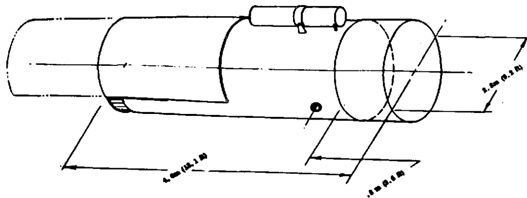
AS020S 2.5 m CRYO-COOLED IR TELESCOPE
