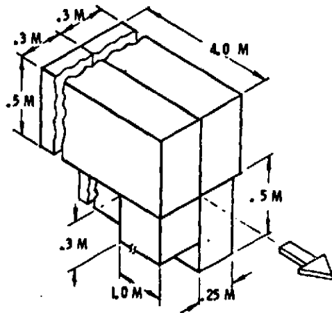
S0 007 SPECTROMETER, 60FT X-RAY/SPECTROHELIOGRAPH
