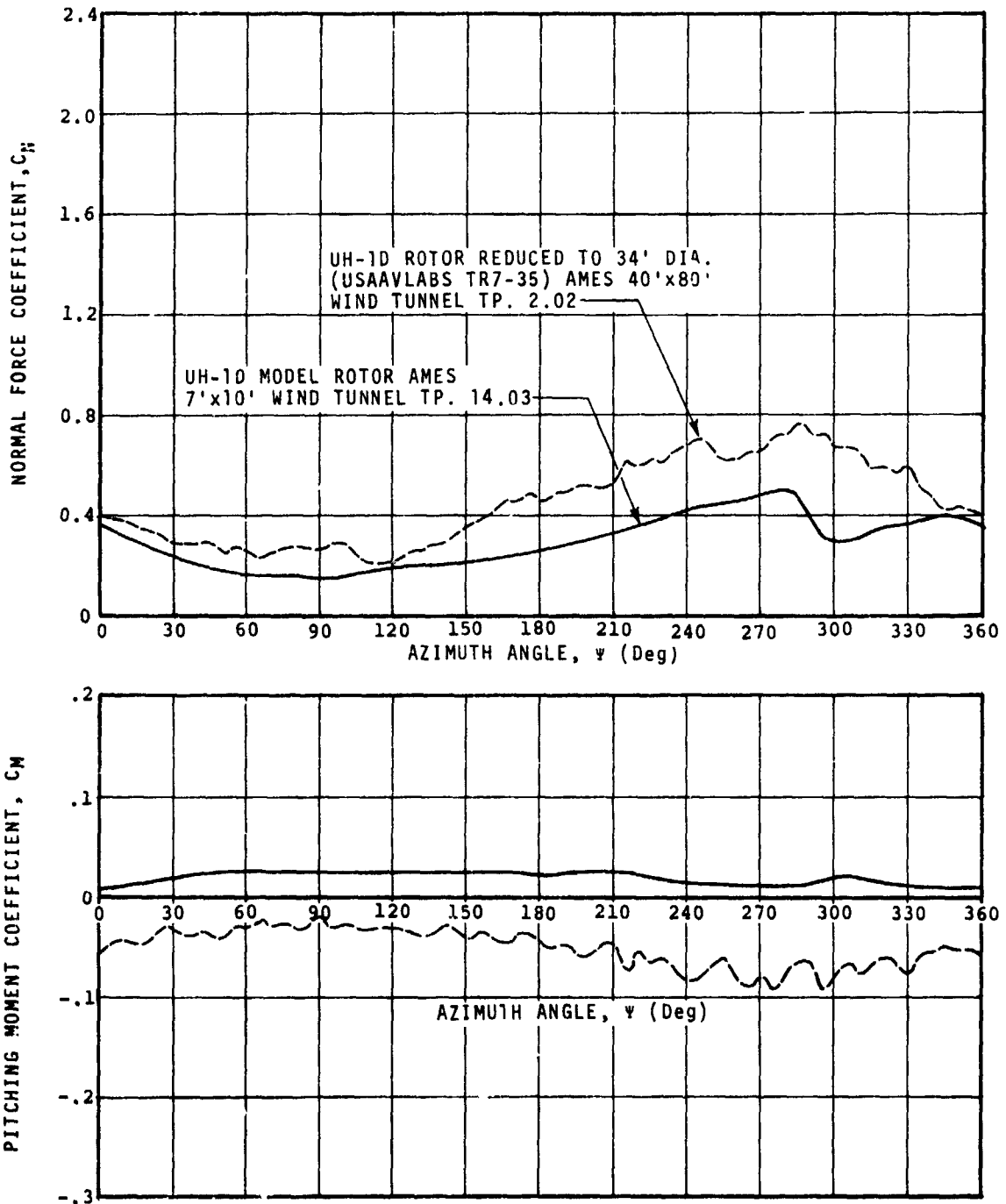
FIGURE 13 INTEGRATED LOADS FOR TEST POINT 14.03, \mu=0.195 , M_{1,90}=0.296 , \theta_{.75R}=3.1^\circ COMPARISON WITH FULL SCALE DATA
