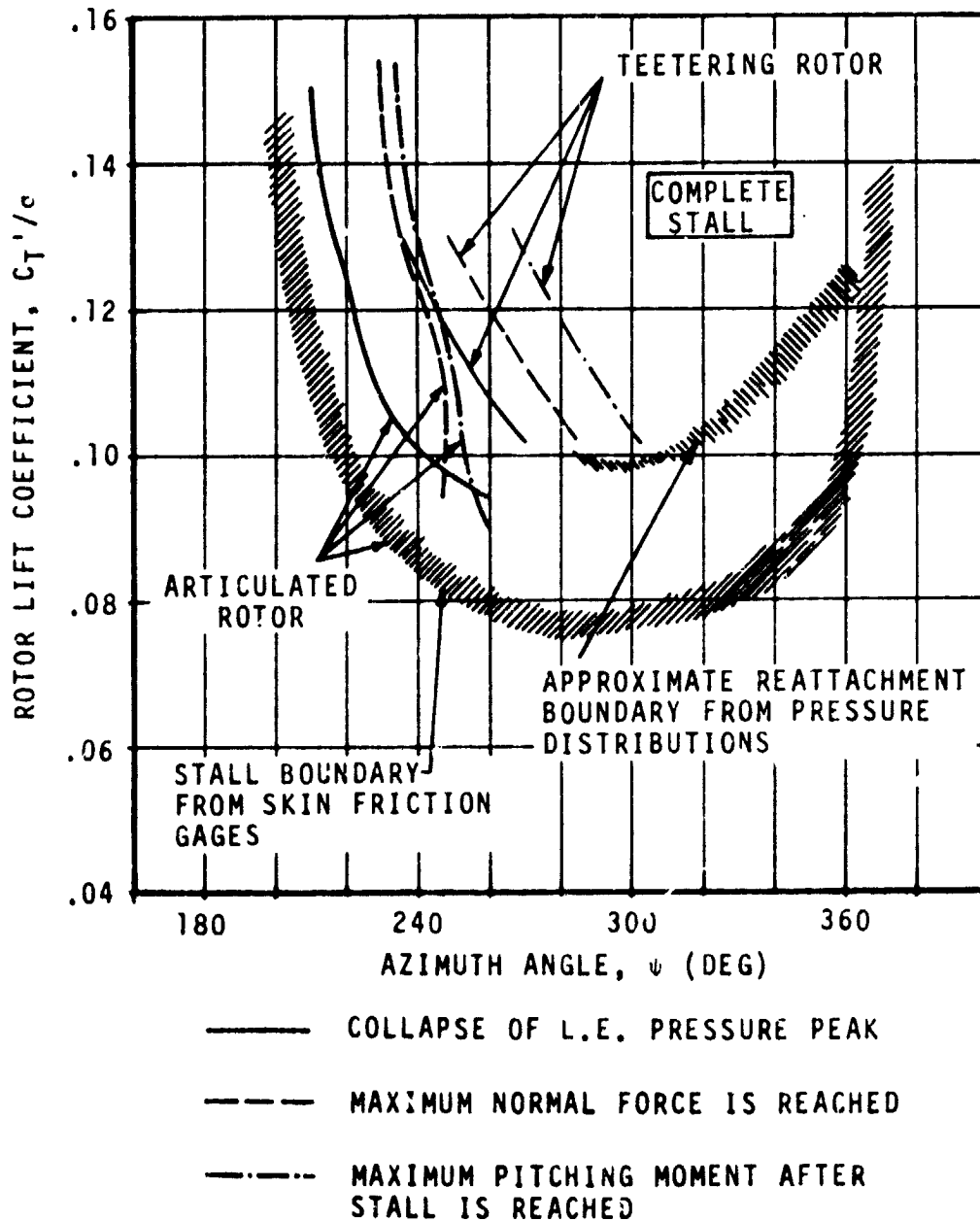
FIGURE 28 COMPARISON OF STALL BOUNDARIES OF TEETERING AND ARTICULATED ROTORS
