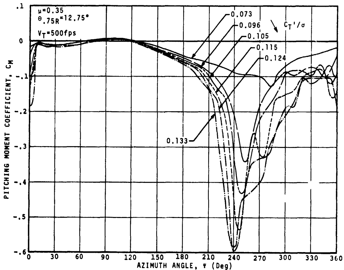
FIGURE 21 PITCHING MOMENT COEFFICIENTS OBTAINED FROM INTEGRATED PRESSURES AT r/R=0.75 . COMPARISON BETWEEN TEETERING AND ARTICULATED ROTORS
