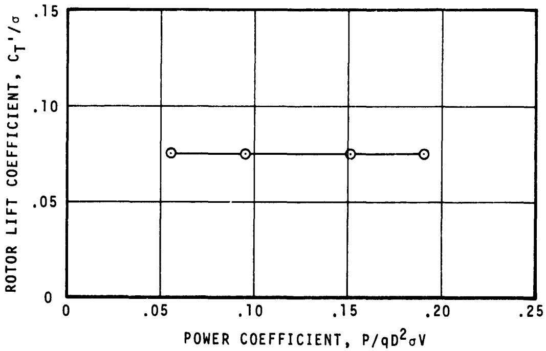
FIGURE 30 MODEL ROTOR PERFORMANCE DATA IN FORWARD FLIGHT. VARIATION IN PROPULSIVE FORCE AT CONSTANT LIFT.
