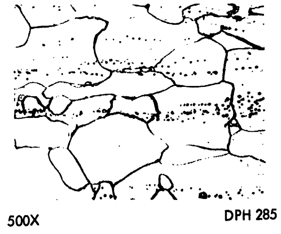
D. Swaged + 1 Hr/1371°C (2500°F)
