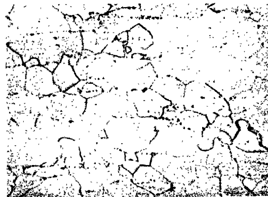
B. Swaged + 1 Hr/1482°C (2700°F)-DPH 341
