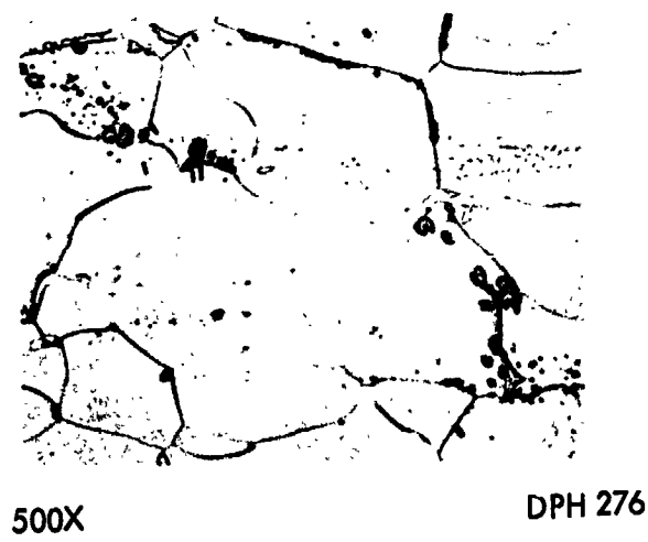
C. Swaged + 1 Hr/1260°C (2300°F)
