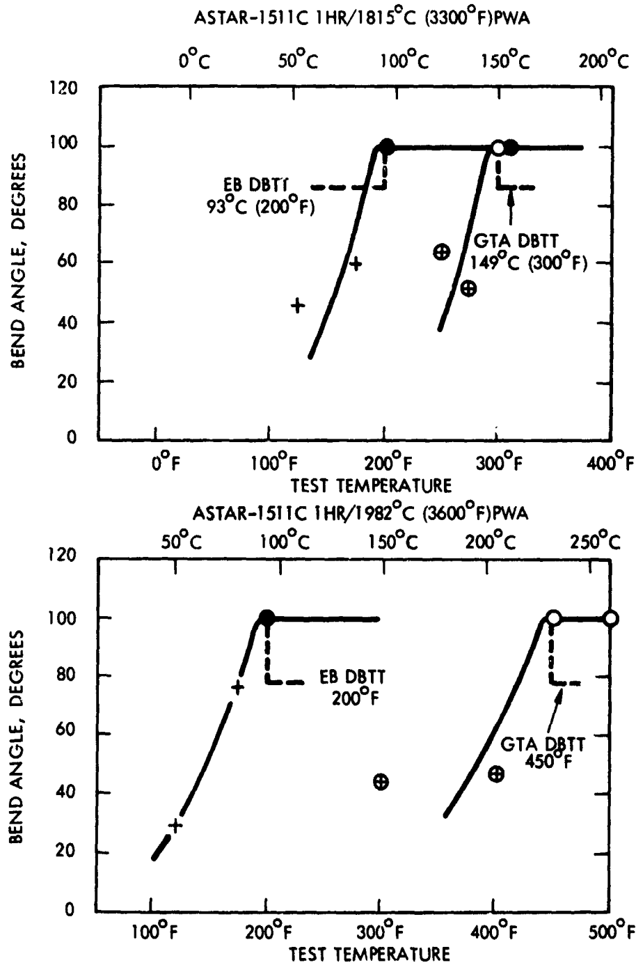
Figure 95. Results of 1t Bend Tests on EB and GTA Welds on 1.0 mm (0.040 inch) ASTAR-1511C Sheet. Thermal History as Indicated.
