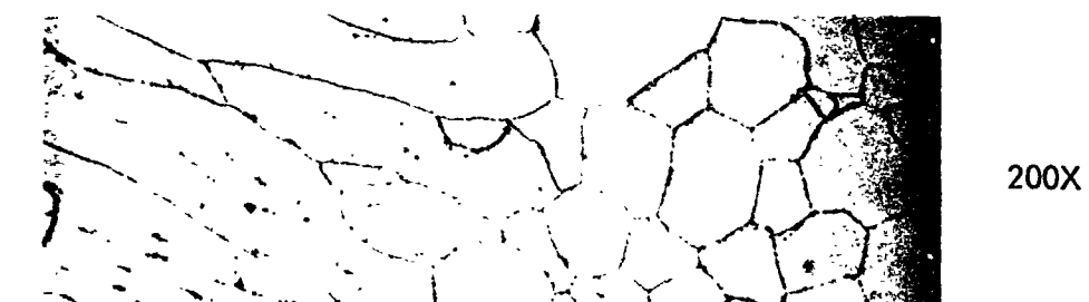
Weld Metal PWA-1 hr/1815°C (3300°F) Base Metal
