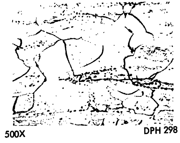
B. Swaged + 1 Hr/1093°C (2000°F)
