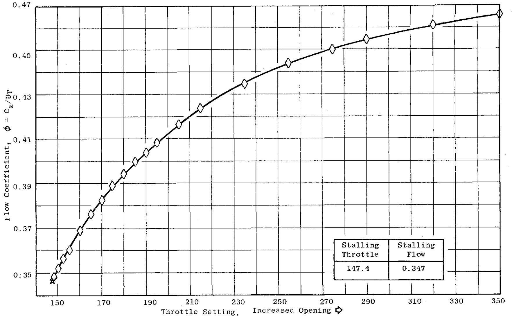
Figure 12. Flow Coefficient Versus Throttle Setting, Smooth Spool (Baseline) Configuration No. 1.
