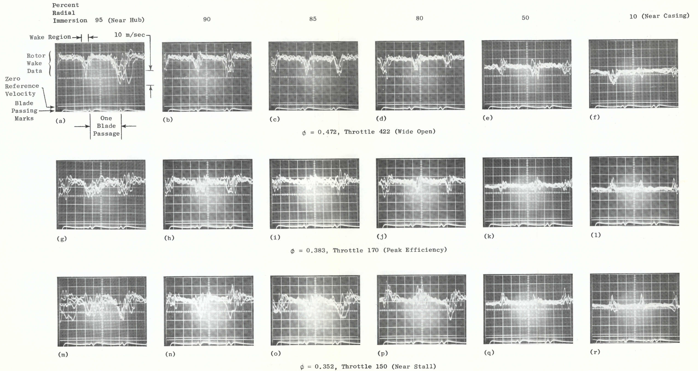
Figure 24. Typical Oscillograms Showing the Output of a Single Parallel Element Hot Film Anemometer Located at Rotor One Exit Plane, Smooth Spool Baseline Configuration No. 1, U_t = 45.7 m/sec (150 ft/sec).
