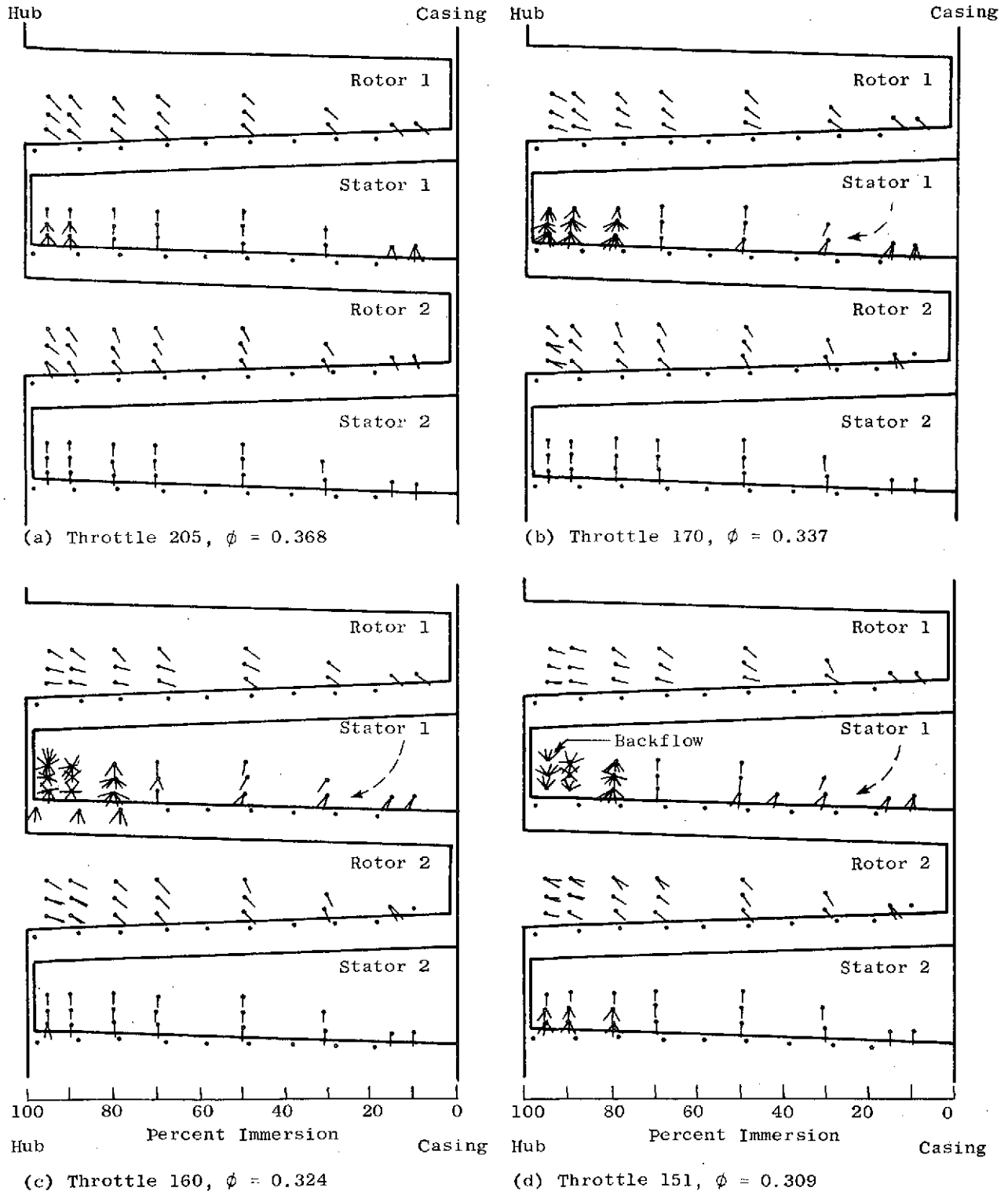
Figure 35. Schematic Representation of the Tuft Probing Measurements, Baseline Configuration No. 2, Restagger 0^\circ , +8^\circ , -4^\circ , +8^\circ , U_t = 45.7 m/sec (150 ft/sec).
