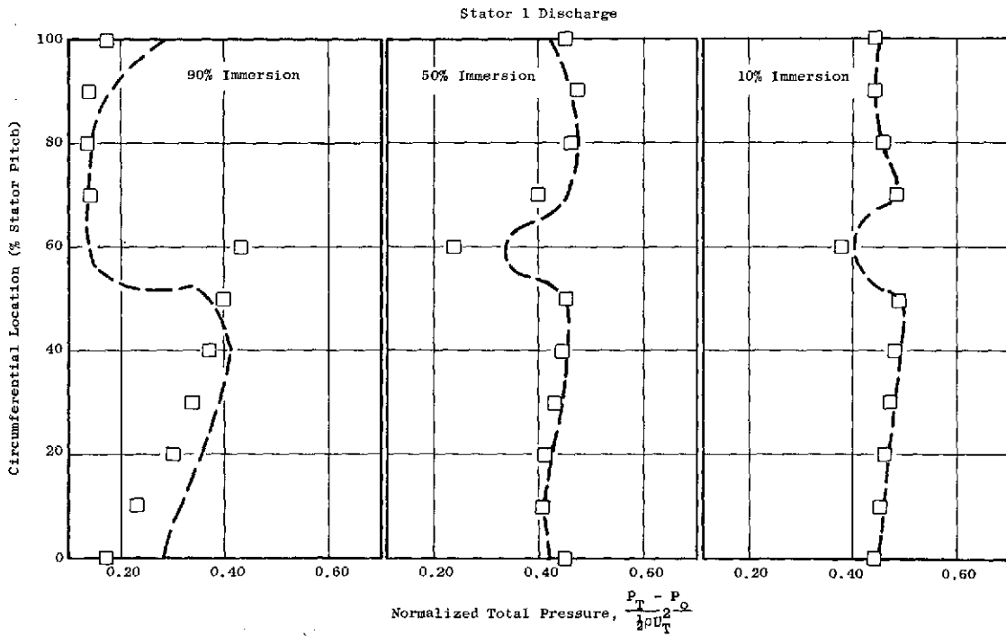
Figure 46. Comparison of the Circumferential Variation of Normalized Total Pressure for the Smooth Spool Baseline and Baffled Wide Blade Angle Slot Treatment Configurations No. 3, U_t = 45.7 m/sec (150 ft/sec).
