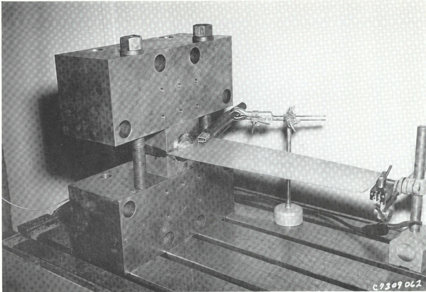
Figure 4. Bench Test Setup to Evaluate Stator Vane Critical Frequencies.
