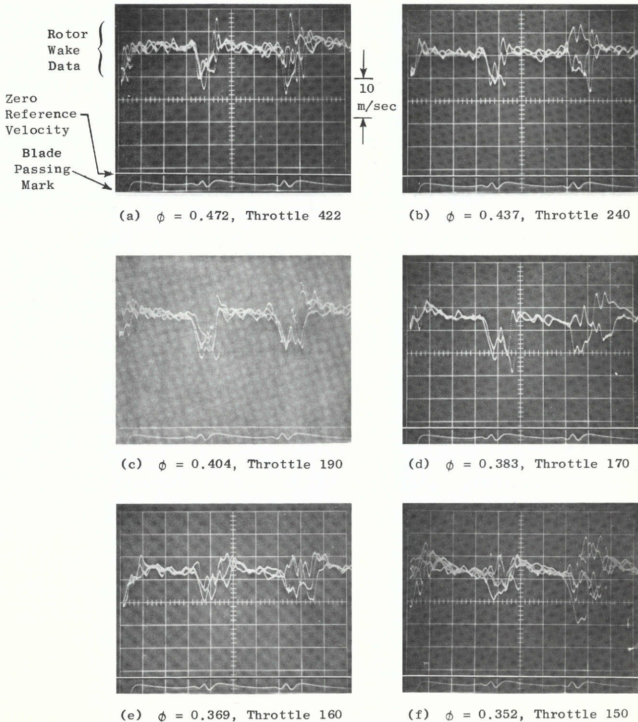
Figure 26. Typical Oscillograms Showing the Output of a Single Parallel Element Hot Film Anemometer Located at Rotor One Exit Plane, 90% Radial Immersion, Smooth Spool Baseline Configuration No. 1, U_t = 45.7 m/sec (150 ft/sec).
