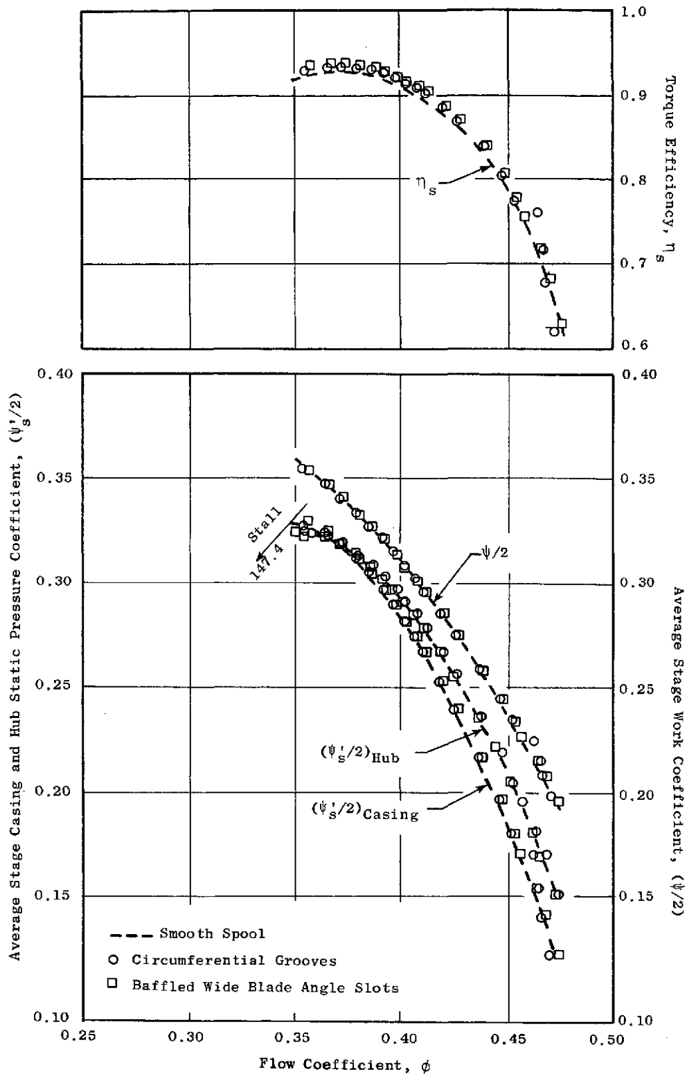
Figure 15. Overall Performance Comparison of Smooth Spool, Circumferential Groove and Baffled Wide Blade Angle Slot Treatment Configuration No. 1, Based on Preview Data, U_t = 45.7 m/sec (150 ft/sec).
