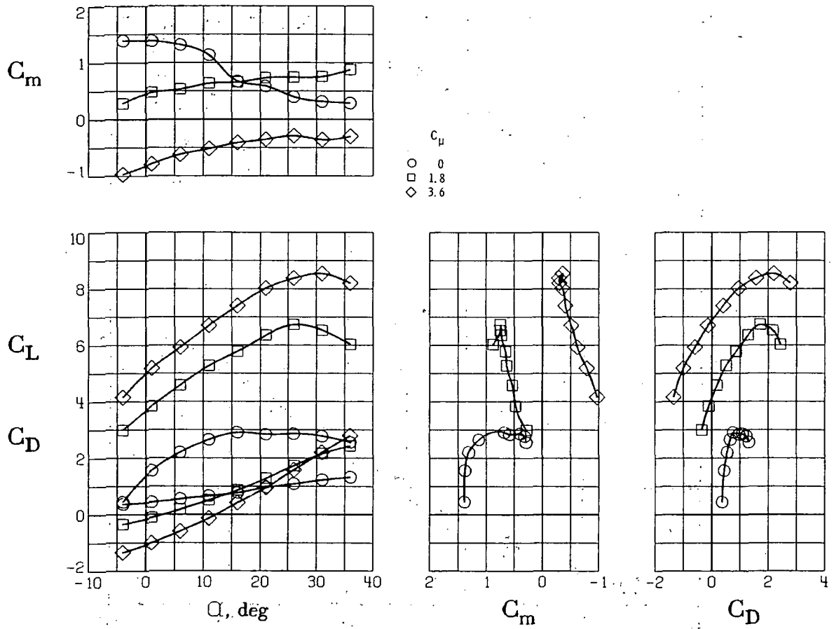
Figure 12.- Longitudinal aerodynamic characteristics of the model with T-tail.
