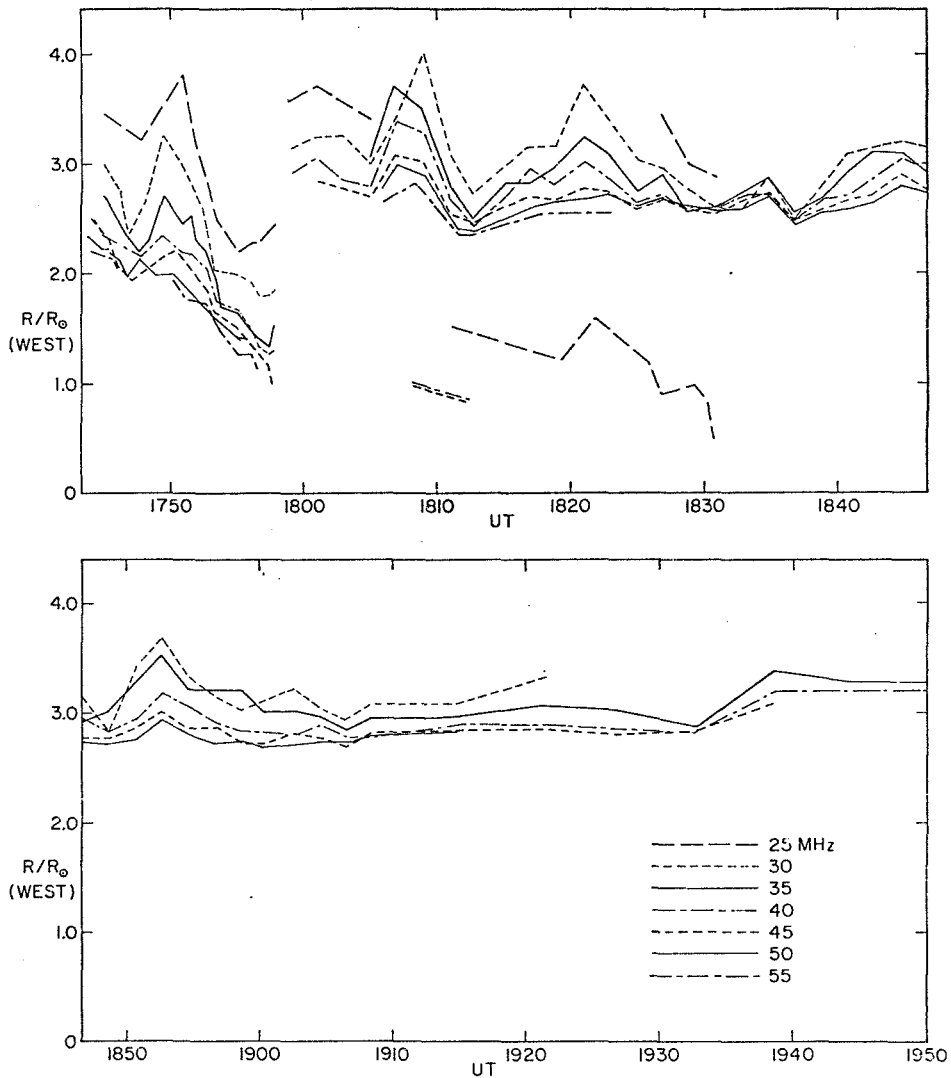
Fig. 3c. Positions of the composite type II-type IV event as a function of frequency and time.
