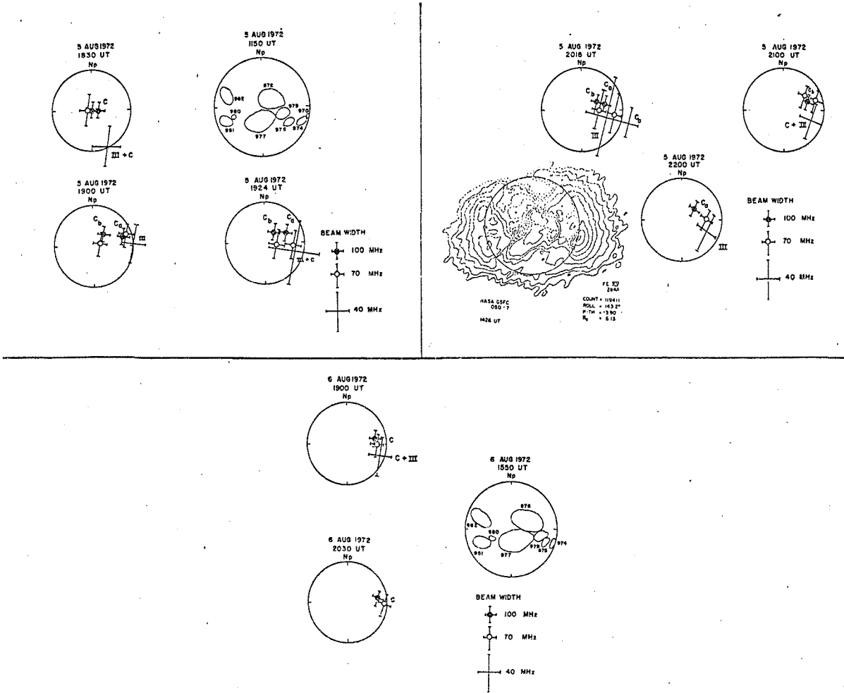
Fig. 4. Positions of bursts for August 5 and 6, together with the McMath-Hulbert Calcium reports. Also included is the Fe xv line ( 284 \text{ \AA} ) map for August 5, obtained by NASA-GSFC OSO-7. The radio positions are indicated in the same way as in Figure 2.
