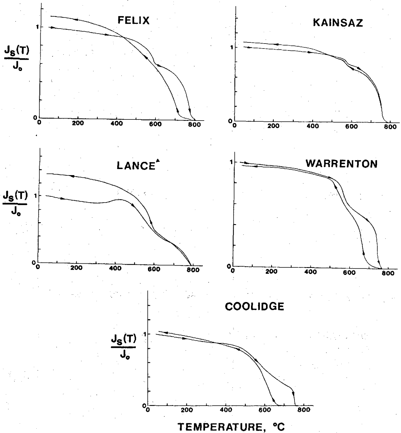
Fig. 3. Saturation magnetization vs. temperature ( J_S - T ) curves for four C3 chondrites and the remaining C4 chondrite. Felix and Lance 1 show evidence for slight magnetite production. No magnetite production was seen in the Kainsaz and Warrenton C3 chondrites or in the Coolidge C4 chondrite.
