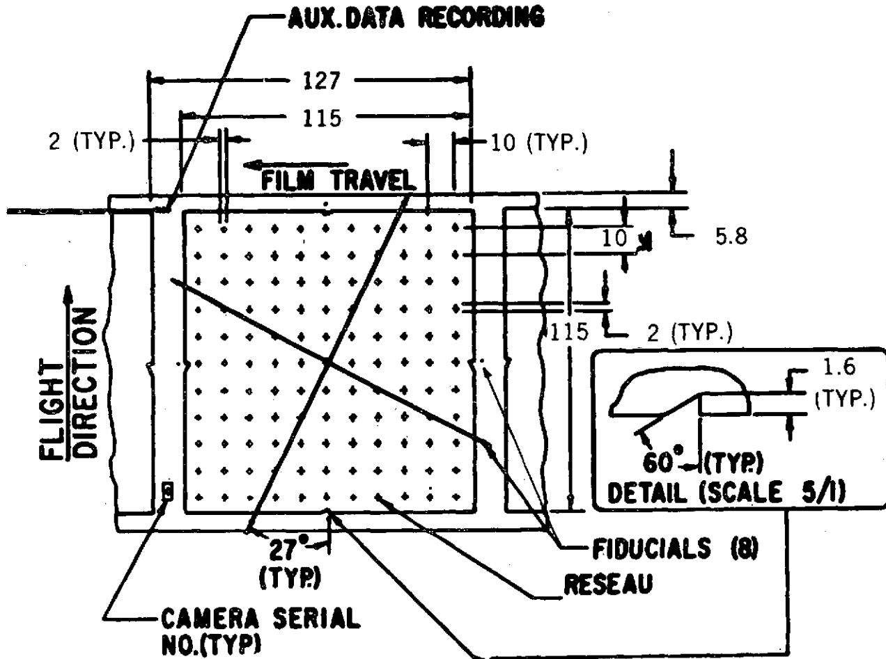
Figure 2. Mapping Camera Film Format (in millimeters)
