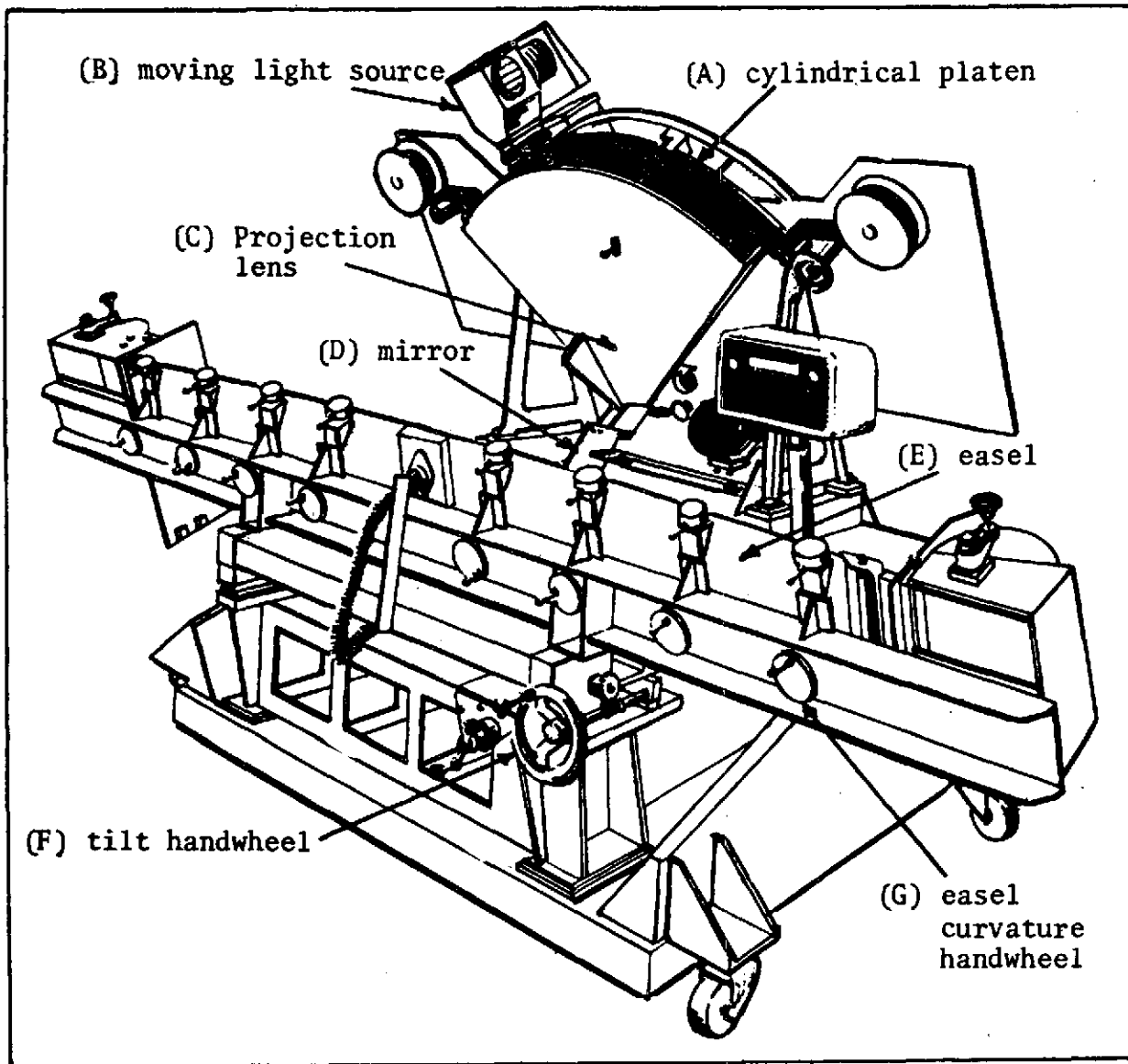
Figure 13. Transforming Printer for Apollo Panoramic Camera Photography
