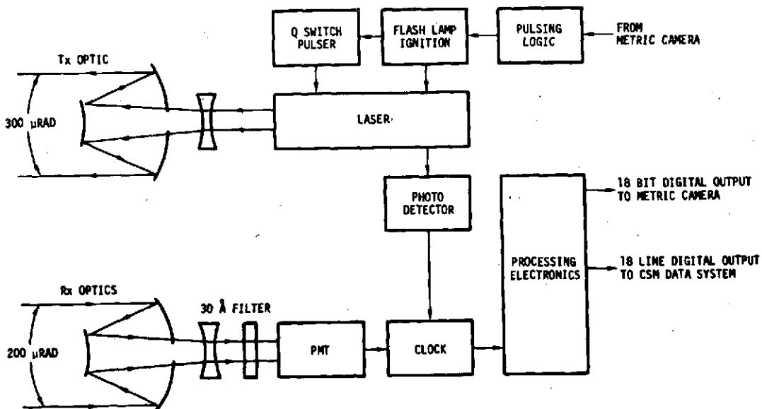
Figure 4. Laser Altimeter Block Diagram
