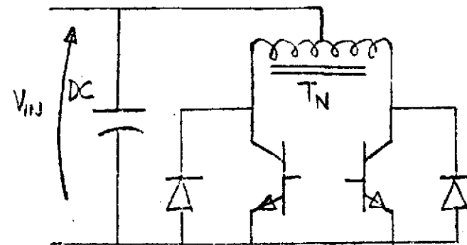
MULTICYLINDER INVERTER
