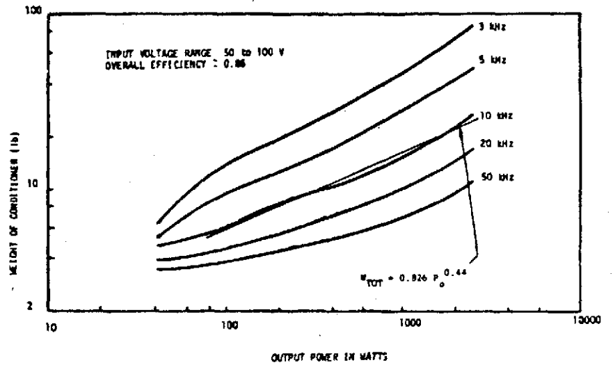
Conditioner weight as a function of output power.
