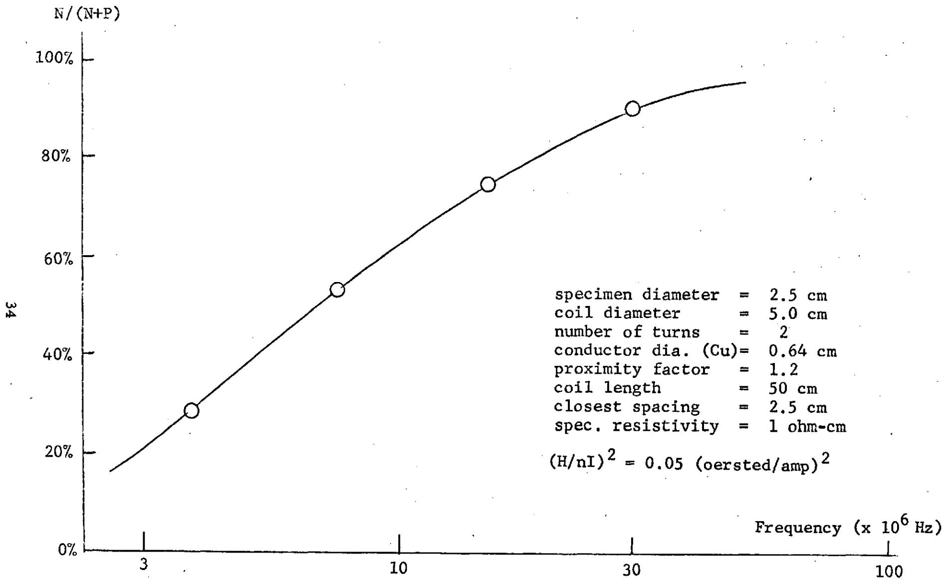
Figure 4-2. Efficiency of Heating a ZrO_2 Specimen at 2000^\circ in a Baseball Coil
