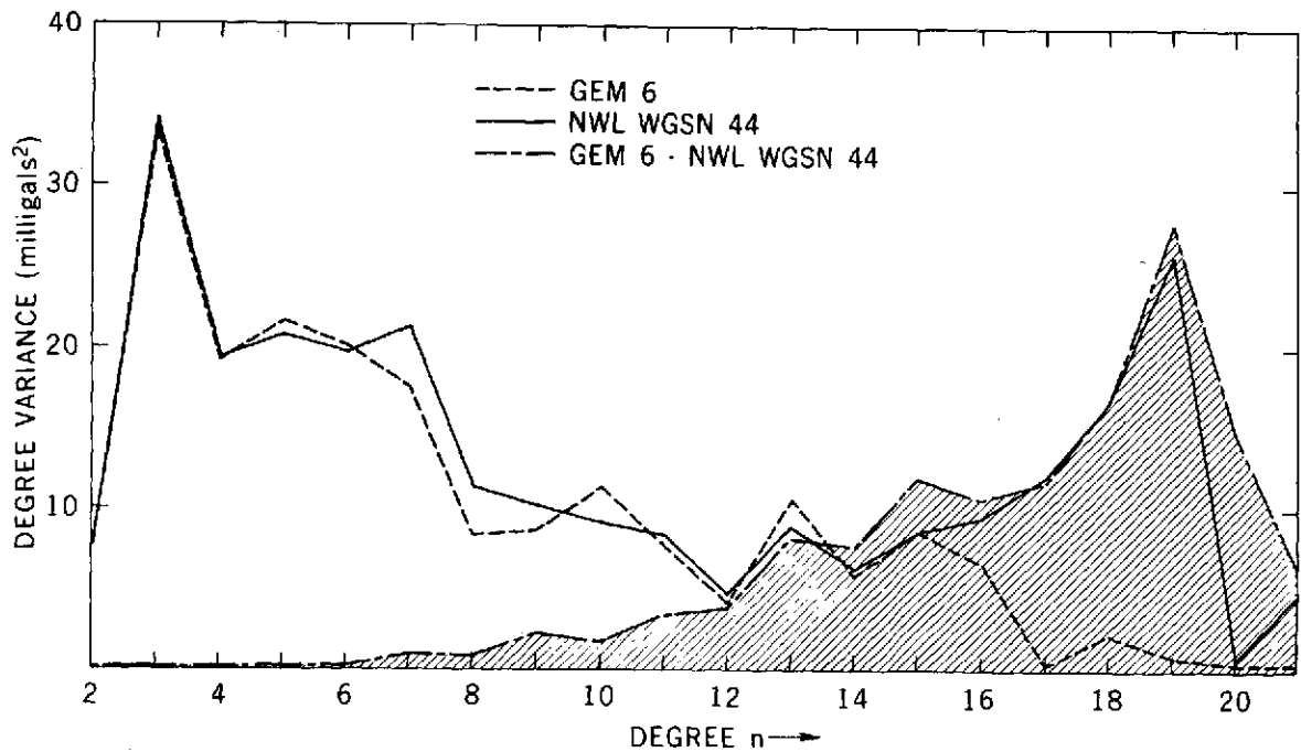
Figure 8. Degree Variances: GEM 6 and WGSN 44
