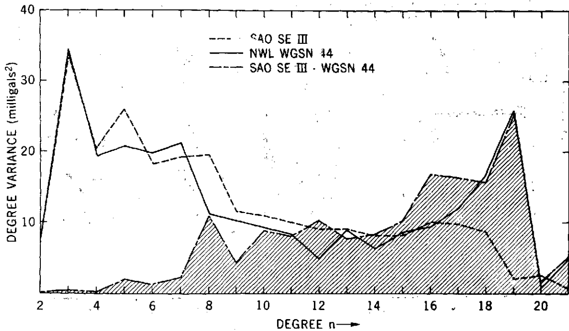
Figure 6. Degree Variances: SE III and NWL WGSN 44
