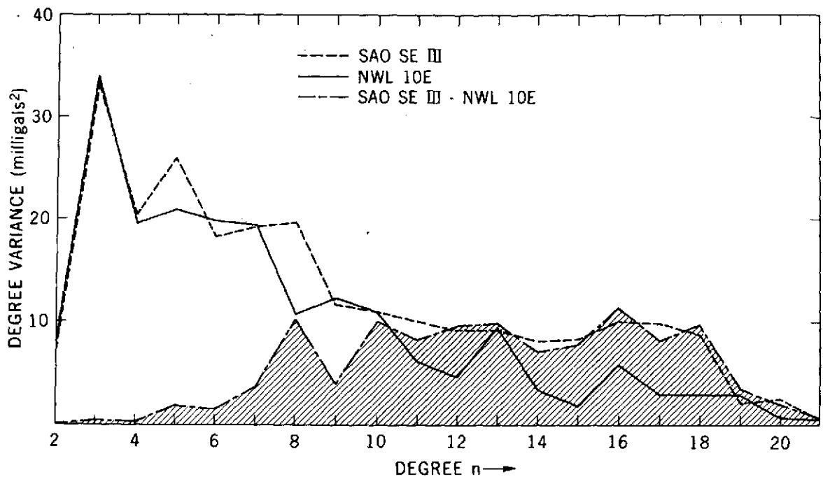
Figure 7. Degree Variances: SE III and NWL 10E
