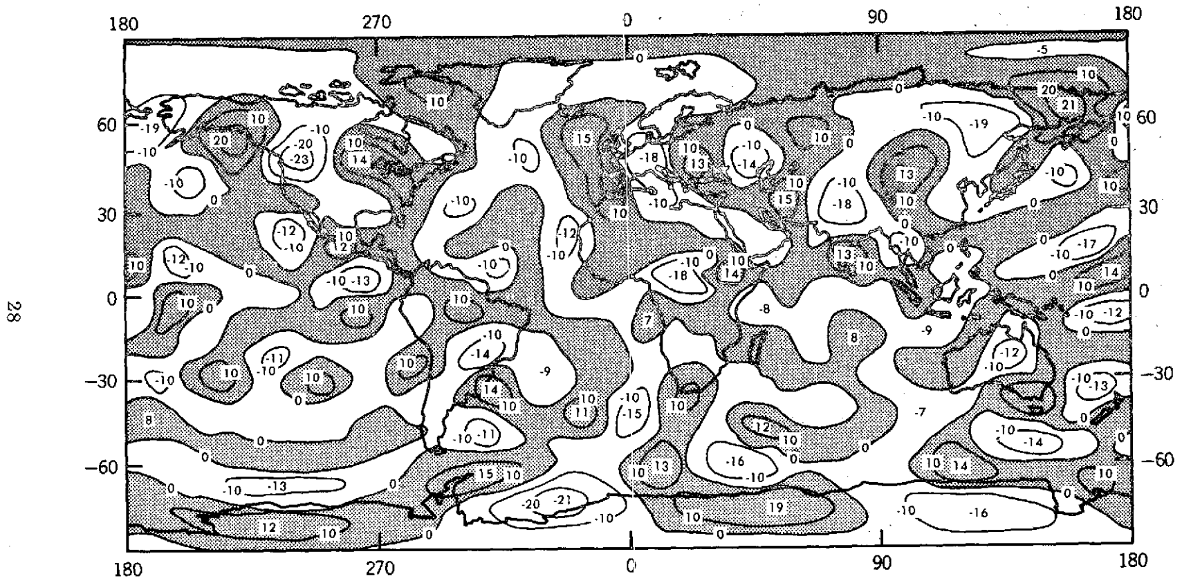
Figure 16. Free Air Gravity Anomalies based on differences between GEM 6 and GEM 5
