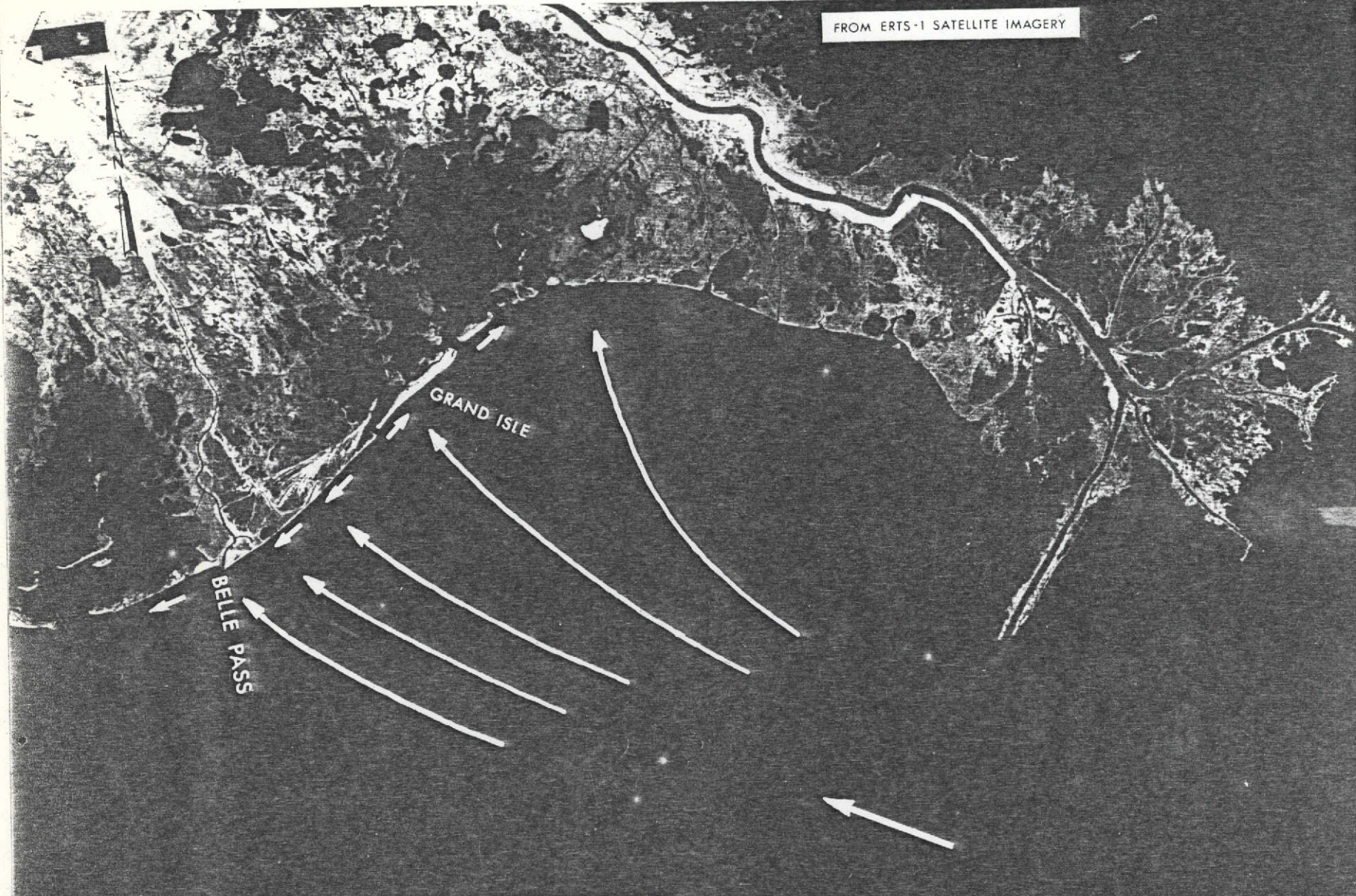
WAVE AND LITTORAL CURRENT DIRECTIONS EAST-SOUTHEASTERLY WINDS BELLE PASS AREA, LOUISIANA
