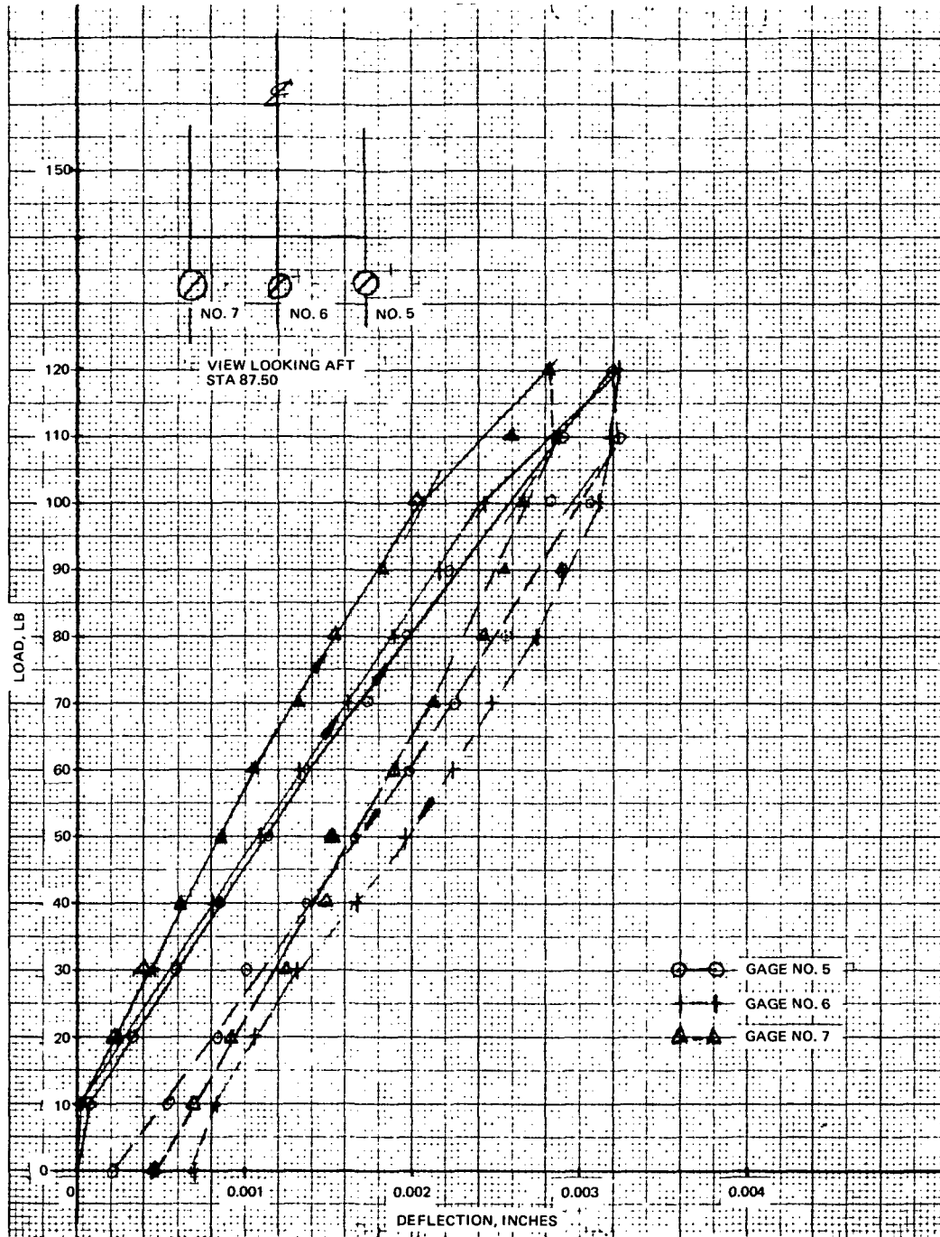
Fig. A3-12 Static Deflections (Run No. 5): +Z Load at Sta 116.0 (No Doors)
