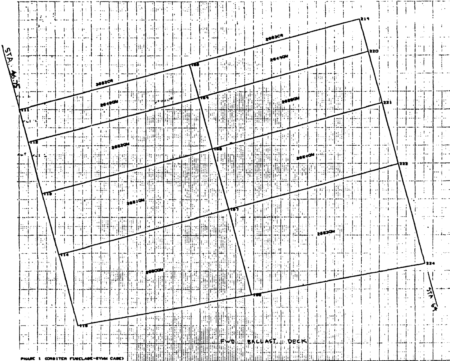
PHASE 1 CORBITER FUSELAGE-SYMM CASE) REVISION 4/22/74 (HALF EFFECTIVE SKINS) UNDEFORMED SHAPE
