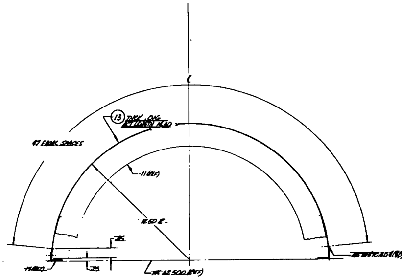
VIEW J - J (TOP A. PLACES) SCALE 1:1
