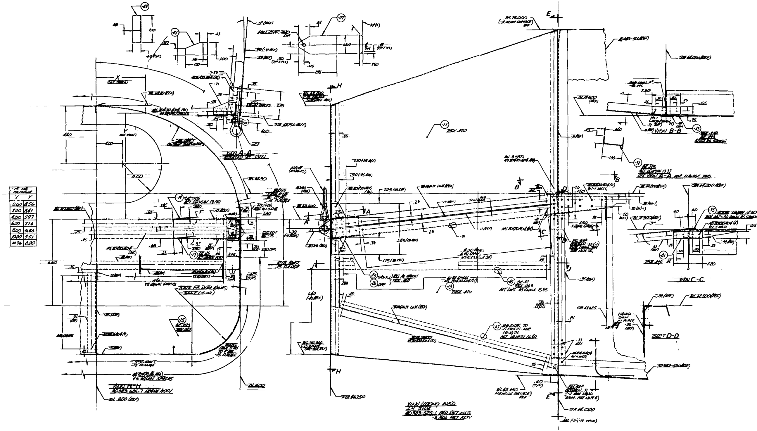
Orbiter Forward Section Ass'y and Installation (Sta 46.750 to 64.000) (Sheet 2 of 3)
