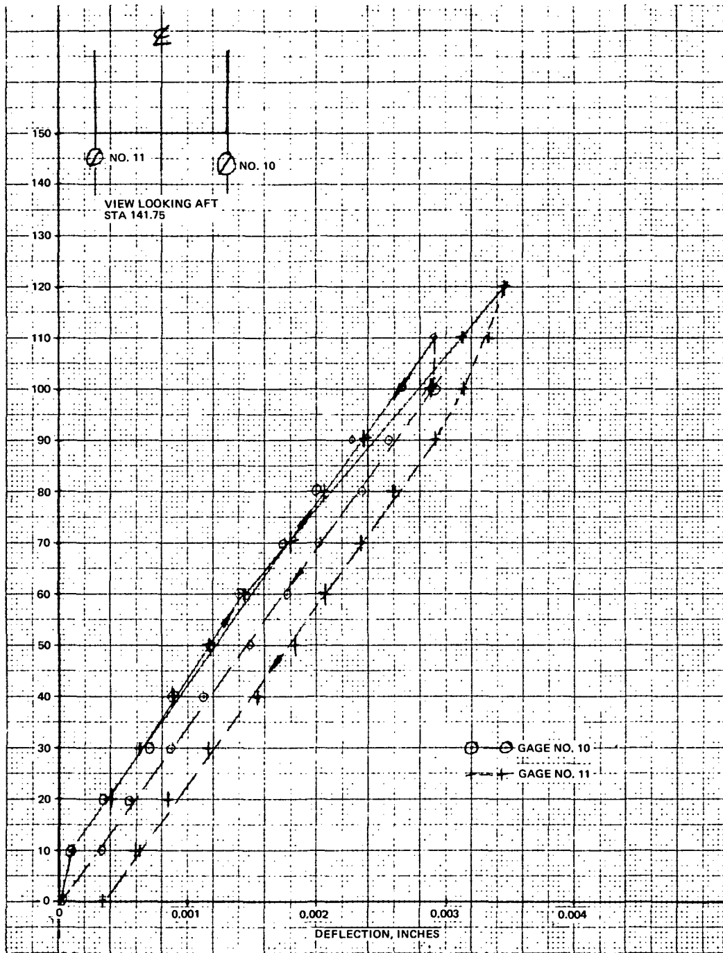
Fig. A3-14 Static Deflections (Run No. 5): Load +Z at Sta 116 (No Doors)
