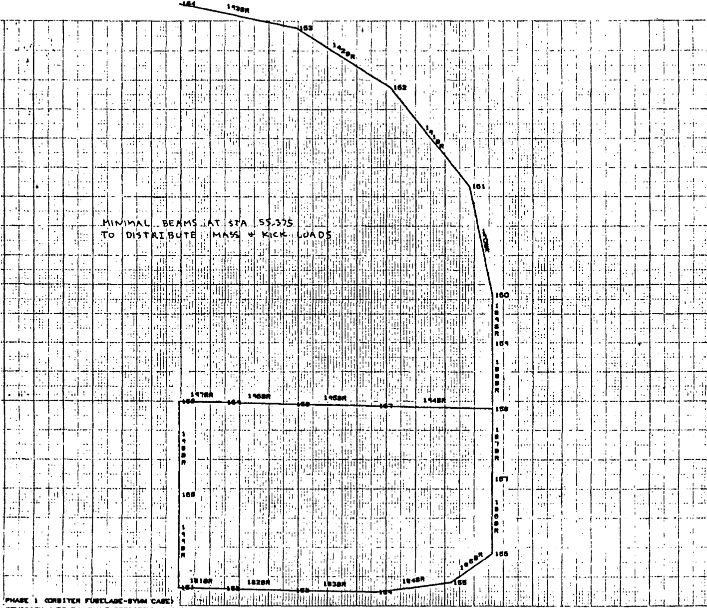
PHASE 1 ORBITER FUELADE-SYMM CASE) REVISION 4/22/74 (HALF EFFECTIVE SKINS)
