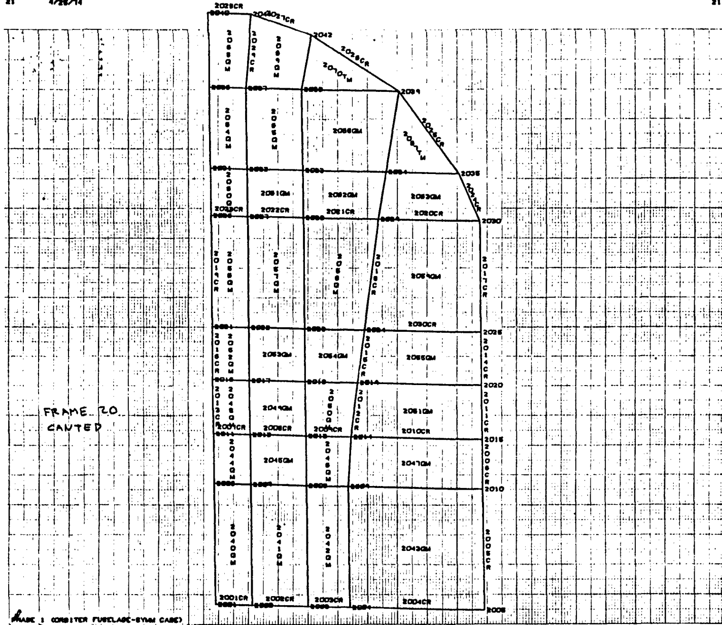
FIGURE 1 (CORBITER FUSELAGE-SYMM CASE) REVISION 4/22/74 (HALF EFFECTIVE SKINS)
