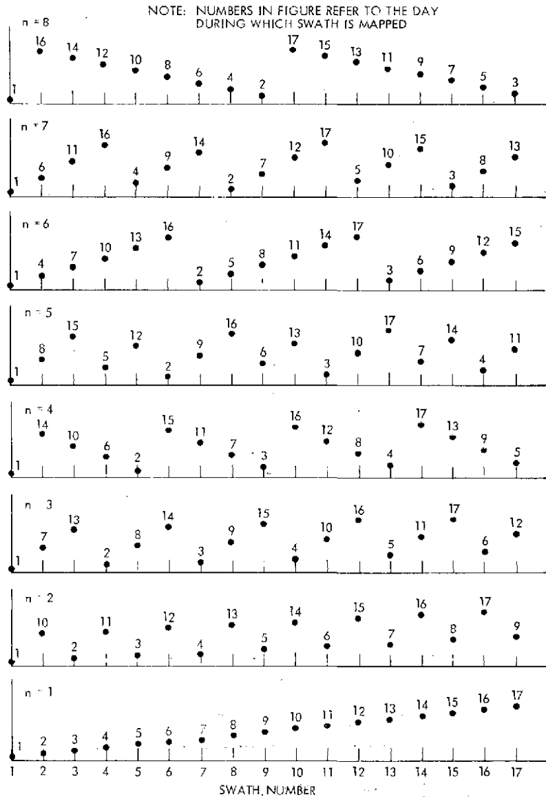
Figure 3-6. Swathing Patterns for 17-Day Cycle ( n > 8 )
