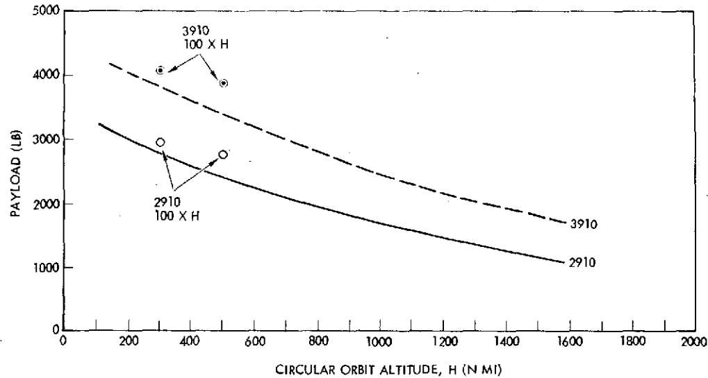
Figure 3-15. Thor-Delta Sun-Synchronous Orbit Capability from WTR
