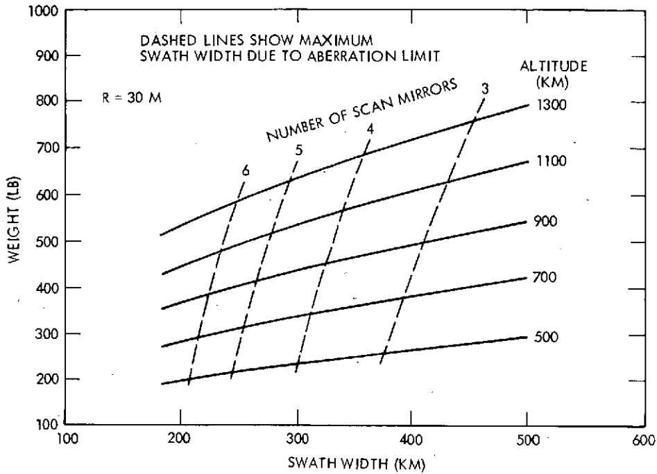
Figure 4-4. Weight of Honeywell Scammer
