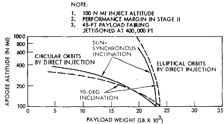
Figure 3-17. Titan IIID Payload Weight Versus Altitude (WTR)
