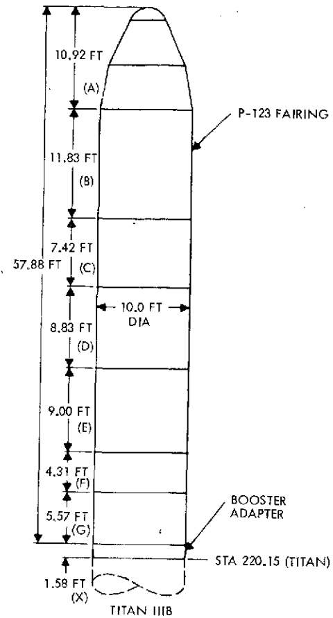
Figure 3-20. Payload Fairing and Agena Shroud for Titan IIIB (SSB)/ Ascent Agena (ETR and WTR)
