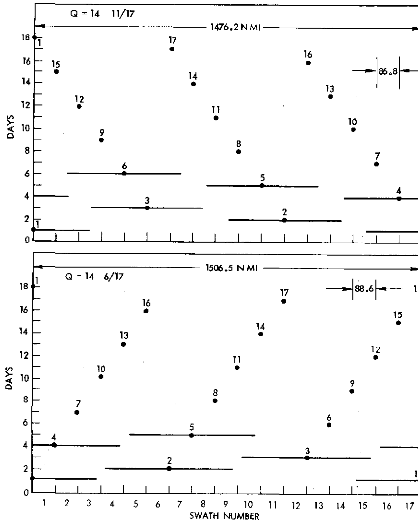
Figure 3-7. HRPI Offset Considerations
