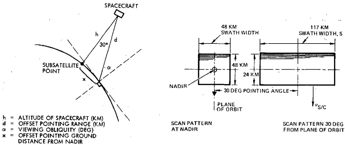
Figure 4-7. HRPI Scan Pattern at Nadir and 30-Degree Offset Pointing (See Table 4-13 for s as a Function of Altitude)
