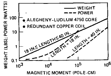
Figure 5-6. Magnetic Torquer Sizing
