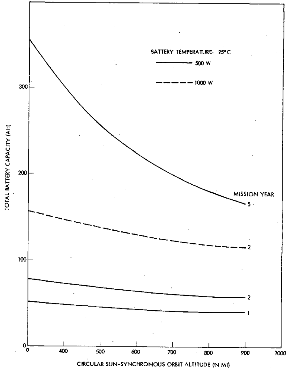
Figure 5-2. Average Occult Discharge Power
