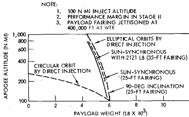
Figure 3-16. Titan IIIB (SSB), Payload Weight Versus Altitude (WTR)
