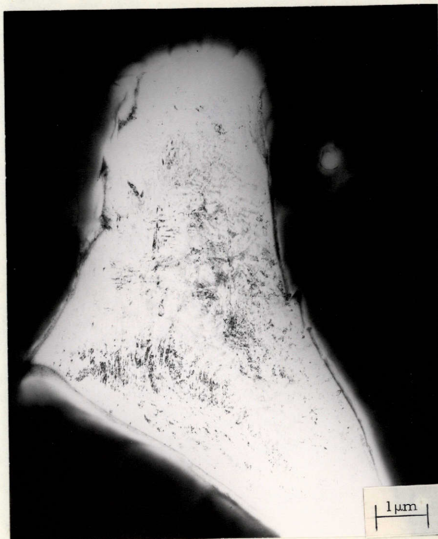
Figure 3. Transmission electron micrograph showing the complex structure of the dispersed phase in the air-cooled, normal interstitial Ti-5Al-2.5Sn alloy.
