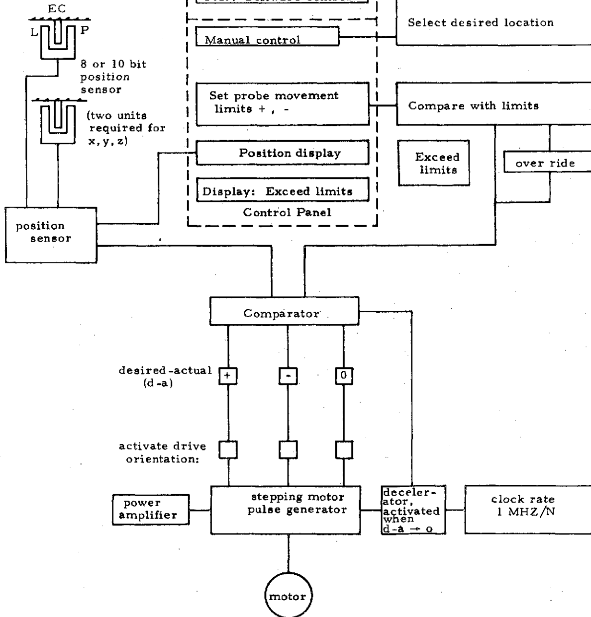
Figure 3. Schematic of position control sub-system; Note: One sub-system for each position: x, y, z, \theta ; N will be selected to obtain the maximum stepping rate per the torque requirements of the individual position control circuit
