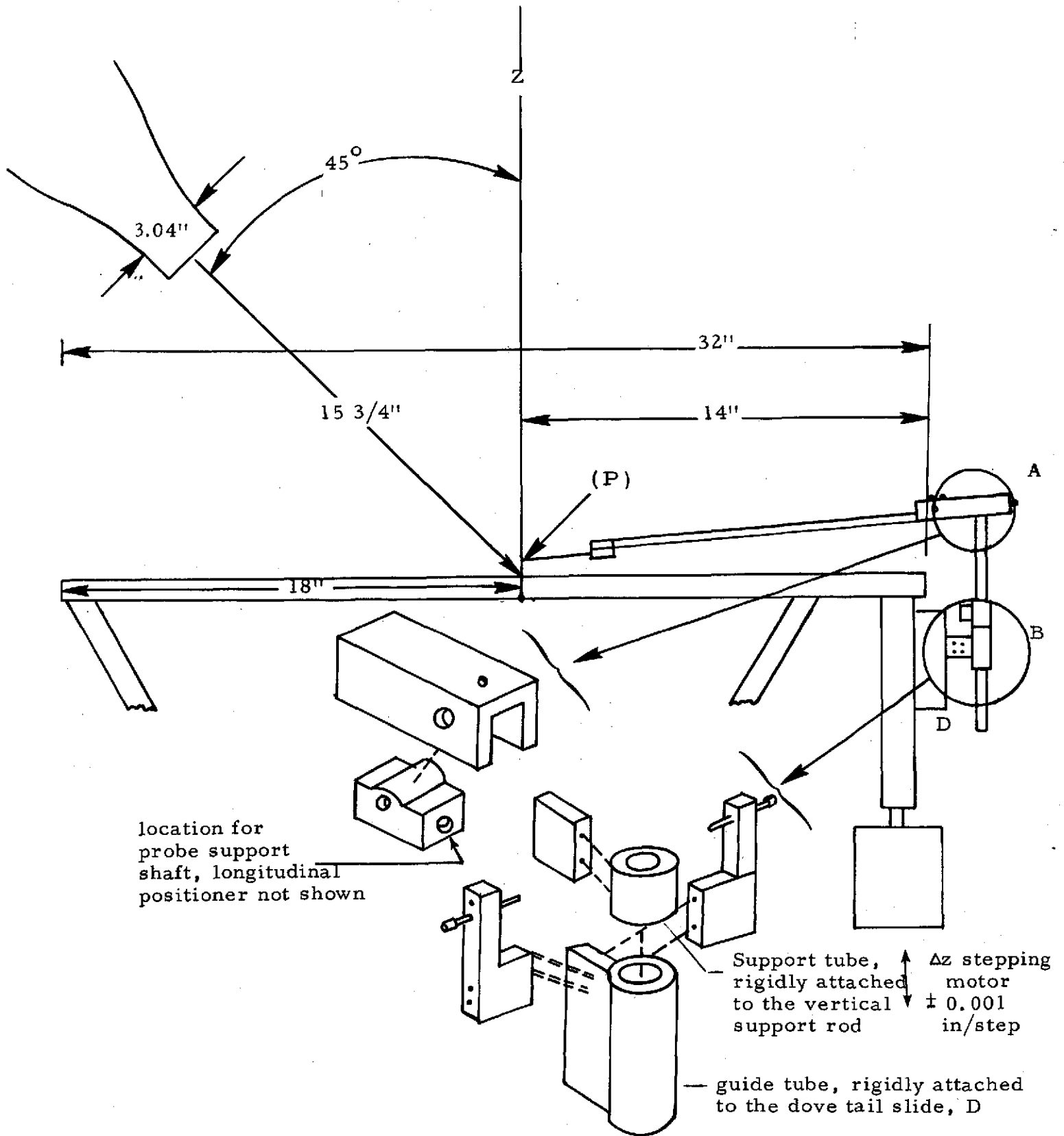
Figure 2b. Upper plate and jet. Detail A shows the mechanism to allow longitudinal and pitch angle positioning of the probe (P). Detail B shows the yaw angle positioner. These three adjustments are sufficient to locate the probe tip over the rotation axis of the plate.
