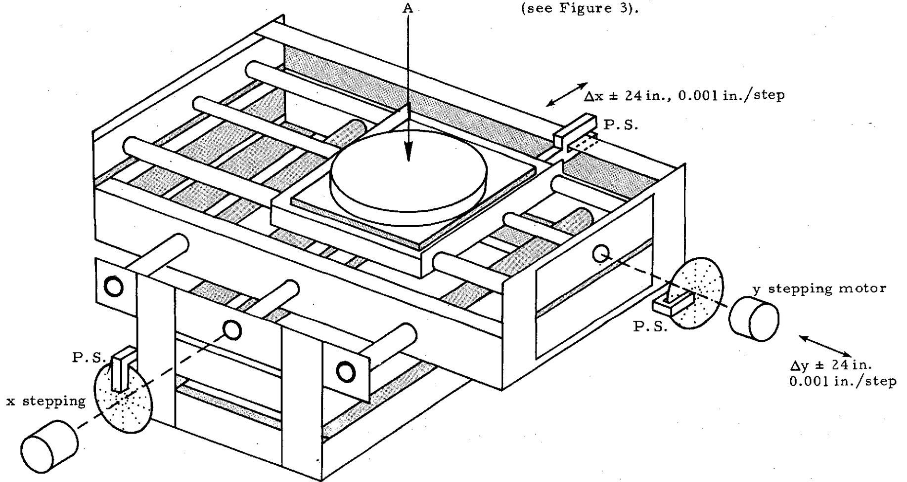
Figure 2a. The x, y, \theta traverse device.
